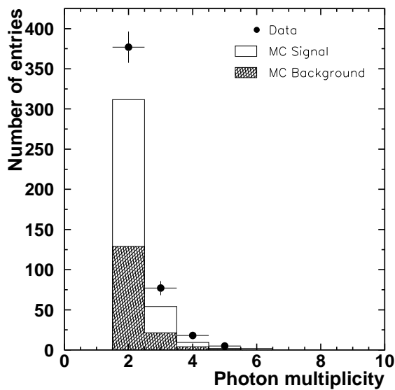
FIG. 6. Photon multiplicity of \text{CC}\pi^0 candidate events
