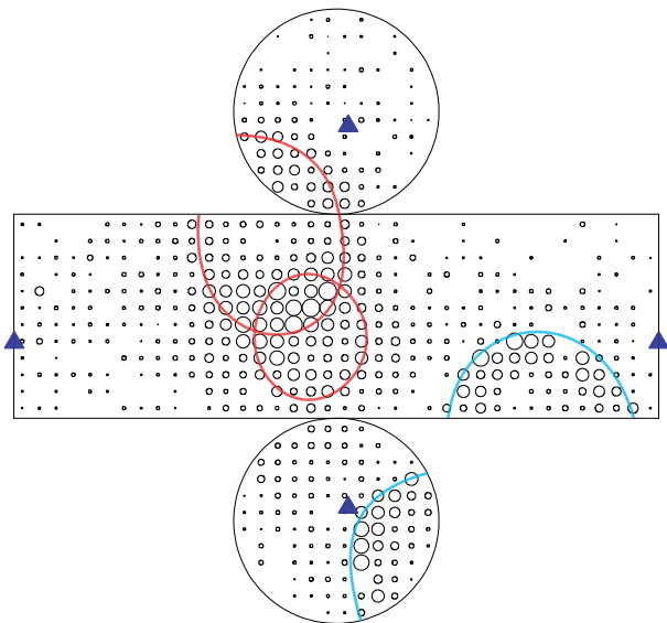
FIG. 6: Event display of “ p \rightarrow \mu\pi^0 ” sample in the KT real data satisfying selection criteria (A)–(E). Each hit PMT is represented by a small circle whose area is proportional to the PMT’s measured charge. The small blue triangles show the projection of the reconstructed vertex onto the walls. Cyan (red) thick circles show reconstructed rings identified by the PID as muon (electron)-like (Two overlapped thick circles are identified as electron-like rings). The reconstructed M_{\pi^0}, M_{tot} , and P_{tot} for this event are 164 \text{ MeV}/c^2, 851 \text{ MeV}/c^2, and 226 \text{ MeV}/c , respectively.
