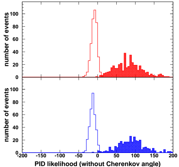
FIG. 3: PID likelihood for cosmic ray muons (shaded histogram) and the decay electrons (open histogram). The red (blue) histogram (top (bottom) figure) shows data (MC). Positive (negative) likelihood corresponds to muon (electron)-like.
