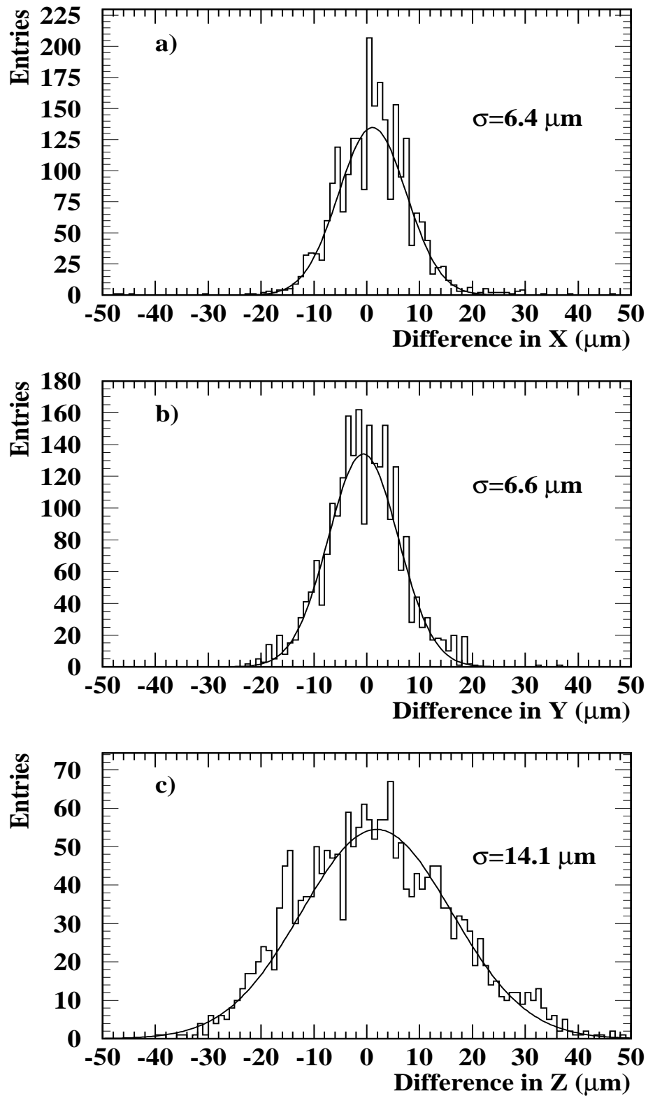
Figure 15: Resolution of the surveying system. Systematic differences in the measurements of the coordinates a) X, b) Y and c) Z.
