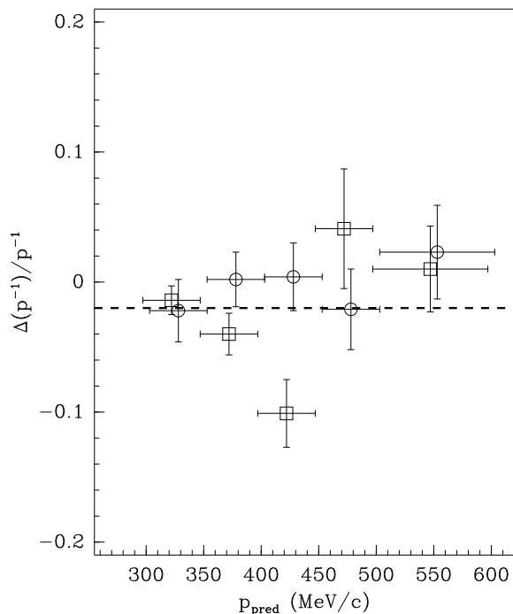
Figure 5. The momentum bias of the fit without vertex constraint measured with elastic scattering data (3 GeV/ c : open squares, 5 GeV/ c : open circles) as a function of the momentum predicted by the forward scattered track. In the absence of a clear trend, the average of the points constrains the bias to be smaller than 3%. For these comparisons only the first 50 events in the spill are used since the unconstrained fit is sensitive to dynamic distortions beyond this value.
