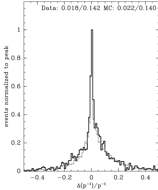
Figure 4. Comparison of the unconstrained ( p_1 ) and constrained ( p_2 ) momentum ( p_1/p_2 - 1 ) for pions (above 350 MeV/ c ) using data (from different target materials) and the corresponding Monte Carlo. The data are indicated by the black histogram and the Monte Carlo by the dashed histogram. The position of the peak is at zero well within 1% and the mean is 2% both for data and MC. The first 50 events in the spill are used.
