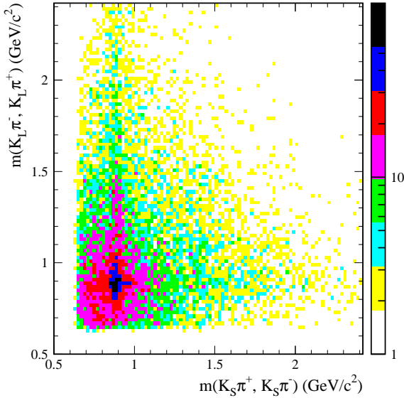
FIG. 21: The K_L^0 \pi^+ invariant mass versus the K_S^0 \pi^- invariant mass (two entries per event).
