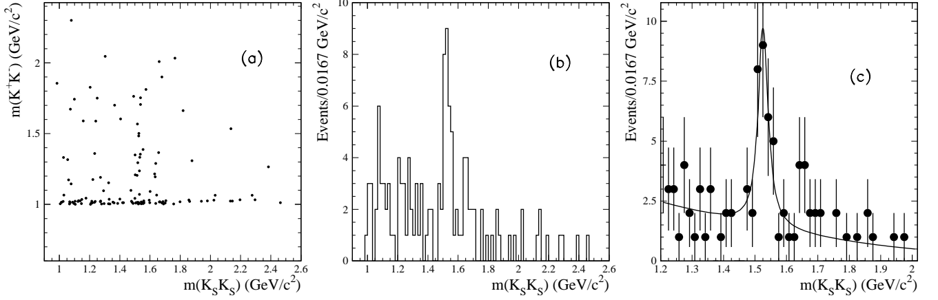
FIG. 38: (a) The K^+K^- versus K_S^0K_S^0 invariant mass for all selected K_S^0K_S^0K^+K^- events in the data. (b) The m(K_S^0K_S^0) projection of (a). (c) An expanded view of (b) in which the line represents the result of the fit described in the text.
