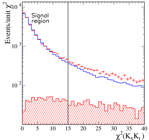
FIG. 6: The three-constraint \chi^2 distribution for K_S^0 -cluster- \gamma events in the data (points) fitted under the K_S^0 K_L^0 \gamma hypothesis. The open histogram represents the same distribution for the MC-simulated signal events, normalized to the data in the region \chi^2 < 10 , and the shaded histogram represents the estimated background in the data.
