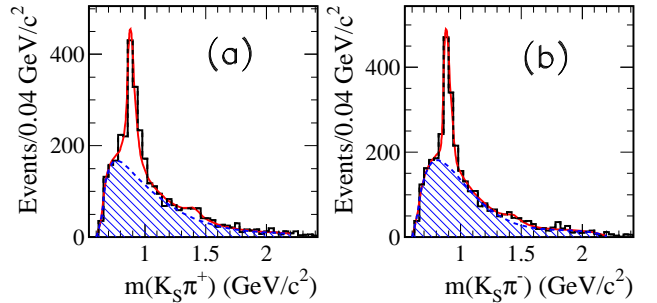
FIG. 31: The (a) m(K_S^0 \pi^+) and (b) m(K_S^0 \pi^-) projections of Fig. 30. The lines and hatched areas represent the results of the fits described in the text and their non- K^* components, respectively.
