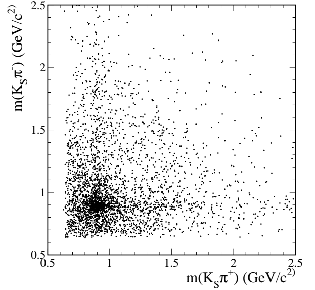
FIG. 30: The K_S^0 \pi^- invariant mass versus the K_S^0 \pi^+ invariant mass (two entries per event).
