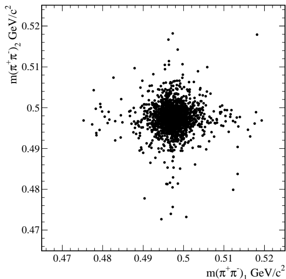
FIG. 26: Scatter plot of the \pi^+ \pi^- invariant mass of one K_s^0 candidate versus that of the other K_s^0 candidate calculated using the results of the constrained fit.
