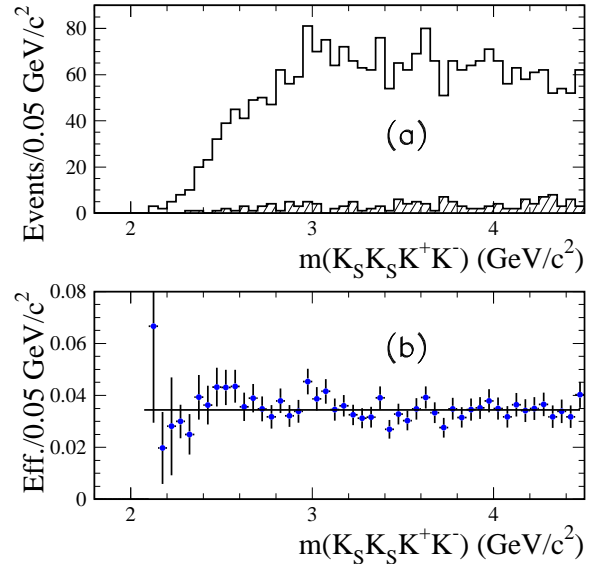
FIG. 36: (a) The K_s^0 K_s^0 K^+ K^- invariant mass distribution for the MC-simulated signal events in the signal and control (shaded) regions of Fig. 34. (b) The net reconstruction and selection efficiency from the simulation.
