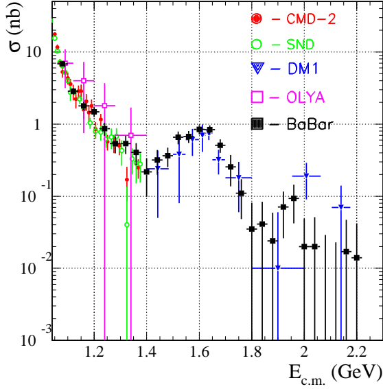
FIG. 15: The e^+e^- \rightarrow K_S^0 K_L^0 cross section compared with all available data in this E_{c.m.} region.
