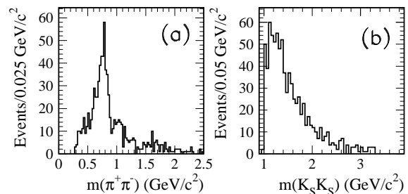
FIG. 33: The (a) \pi^+ \pi^- and (b) K_S^0 K_S^0 invariant mass distributions for the selected K_S^0 K_S^0 \pi^+ \pi^- events with K^*(892)^+ K^*(892)^- events excluded (see text).
