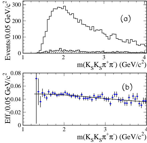
FIG. 28: (a) The K_S^0 K_S^0 \pi^+ \pi^- invariant mass distribution for the MC-simulated signal events in the signal and control (shaded) regions of Fig. 25. (b) The net reconstruction and selection efficiency from the simulation.
