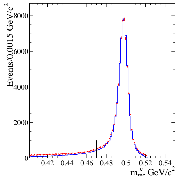
FIG. 2: The distribution of constrained recoil mass m_{\text{rec}}^c , obtained according to Eqs. 1 and 2, for selected \gamma K_s^0 candidates. The points represent the data, and the histogram an MC simulation of e^+e^- \rightarrow \gamma\phi \rightarrow \gamma K_s^0 K_L^0 events, normalized to the two most populated bins.
