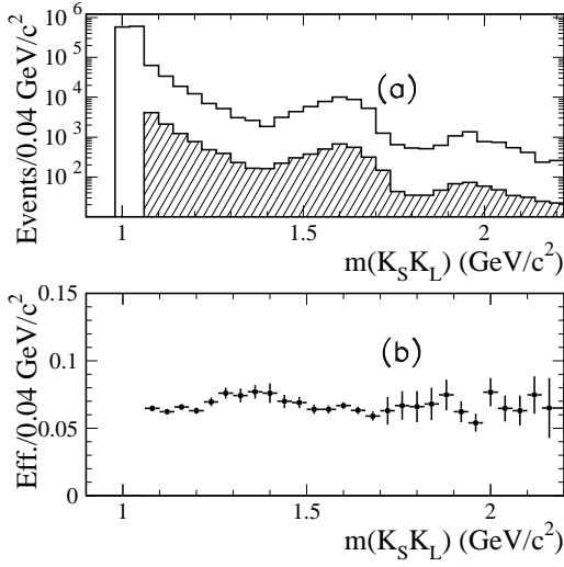
FIG. 14: a) The K_S^0 K_L^0 mass distributions from the MC simulation for the signal (unshaded) and control (shaded) regions of Fig. 12. b) The mass dependence of the simulated net reconstruction and selection efficiency for the K_S^0 K_L^0 final state in the m(K_S^0 K_L^0) > 1.06 \text{ GeV}/c^2 region.
