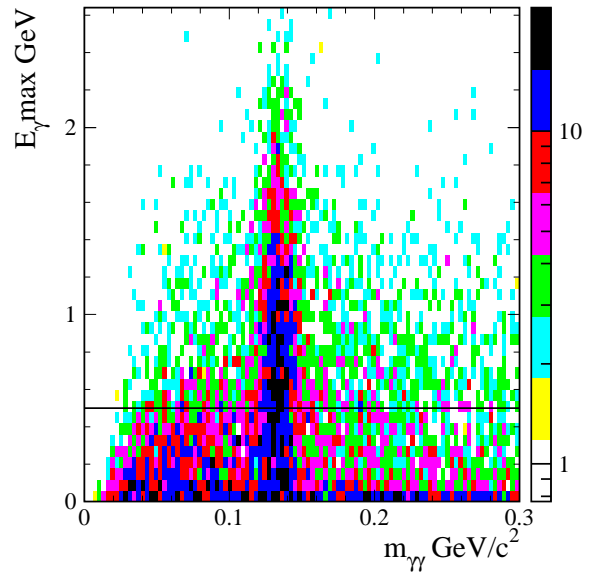
FIG. 11: Two-dimensional plot of the higher cluster energy in a photon-candidate pair versus the corresponding diphoton mass m_{\gamma\gamma} for all pairs of EMC clusters, containing neither the ISR photon nor the K_L^0 candidate.
