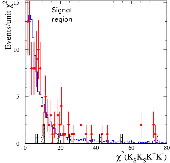
FIG. 34: The four-constraint \chi^2 distributions for K_s^0 K_s^0 K^+ K^- \gamma candidate events in the data (points) and signal MC simulation (open histogram) fitted under the K_s^0 K_s^0 K^+ K^- hypothesis. The cross-hatched histogram represents the simulated contribution from non-ISR q\bar{q} events.
