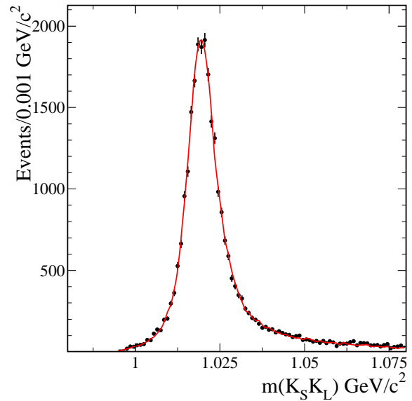
FIG. 10: The K_S^0 K_L^0 invariant mass distribution in the \phi(1020) region. Only statistical uncertainties are shown. The curve represents the result of the fit described in the text.
