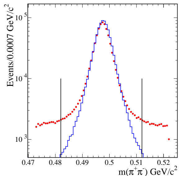
FIG. 1: The \pi^+\pi^- invariant mass distribution for the selected K_S^0 candidates for the data (points) and simulation (histogram). The vertical lines indicate the signal region.
