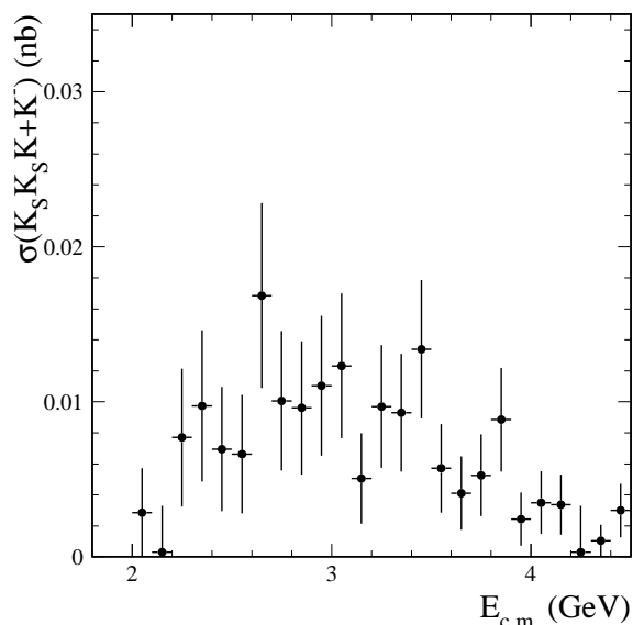
FIG. 37: The e^+e^- \rightarrow K_S^0 K_S^0 K^+ K^- cross section. Events with invariant mass within 0.05 \text{ GeV}/c^2 of the J/\psi mass are excluded.
