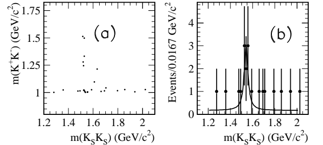
FIG. 42: (a) The K^+ K^- versus K_S^0 K_S^0 invariant mass for the K_S^0 K_S^0 K^+ K^- events under the J/\psi peak (see text). (b) The K_S^0 K_S^0 invariant mass distribution for the events in (a) with m(K^+ K^-) < 1.04 \text{ GeV}/c^2 . The line represents the result of the fit described in the text.
