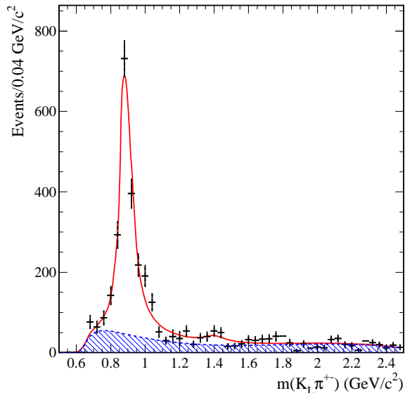
FIG. 23: The number of K^*(892)^\pm events obtained from fits to the K_S^0\pi^\pm invariant mass distribution in each 0.04 \text{ GeV}/c^2 interval of K_L^0\pi^\mp mass. The curve represents the result of the fit described in the text, with the hatched areas representing the non-resonant component.
