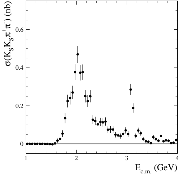
FIG. 29: The e^+ e^- \rightarrow K_S^0 K_S^0 \pi^+ \pi^- cross section.
