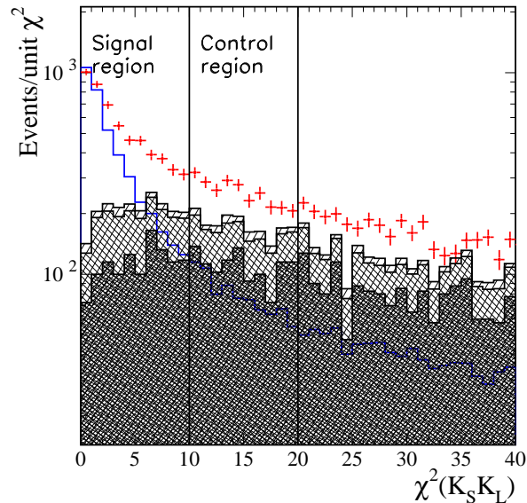
FIG. 12: The 3C \chi^2 distributions for K_S^0 K_L^0 \gamma candidate events in the data (points) and signal simulation (open histogram), fitted under the K_S^0 K_L^0 hypothesis. The shaded, cross-hatched, and hatched areas represent the simulated contributions from the ISR \phi\eta , K_S^0 K_L^0 \pi^0 , and K_S^0 K_L^0 \pi^0 \pi^0 channels, respectively.
