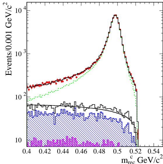
FIG. 3: The experimental m_{\text{rec}}^c distribution (points) compared with our estimated background contributions from (cumulatively): K_s^0 K_L^0 2\pi^0 \gamma (shaded area), K_s^0 K_L^0 \pi^0 \gamma (hatched), and \phi(K_s^0 K_L^0) \eta \gamma (open histogram). The simulated signal distribution is shown as the dashed histogram and the sum of all simulated events as the solid histogram.
