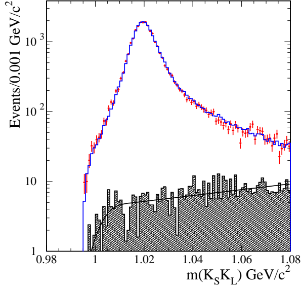
FIG. 7: The K_S^0 K_L^0 invariant mass distribution in the data (points) and signal-MC simulation (histogram) for candidate events in the signal region of Fig. 6. The shaded histogram represents the estimated background, and the line is a smooth parametrization thereof.
