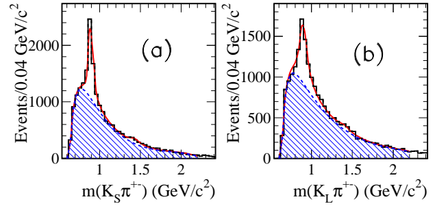
FIG. 22: The (a) K_S^0 \pi^\pm and (b) K_L^0 \pi^\pm mass projections of Fig. 21. The curves represent the results of the fits described in the text, with the hatched areas representing the non-resonant components.
