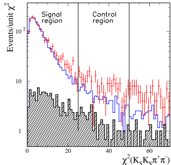
FIG. 25: The four-constraint \chi^2 distributions for K_S^0 K_S^0 \pi^+ \pi^- \gamma candidate events selected in the data (points) and signal-MC simulation (open histogram) fitted under the K_S^0 K_S^0 \pi^+ \pi^- hypothesis. The cross-hatched histogram represents the simulated background contribution from non-ISR q\bar{q} events.
