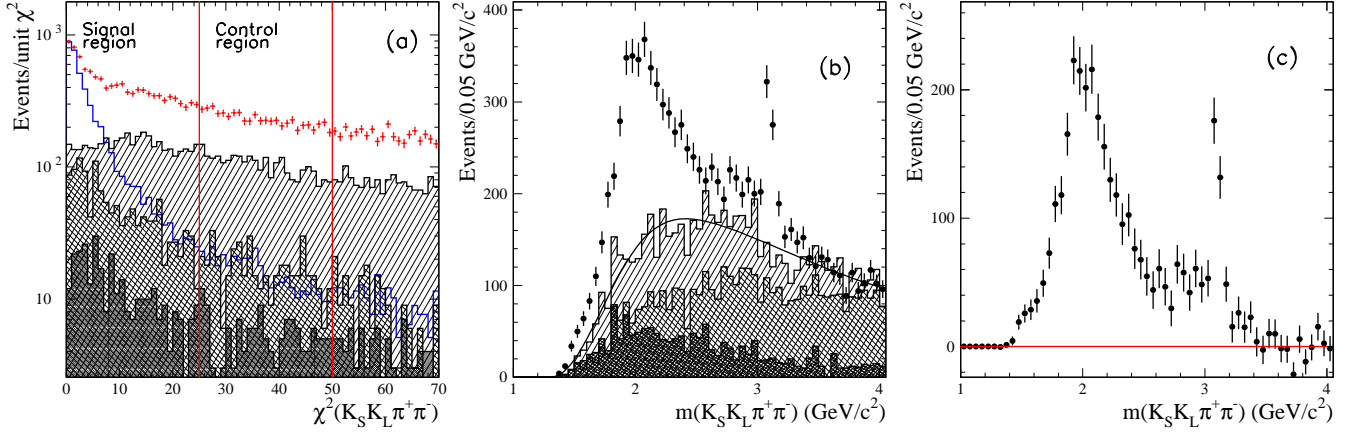
FIG. 18: (a) The three-constraint \chi^2 distributions for data (points) and MC simulated K_S^0 K_L^0 \pi^+ \pi^- \gamma events (open histogram). The shaded, cross-hatched, and hatched histograms represent the simulated contributions from ISR \phi\eta , ISR K_S^0 K \pi \pi^0 , and non-ISR q\bar{q} events, respectively. (b) The K_S^0 K_L^0 \pi^+ \pi^- invariant mass distribution for data events in the signal region of (a) (points). The shaded and cross-hatched histograms represent the simulated contributions from ISR \phi\eta + K_S^0 K \pi \pi^0 and non-ISR q\bar{q} events, respectively, and the hatched area represents that estimated from the control region. The curve shows the empirical fit used for background subtraction. (c) The K_S^0 K_L^0 \pi^+ \pi^- invariant mass distribution after background subtraction.
