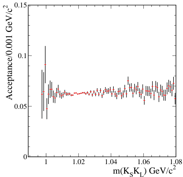
FIG. 9: The simulated detection efficiency \epsilon(s) versus the generated K_S^0 K_L^0 invariant mass, calculated by dividing the number of events in the signal region of Fig. 6 by the number generated in each bin.
