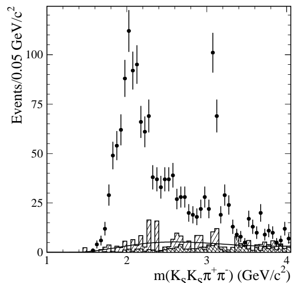
FIG. 27: The K_s^0 K_s^0 \pi^+ \pi^- invariant mass distribution (points) for events in the signal region of Fig. 25. The cross-hatched and hatched histograms represent the backgrounds from non-ISR q\bar{q} events and others estimated from the \chi^2 control region of Fig. 25, respectively. The curve represents the smooth empirical fit to the total background used for subtraction.
