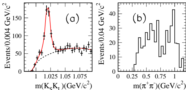
FIG. 24: (a) The K_S^0 K_L^0 invariant mass distribution for the selected K_S^0 K_L^0 \pi^+ \pi^- events. The solid and dashed lines represent the result of the fit described in the text and its non- \phi component, respectively. (b) The \pi^+ \pi^- invariant mass distribution for events in the \phi peak (see text).
