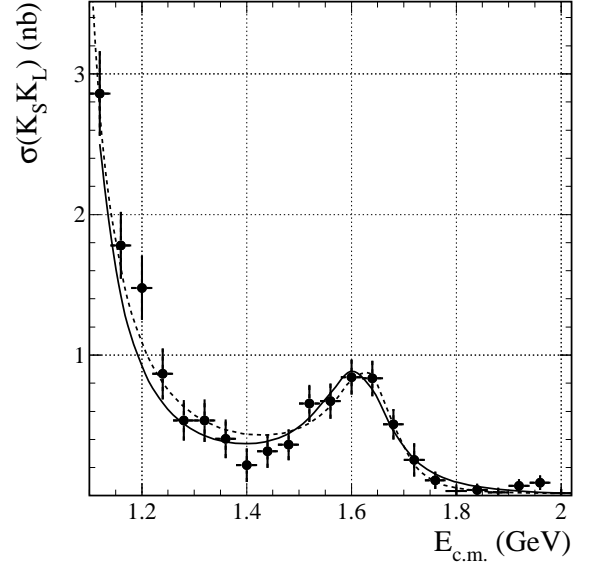
FIG. 16: The e^+e^- \rightarrow K_S^0 K_L^0 cross section (points) compared with the results of the fits described in the text with the non-resonant amplitude fixed to zero (solid lines) and floating (dashed lines).
