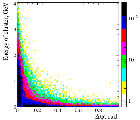
FIG. 4: The EMC cluster energy versus the opening angle between the measured cluster direction and the predicted K_L^0 direction for all non-ISR clusters in the data.
