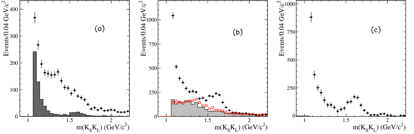
FIG. 13: The K_S^0 K_L^0 invariant mass distribution for data (circles) in the \chi^2 control (a) and signal (b) regions (see Fig. 12). The histogram in (a) represents MC-simulated signal events in the control region, and that in (b) represents the simulated background from \phi\eta , K_S^0 K_L^0 \pi^0 , and K_S^0 K_L^0 2\pi^0 events; The squares show the total estimated background, obtained as the difference between the data and simulated distributions in (a), normalized to the data in the signal region. (c) The K_S^0 K_L^0 invariant mass distribution above 1.06 GeV/ c^2 for the data after background subtraction.
