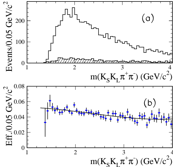
FIG. 19: (a) The K_S^0 K_L^0 \pi^+ \pi^- invariant mass distribution for MC-simulated signal events in the signal (open histogram) and control region (shaded) of Fig. 18. (b) The net reconstruction efficiency from the simulation.
