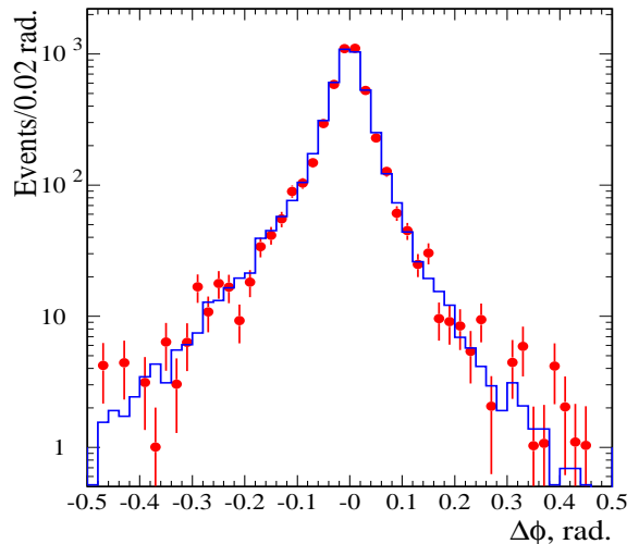
FIG. 5: The difference in azimuthal angle between the EMC cluster direction and the predicted K_L^0 direction for selected clusters in the data (points) and MC-simulated K_s^0 K_L^0(\phi) \gamma events (histogram).
