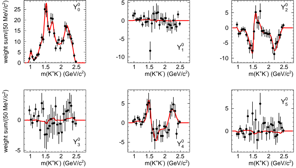
FIG. 7: Legendre polynomial moments for \eta_c \rightarrow K^+ K^- \eta as a function of K^+ K^- mass. The superimposed curves result from the Dalitz plot analysis described in the text.
