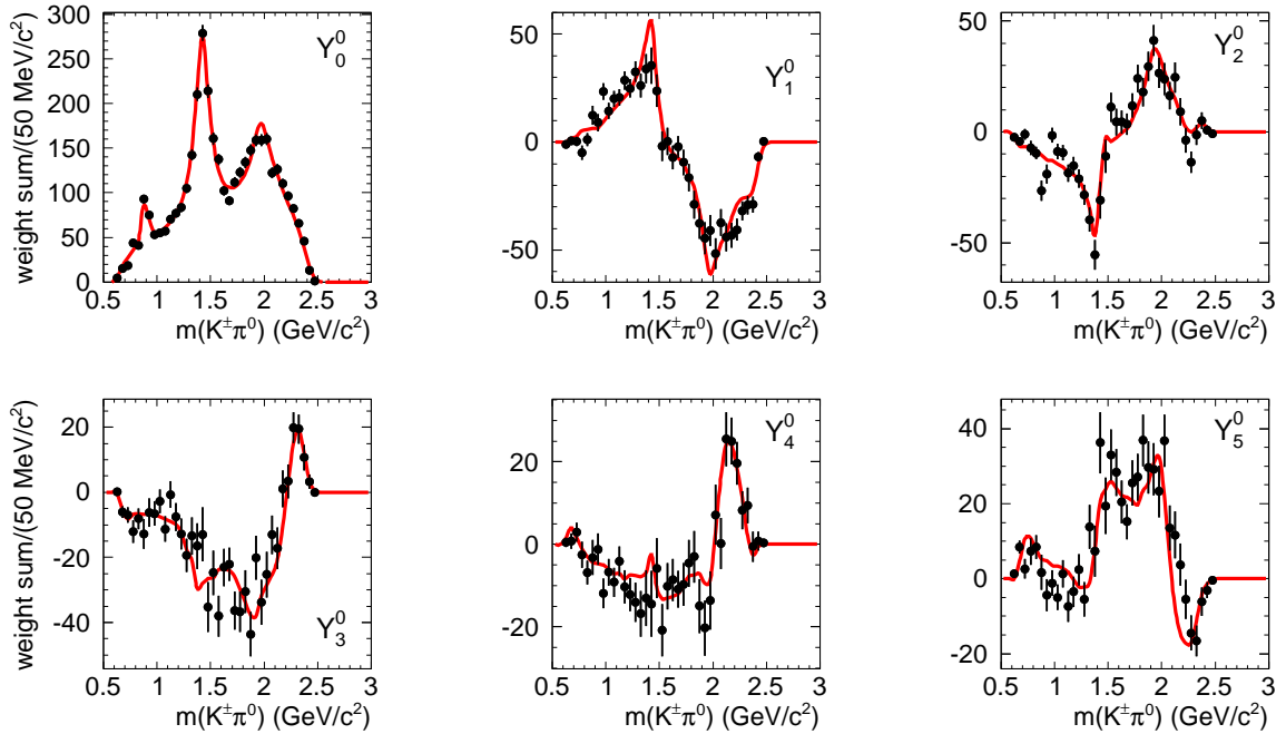
FIG. 12: Legendre polynomial moments for \eta_c \rightarrow K^+ K^- \pi^0 as a function of K^\pm \pi^0 mass. The superimposed curves result from the Dalitz plot analysis described in the text. The corresponding K^+ \pi^0 and K^- \pi^0 distributions are combined.
