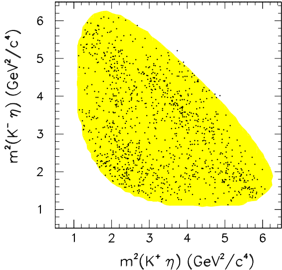
FIG. 5: Dalitz plot for the \eta_c \rightarrow K^+K^-\eta events in the signal region. The shaded area denotes the accessible kinematic region.
