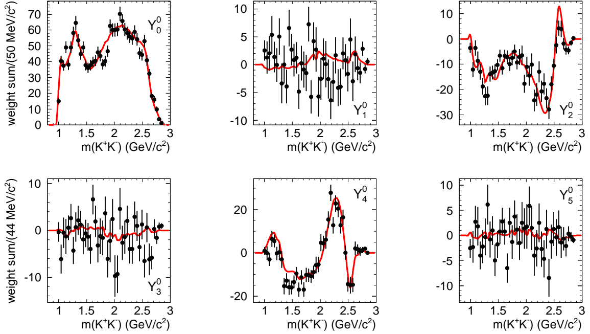
FIG. 11: Legendre polynomial moments for \eta_c \rightarrow K^+ K^- \pi^0 as a function of K^+ K^- mass. The superimposed curves result from the Dalitz plot analysis described in the text.
