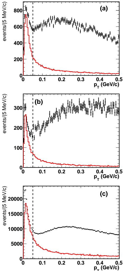
FIG. 1: Distributions of p_T for (a) \gamma\gamma \rightarrow K^+K^-\eta ( \eta \rightarrow \gamma\gamma ), (b) \gamma\gamma \rightarrow K^+K^-\eta ( \eta \rightarrow \pi^+\pi^-\pi^0 ), and (c) \gamma\gamma \rightarrow K^+K^-\pi^0 . In each figure the data are shown as points with error bars, and the MC simulation is shown as a histogram; the vertical dashed line indicates the selection applied to isolate two-photon events.
