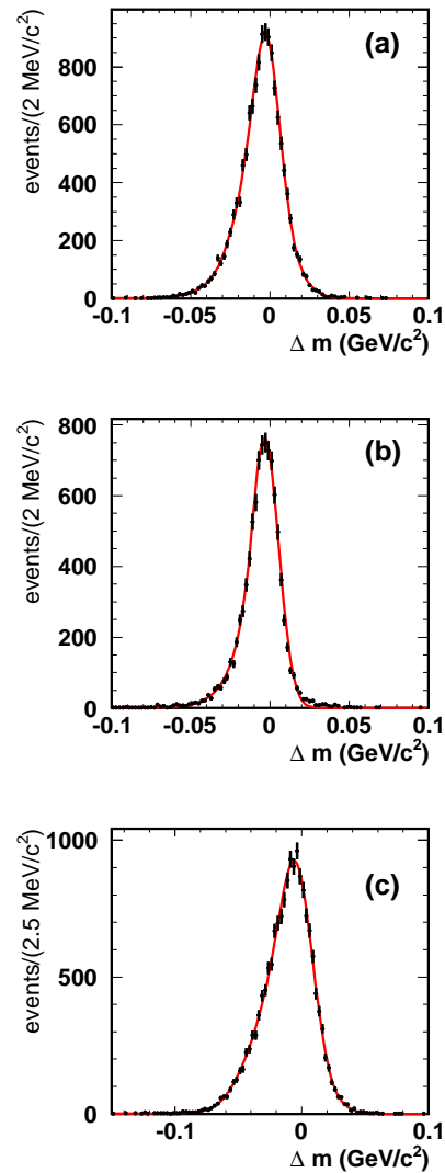
FIG. 3: MC mass resolution for (a) \eta_c \rightarrow K^+K^-\eta ( \eta \rightarrow \gamma\gamma ), (b) \eta_c \rightarrow K^+K^-\eta ( \eta \rightarrow \pi^+\pi^-\pi^0 ), and (c) \eta_c \rightarrow K^+K^-\pi^0 . The curves represent the fits described in the text.
