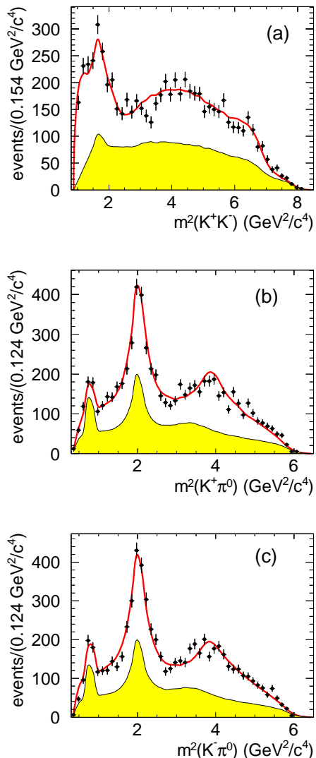
FIG. 10: The \eta_c \rightarrow K^+ K^- \pi^0 Dalitz plot projections. The superimposed curves result from the Dalitz plot analysis described in the text. The shaded regions show the background estimates obtained by interpolating the results of the Dalitz plot analyses of the sideband regions.
