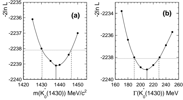
FIG. 13: Likelihood scans as functions of the K_0^*(1430) (a) mass and (b) width. The horizontal (dotted) lines indicate the \Delta(-2\ln\mathcal{L}) = 1 positions, the solid line the likelihood minimum, and the vertical (dashed) lines the uncertainty ranges.
