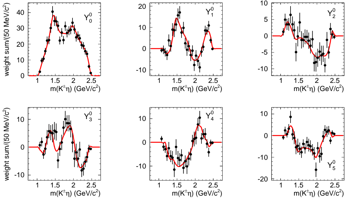
FIG. 8: Legendre polynomial moments for \eta_c \rightarrow K^+ K^- \eta as a function of K^\pm \eta mass. The superimposed curves result from the Dalitz plot analysis described in the text. The corresponding K^+ \eta and K^- \eta distributions are combined.
