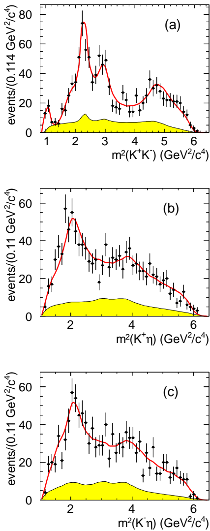
FIG. 6: The \eta_c \rightarrow K^+ K^- \eta Dalitz plot projections. The superimposed curves result from the Dalitz plot analysis described in the text. The shaded regions show the background estimates obtained by interpolating the results of the Dalitz plot analyses of the sideband regions.
