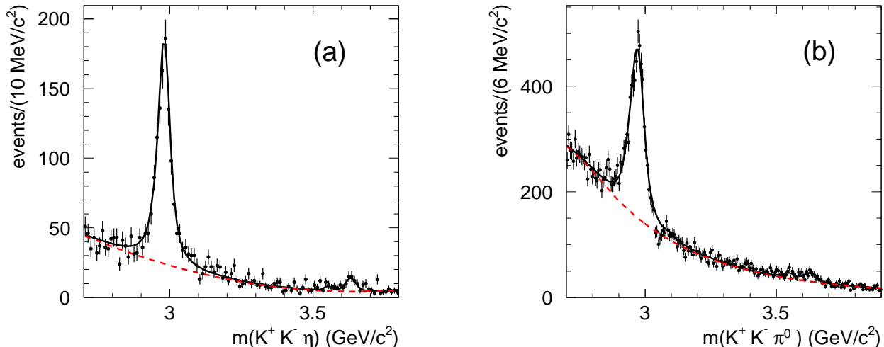
FIG. 4: (a) The K^+K^-\eta mass spectrum summed over the two \eta decay modes. (b) The K^+K^-\pi^0 mass spectrum. In each figure, the solid curve shows the total fitted function and the dashed curve shows the fitted background contribution.
