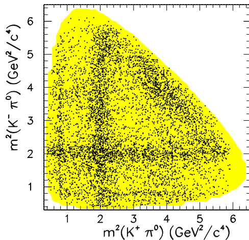
FIG. 9: Dalitz plot for the events in the \eta_c \rightarrow K^+ K^- \pi^0 signal region. The shaded area denotes the accessible kinematic region.
