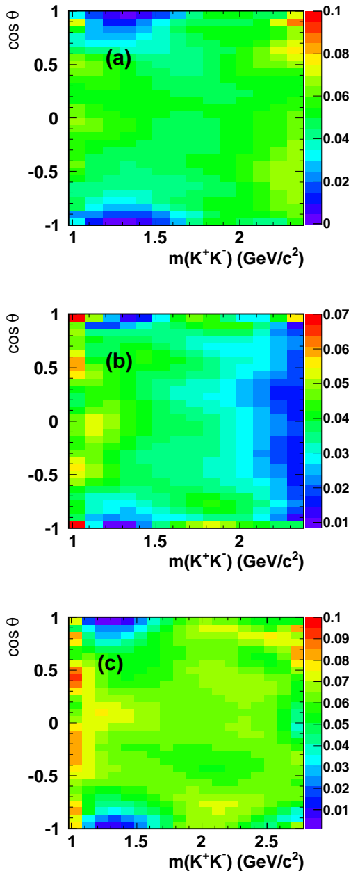
FIG. 2: Fitted detection efficiency in the \cos\theta vs. m(K^+K^-) plane for (a) \eta_c \rightarrow K^+K^-\eta ( \eta \rightarrow \gamma\gamma ), (b) \eta_c \rightarrow K^+K^-\eta ( \eta \rightarrow \pi^+\pi^-\pi^0 ), and (c) \eta_c \rightarrow K^+K^-\pi^0 . Each bin shows the average value of the fit in that region.
