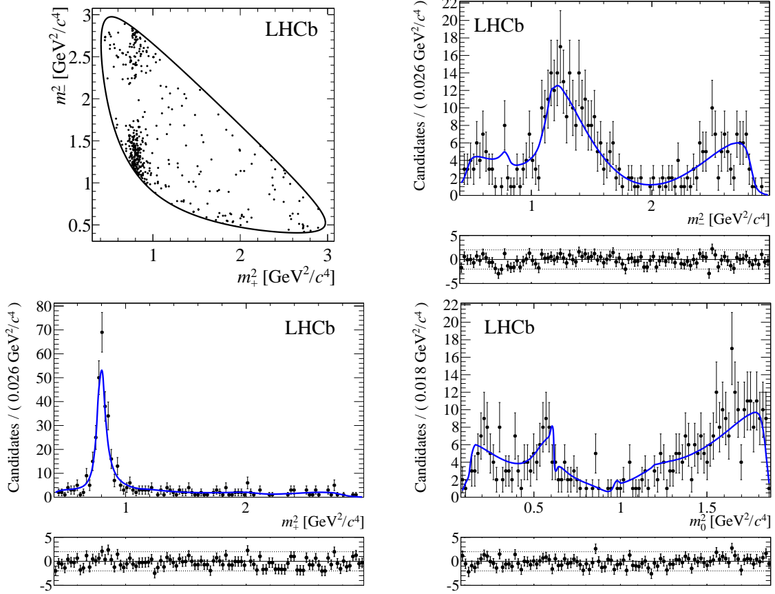
Figure 5: Dalitz plot and its projections, with fit result superimposed, for B^+ \rightarrow DK^+ candidates; m_{\pm}^2 \equiv m_{K_S^0 \pi^{\pm}}^2 and m_0^2 \equiv m_{\pi^+ \pi^-}^2 . The lower parts of the figures are normalised residual distributions.
