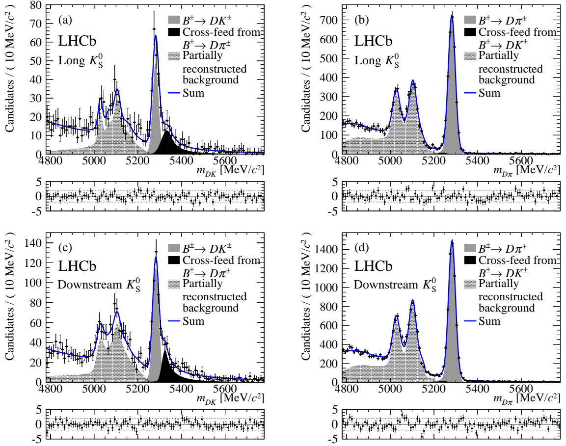
Figure 1: Invariant mass distributions for (a) B^\pm \rightarrow D(\rightarrow K_S^0 \pi^+ \pi^-) K^\pm long , (b) B^\pm \rightarrow D(\rightarrow K_S^0 \pi^+ \pi^-) \pi^\pm long , (c) B^\pm \rightarrow D(\rightarrow K_S^0 \pi^+ \pi^-) K^\pm downstream and (d) B^\pm \rightarrow D(\rightarrow K_S^0 \pi^+ \pi^-) \pi^\pm downstream candidates. The fit results, including signal and background components, are superimposed. The lower plots are normalised residual distributions.
