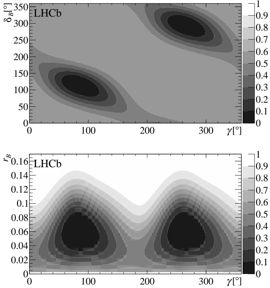
Figure 7: Projections of the p-value regions onto the (\gamma, \delta_B) and (\gamma, r_B) planes with all sources of uncertainty taken into account.
