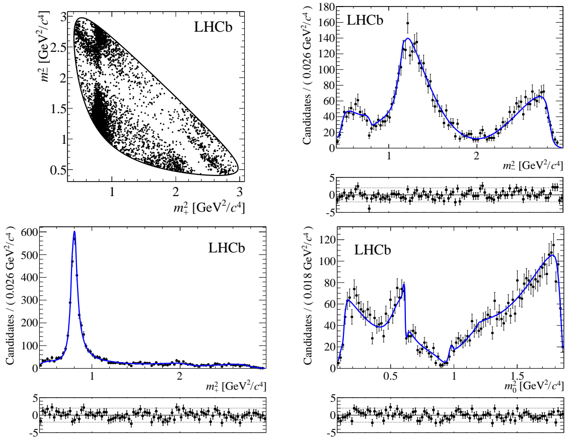
Figure 3: Dalitz plot and its projections, with fit result superimposed, for B^+ \rightarrow D\pi^+ candidates; m_{\pm}^2 \equiv m_{K_S^0\pi^{\pm}}^2 and m_0^2 \equiv m_{\pi^+\pi^-}^2 . The lower parts of the figures are normalised residual distributions.
