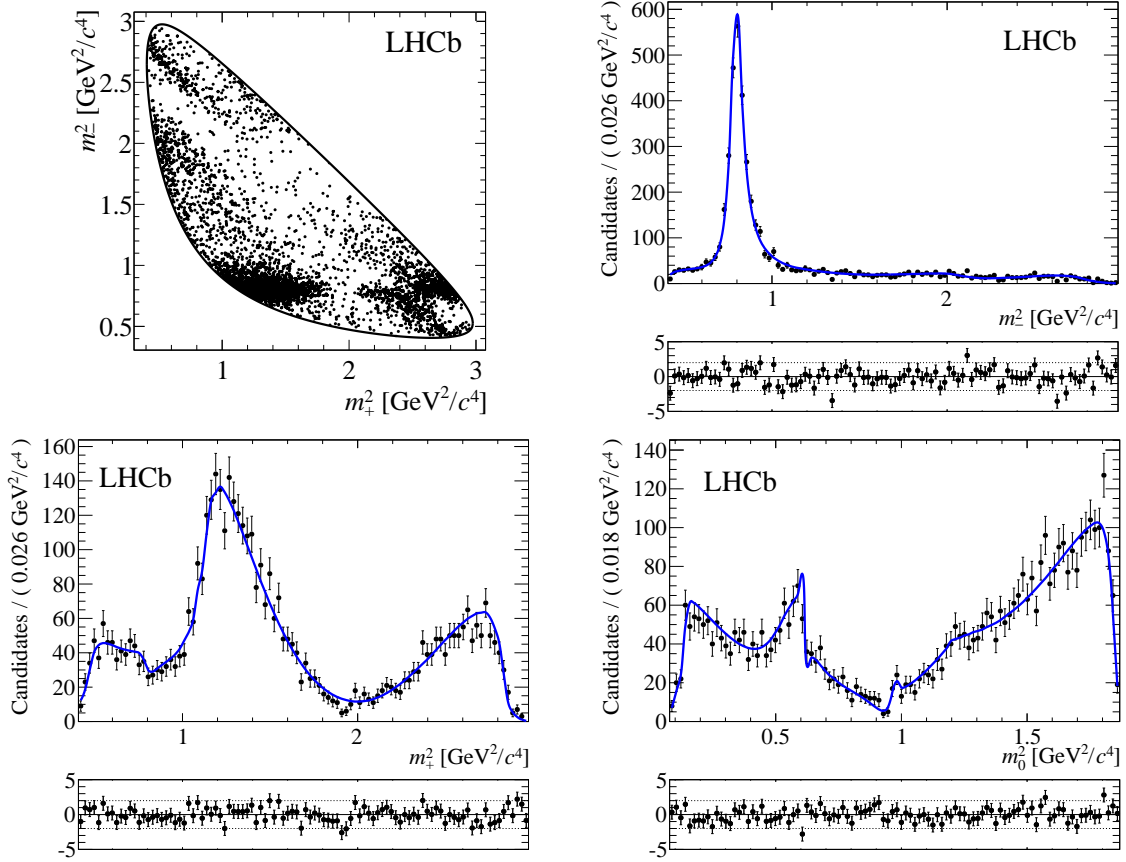
Figure 2: Dalitz plot and its projections, with fit result superimposed, for B^- \rightarrow D\pi^- candidates; m_{\pm}^2 \equiv m_{K_S^0\pi^{\pm}}^2 and m_0^2 \equiv m_{\pi^+\pi^-}^2 . The lower parts of the figures are normalised residual distributions.
