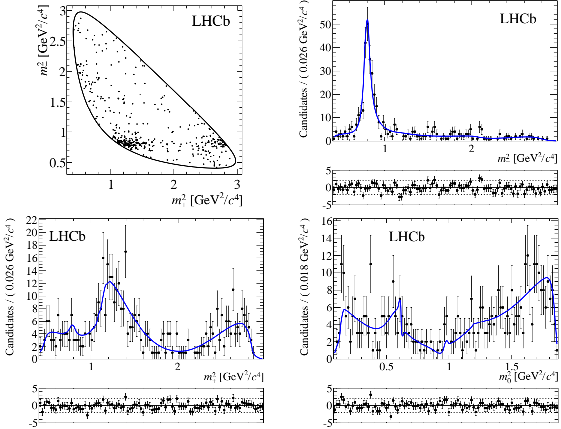
Figure 4: Dalitz plot and its projections, with fit result superimposed, for B^- \rightarrow DK^- candidates; m_{\pm}^2 \equiv m_{K_s^0 \pi^{\pm}}^2 and m_0^2 \equiv m_{\pi^+ \pi^-}^2 . The lower parts of the figures are normalised residual distributions.
