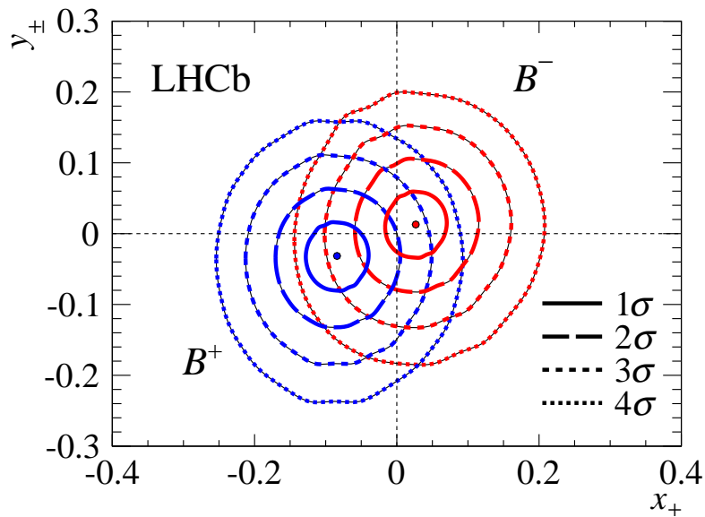
Figure 6: Likelihood contours at 39.35%, 86.47%, 98.89% and 99.97% confidence level for (x_+, y_+) (blue) and (x_-, y_-) (red).
