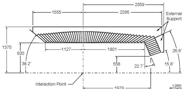
Figure 2.2.10. Longitudinal section of the BABAR EMC (Au- bert, 2002j) showing the arrangement of the 56 CsI(Tl) crystal rings: 48 for the barrel and 8 for the forward end cap. All dimensions quoted on the drawing are in mm.
