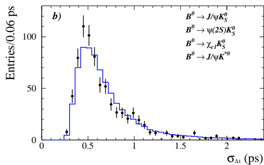
Figure 6.5.2. Distribution of event-by-event uncertainty on \Delta t for the J/\psi K_S^0 , \psi(2S) K_S^0 , \chi_{c1} K_S^0 and J/\psi K^{*0} events. The histogram corresponds to Monte Carlo simulation and the points with error bars to BABAR data. From (Aubert, 2002a).
