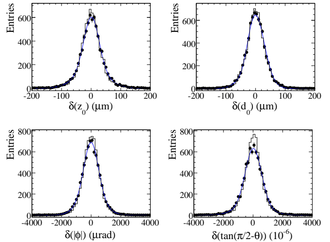
Figure 6.2.2. Measurements of the differences between the fitted track parameters of the top and bottom stubs of cosmic ray muons with a momentum above 2 \text{ GeV}/c in BABAR . The data are shown as points, Monte Carlo simulation as histograms. The (blue) smooth curves are the results of a Gaussian fit to the data. From (Brown, Gritsan, Guo, and Roberts, 2009).
