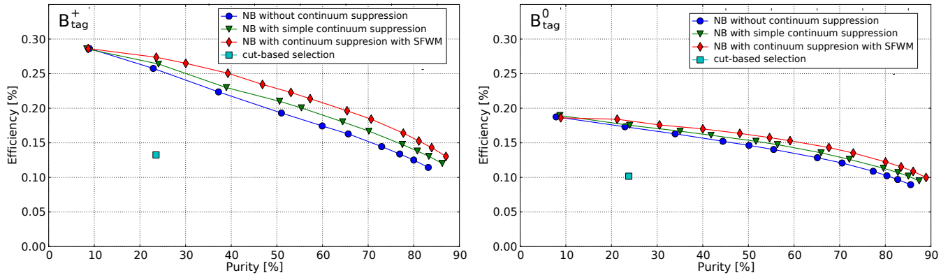
Figure 7.4.3. Purity-efficiency plots for hadronic B_{\text{tag}}^+ (left) and B_{\text{tag}}^0 (right) as obtained by Belle with neural network based selection (NB) and cut-based selection (Feindt et al., 2011). The network based selection can include no continuum suppression variables (blue), only simple ones (green) or Super-Fox-Wolfram moments (SFWM; red).
