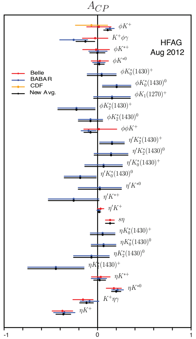
Figure 17.4.15. A_{CP} measurements for kaonic modes with \eta or \phi (Amhis et al. (2012)).
