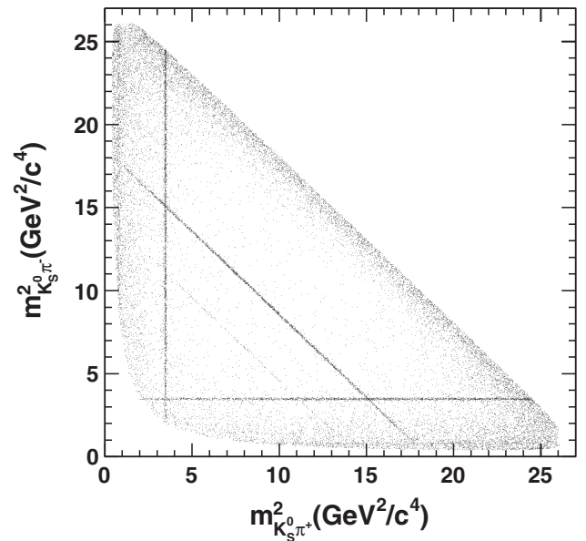
Figure 17.4.17. Dalitz Plot of data selected from B^0 \rightarrow K_S^0 \pi^+ \pi^- decays (Aubert, 2009av). The narrow bands correspond to D^\pm \pi^\mp , J/\psi K_S^0 , and \psi(2S) K_S^0 background events. As in many charmless B meson decay Dalitz Plots, the events of interest are often at the edges of the allowed kinematic region.
