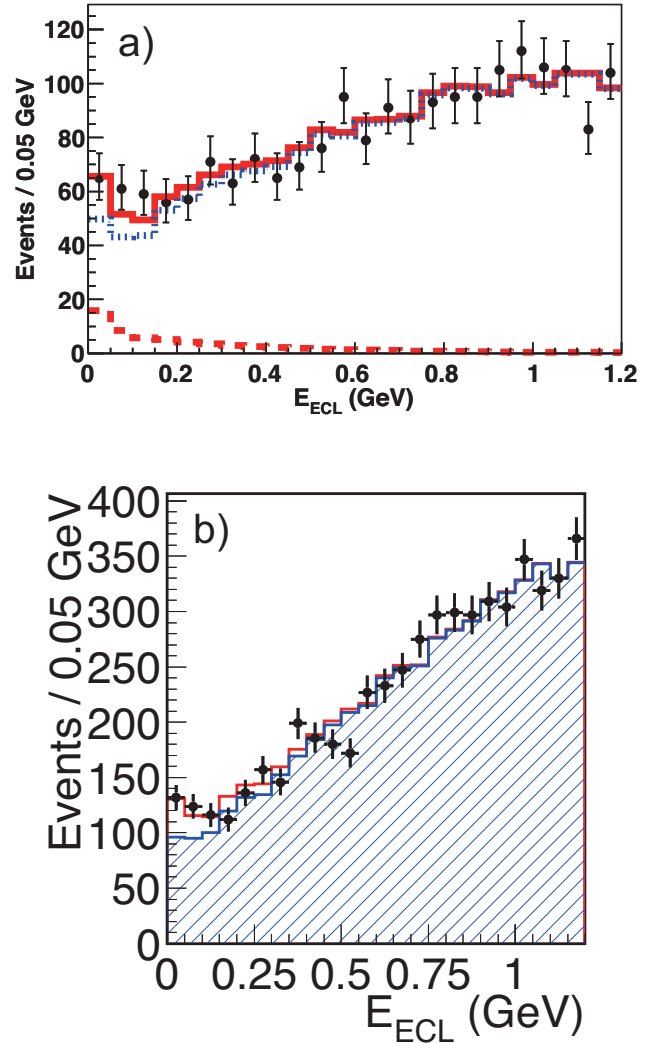
Figure 17.10.2. (a) Distribution of residual energy E_{\text{ECL}} (referred to as E_{\text{extra}} in the text) reported by Belle using hadronic tags (Adachi, 2012b). The solid circles with error bars are data. The solid histograms show the projection of the fit. The dashed and dotted histograms show the signal and background components, respectively. (b) The same distribution obtained using semileptonic tagged events (Hara, 2010). The points with error bars are data. The hatched histogram and solid open histogram are the background and the total signal plus background contributions, respectively.
