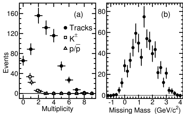
Figure 24.1.9. Background-subtracted distributions for \Lambda_c^+ \Lambda_c^- X events of (a) the numbers of additional tracks in the event and those identified as K^\pm or p\bar{p} , and (b) the missing mass in the event, with imaginary masses given negative real values. Most events have no identified K^\pm or p\bar{p} , and the corresponding zero-multiplicity points are off the vertical scale in (a) (Aubert, 2010b).
