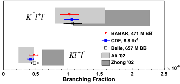
Figure 17.9.13. From (Lees, 2012i). Total branching fractions d\mathcal{B}/dq^2 for B \rightarrow K\ell^+\ell^- and B \rightarrow K^*\ell^+\ell^- from BABAR , CDF and Belle, compared to SM predictions from the models of (Ali, Lunghi, Greub, and Hiller, 2002) and (Zhong, Wu, and Wang, 2003).
