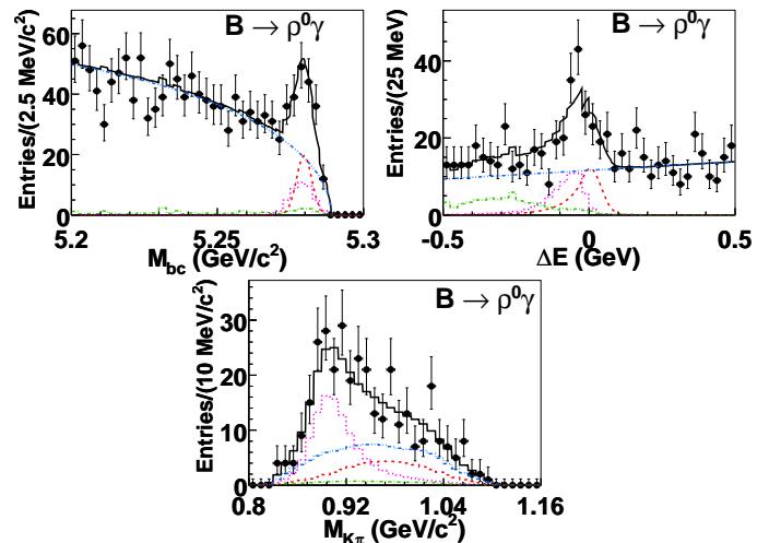
Figure 17.9.8. From (Taniguchi, 2008). Signal for B^0 \rightarrow \rho^0\gamma from Belle in m_{ES} ( =M_{bc} ), \Delta E and M(K\pi) (dashed, red) and backgrounds from B^0 \rightarrow K^*\gamma (dotted, magenta), other B decays (dot-dashed, green) and continuum (dot-dot-dashed, cyan). Each spectrum is made with signal-region cuts on the other plotted quantities.
