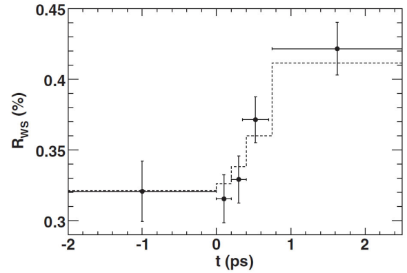
Figure 19.2.12. BABAR (Aubert, 2007j) WS branching fractions R_{WS} for disjoint regions of measured proper time from fits to the (m_{K\pi}, \Delta m) plane (points with error bars). The dashed line shows the expected values of R_{WS} for each slice in proper time assuming the nominal mixing fit results. The \chi^2 with respect to the mixing fit expectation is 1.5; assuming the no-mixing hypotheses (a constant R_{WS} for all time slices), the \chi^2 is 24.
