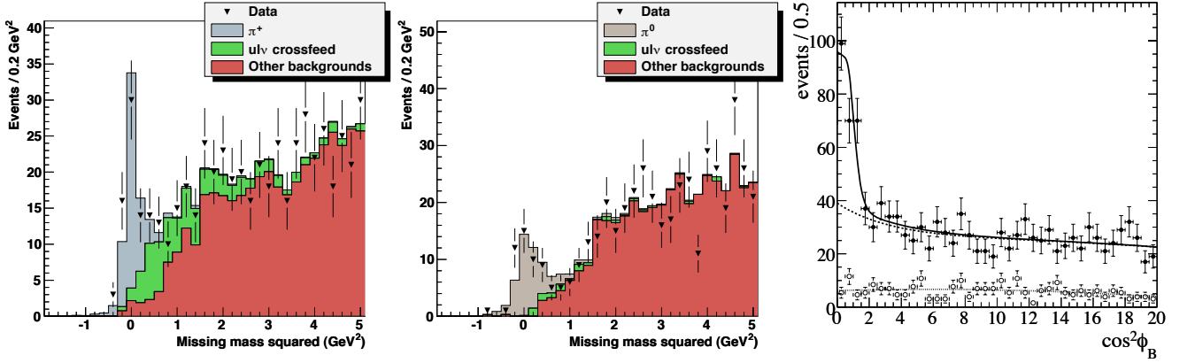
Figure 17.1.14. Missing mass squared distributions from the Belle tagged B^0 \rightarrow \pi^- \ell^+ \nu (left) and B^+ \rightarrow \pi^0 \ell^+ \nu (center) measurements (Adachi, 2008a) and \cos^2 \phi_B distribution from the BABAR semileptonic-tag B^0 \rightarrow \pi^- \ell^+ \nu measurement (Aubert, 2008y) (right). In the right figure, the solid line represents the signal and the dotted and dashed lines represent the backgrounds with combinatorial and with correctly reconstructed D mesons in the semileptonic tag, respectively.
