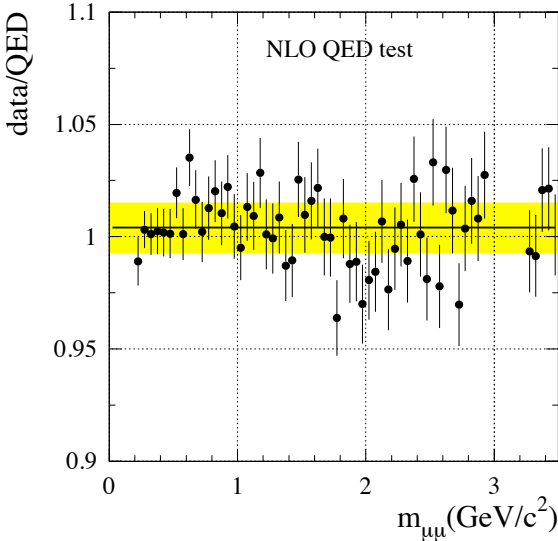
Figure 21.3.2. The ratio of the e^+e^- \rightarrow \mu^+\mu^-\gamma(\gamma) cross section measured by BABAR to the NLO QED prediction (Aubert, 2009ah). The solid line and the shaded band represent the central value and errors given in Eq. (21.3.7).
