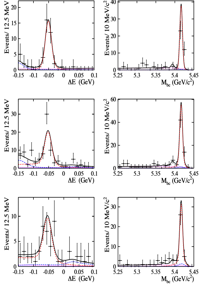
Figure 23.3.6. (left) \Delta E fit projections for events satisfying M_{bc} = m_{ES} \in [5.41, 5.43] \text{ GeV}/c^2 , and (right) m_{ES} fit projections for events satisfying \Delta E \in [-0.08, -0.02] \text{ GeV} . The top row shows B_s^0 \rightarrow D_{(s)}^+ D_s^- ; the middle row shows B_s^0 \rightarrow D_s^{*\pm} D_s^\mp ; and the bottom row shows B_s^0 \rightarrow D_s^{*+} D_s^{*-} . The red dashed curves show correctly reconstructed and wrong combination signal; the blue dash-dotted curves show cross-feed; the magenta dotted curves show background; and the black solid curves show the total. Plots are from Esen (2013).
