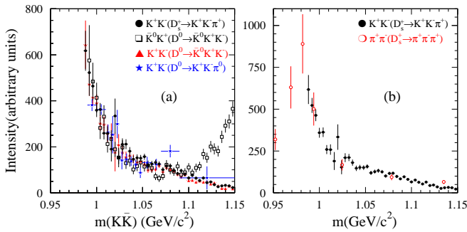
Figure 19.1.34. From (del Amo Sanchez, 2011b). (a) Comparison between K\bar{K} S -wave intensities from different meson Dalitz plot analyses. (b) Comparison of the K\bar{K} S -wave intensity from D_s^+ \rightarrow K^+ K^- \pi^+ with the \pi^+ \pi^- S -wave intensity from D_s^+ \rightarrow \pi^+ \pi^- \pi^+ .
