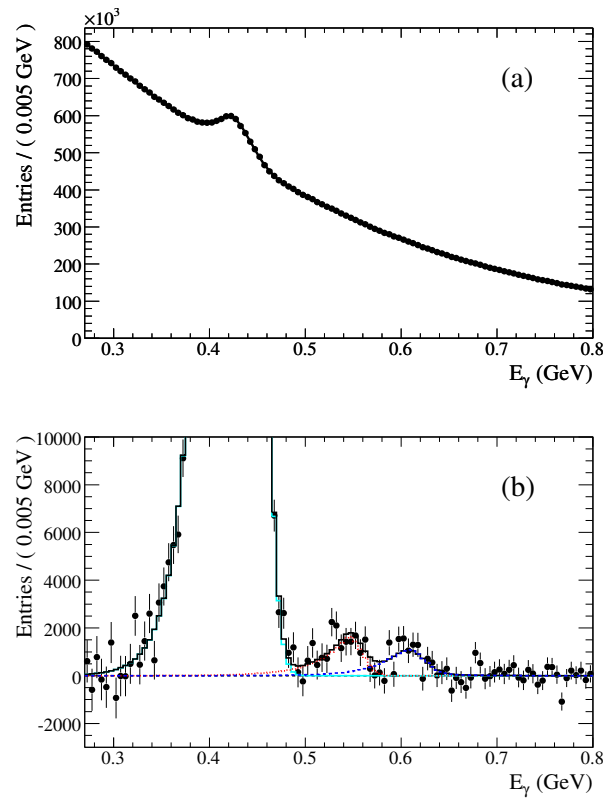
Figure 18.4.6. (a) Inclusive photon spectrum from \Upsilon(2S) decays in the region 0.27 < E_\gamma^* < 0.80 GeV (Aubert, 2009l). The solid line indicates the total fit to the data. (b) The same spectrum after the non-peaking background component has been subtracted, with the \chi_{bJ}(1P) (cyan), ISR (red), and \eta_b (blue) signal components from the fit indicated from left to right on the plot.
