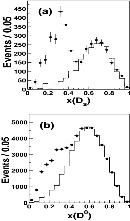
Figure 23.2.3. The D_s^+ normalized momentum x(D_s^+) (a) and the D^0 normalized momentum x(D^0) (b). The points with error bars are the \Upsilon(5S) data, while the histograms show the normalized off-resonance data. Plots are from Drutskoy (2007a).
