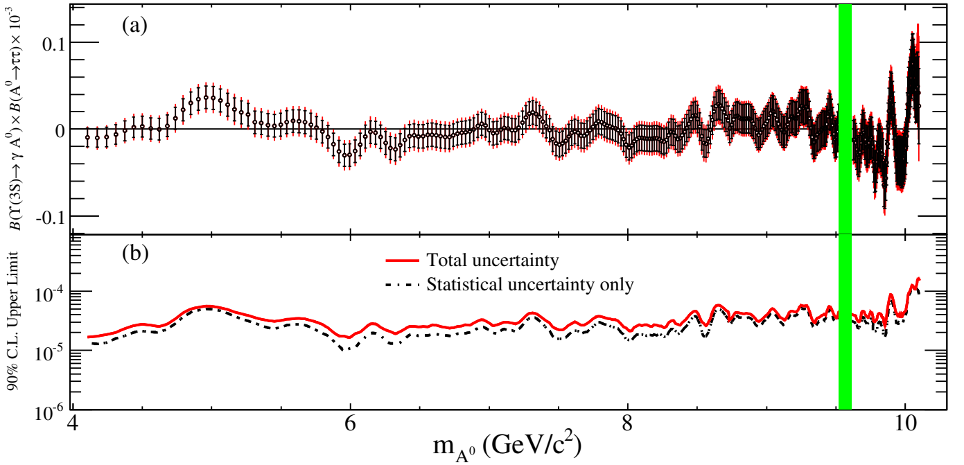
Figure 18.4.24. (a) Product branching fractions as a function of the Higgs mass (Aubert, 2009ai). For each point, both the statistical uncertainty (from the central value to the horizontal bar) and the total uncertainty (statistical and systematic added in quadrature) are shown (from the central value to the end of the error bar). In (b), the corresponding 90% C.L. upper limits on the product of the branching fractions versus the Higgs mass values are shown, with total uncertainty (solid line) and statistical uncertainty only (dashed line). The shaded vertical region represents the excluded mass range corresponding to the \chi_{bJ}(2P) \rightarrow \gamma\Upsilon(1S) states.
