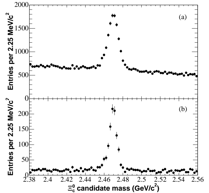
Figure 19.4.10. Invariant mass distribution for the \Xi_c^0 candidates reconstructed in the \Xi^- \pi^+ (upper) and \Omega^- K^+ (lower) decay modes at BABAR. (Aubert, 2005z)
