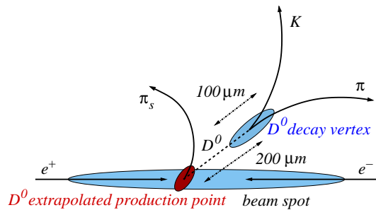
Figure 19.2.7. Illustration of D meson decay length determination with some typical dimensions.
