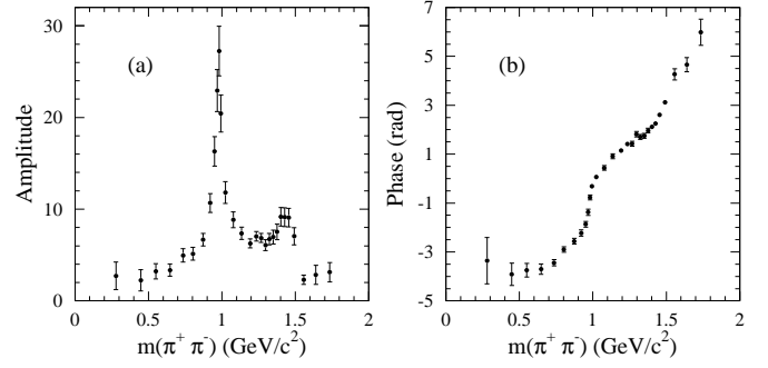
Figure 19.1.29. (a) S -wave amplitude extracted from the D_s^+ \rightarrow \pi^+ \pi^- \pi^+ Dalitz plot analysis. (b) corresponding S -wave phase.
