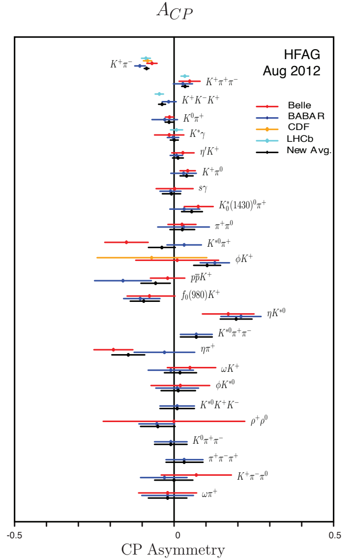
Figure 17.4.13. Summary of the most precise A_{CP} measurements (Amhis et al. (2012)).
