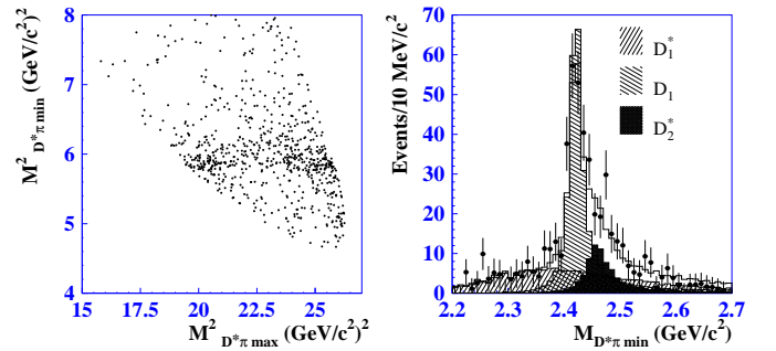
Figure 19.3.6. From (Abe, 2004f). Left: Dalitz plot for the B^- \rightarrow D^{*+} \pi^- \pi^- signal candidates. Right: Background-subtracted M(D^*\pi)_{\min} spectrum. Points with error bars correspond to data, hatched histograms show fitted resonance contributions and the open histogram is a coherent sum of all the contributions. In the figure the D_1^* is indicated as D_1^* .
