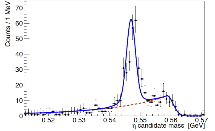
Figure 18.4.21. Signal of \Upsilon(2S) \rightarrow \eta\Upsilon(1S) from the Belle Collaboration result (Tamponi, 2013).
