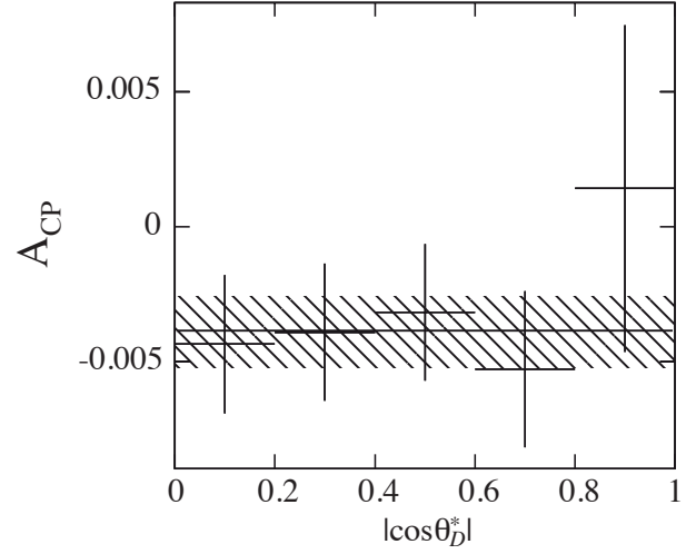
Figure 19.2.29. CP asymmetries for D^+ \rightarrow K_S^0 \pi^+ candidates as a function of |\cos \theta_D^*| . The solid line represents the central value of A_{CP} and the hatched region is the \pm 1\sigma interval, obtained from a minimization assuming no dependence on |\cos \theta_D^*| (del Amo Sanchez, 2011i).
