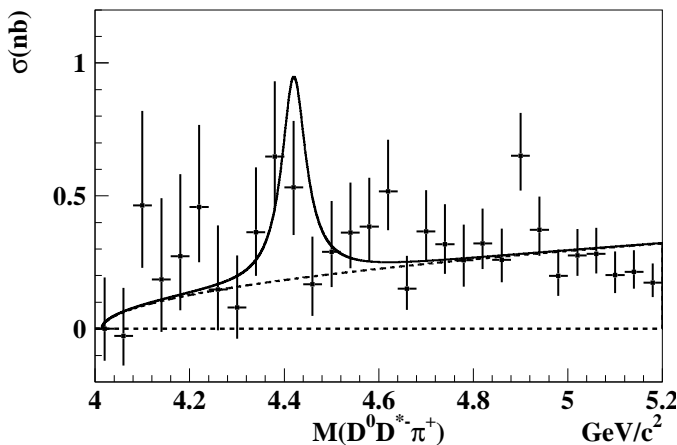
Figure 21.4.9. The exclusive cross section for e^+e^- \rightarrow D^0 D^{*-} \pi^+ averaged over the bin width with statistical uncertainties only from Belle data (Pakhlova, 2009). The total systematic uncertainty is 10%. The fit function corresponds to the 90% C.L. upper limit on \psi(4415) taking into account systematic uncertainties. The solid line represents the sum of the signal and threshold contributions. The threshold function is shown by the dashed line.
