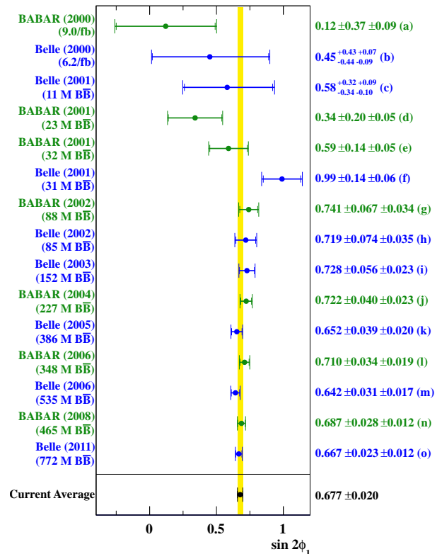
Figure 17.6.8. History of the \sin 2\phi_1 measurements with b \rightarrow c\bar{c}s decays, ordered by the dates they appeared in public. References: (a) (Aubert, 2000), (b) (Aihara, 2000a), (c) (Abashian, 2001), (d) (Aubert, 2001a), (e) (Aubert, 2001e), (f) (Abe, 2001g), (g) (Aubert, 2002g), (h) (Abe, 2002b), (i) (Abe, 2005c), (j) (Aubert, 2005i), (k) (Abe, 2005j), (l) (Aubert, 2006j), (m) (Chen, 2007a), (n) (Aubert, 2009z), (o) (Adachi, 2012c).
