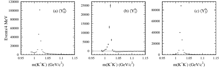
Figure 19.1.32. From (del Amo Sanchez, 2011b). K^+K^- mass spectrum from D_s^+ \rightarrow K^+K^-\pi^+ in the threshold region weighted by (a) Y_0^0 , (b) Y_1^0 , and (c) Y_2^0 , corrected for efficiency and phase space, and background-subtracted.
