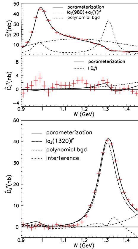
Figure 22.2.2. Spectra of (top) \widehat{S}^2 , (middle) \widehat{D}_0^2 and (bottom) \widehat{D}_2^2 for \gamma\gamma \rightarrow \eta\pi^0 . The solid lines are the results of the partial-wave analysis discussed in Section 22.2.1.2. The error bars show the diagonal components of error matrix for the fit parameters. From (Uehara, 2009a).
