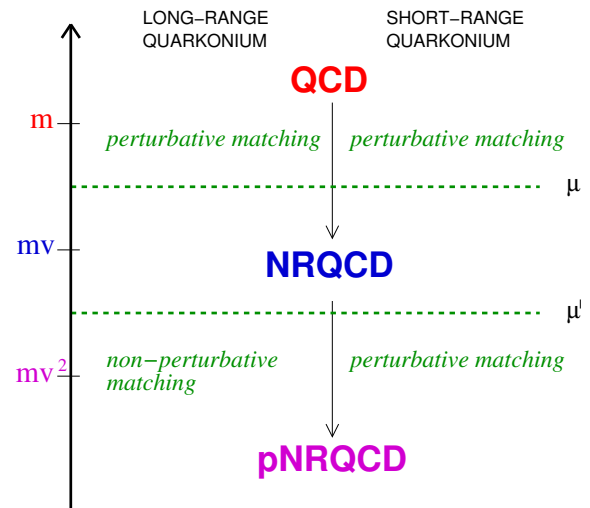
Figure 18.1.2. Energy scales and corresponding effective field theories for quarkonium. The scale \mu separates QCD from NRQCD, while \mu' separates NRQCD from pNRQCD.
