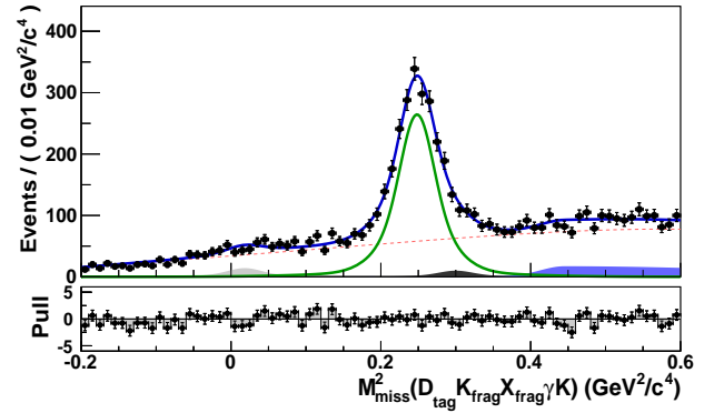
Figure 19.1.6. From (Zupanc, 2013b). M_{miss}^2(D_{tag}KX_{frag}\gamma K) distribution of partially reconstructed D_s^+ \rightarrow \bar{K}^0 K^+ decays within the inclusive D_s sample. The fit result is superimposed and includes fitted signal contribution (solid green line), reflections from charged kaon originating from D_s^+ \rightarrow \eta K^+ and D_s^+ \rightarrow \pi^0 K^+ (full grey histograms) and other true D_s decays (for example D_s^+ \rightarrow \eta\pi^+ with pion being misidentified as kaon) (full blue histogram), and combinatorial background (dashed red line).
