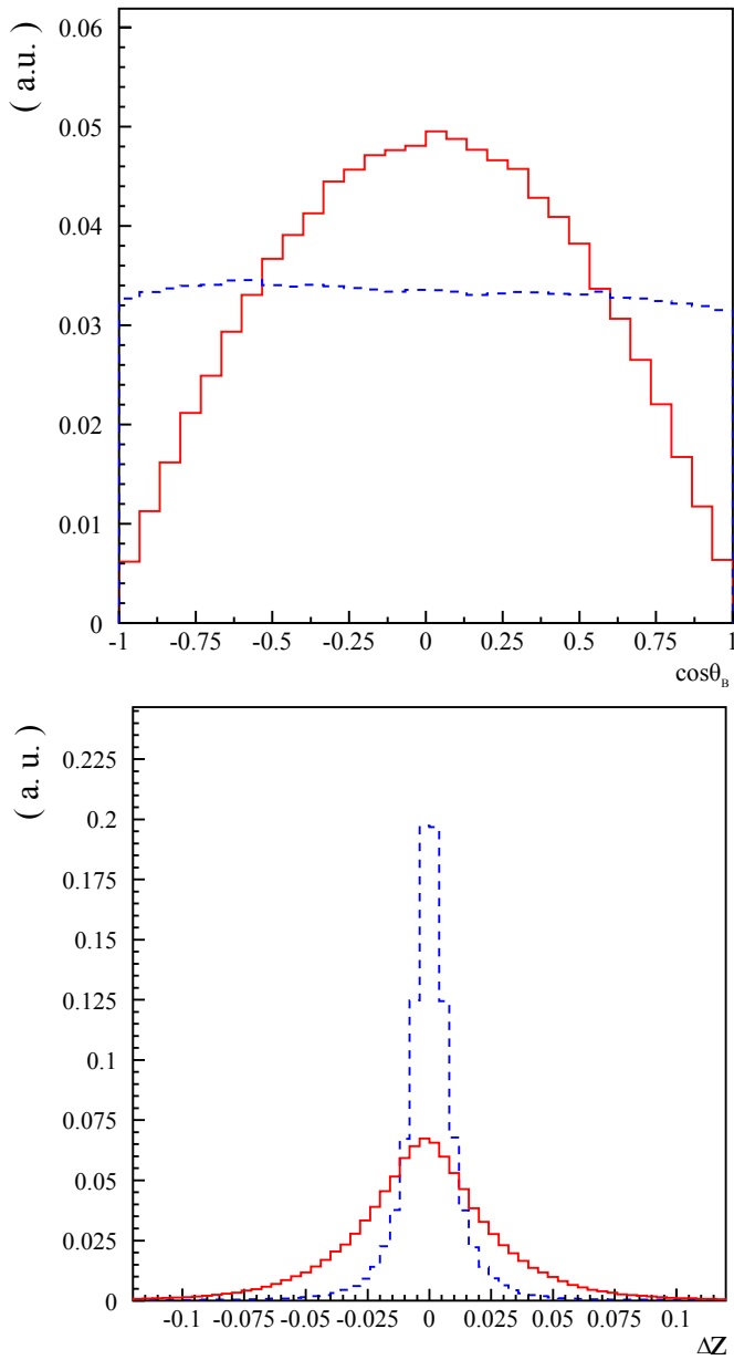
Figure 9.5.1. The \cos\theta_B (top) and \Delta Z (bottom) distributions for the B^+ \rightarrow K^+\pi^0 and continuum MC events. Solid red lines are B signal candidates and dashed blue lines are the continuum background. These figures are Belle internal, from the (Duh, 2012) analysis. The vertical scale is in arbitrary units (a.u.).
