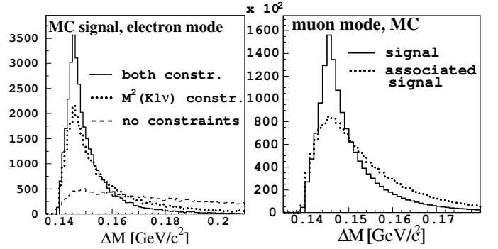
Figure 19.2.22. Left: The effect of the kinematic constraints on the \Delta M distribution of the simulated D^0 \rightarrow K^-e^+\nu_e decays. Right: \Delta M distribution for simulated associated signal events (see text for the explanation). From (Bitenc, 2008).
