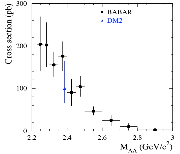
Figure 21.3.22. The e^+e^- \rightarrow \Lambda\bar{\Lambda} cross section measured by BABAR (Aubert, 2007az) in comparison with the DM2 measurement (Bisello et al., 1990).
