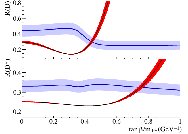
Figure 17.10.10. Comparison of the BABAR measurements of \mathcal{R}(D) (top) and \mathcal{R}(D^*) (bottom) with the prediction of the Type-II 2HDM (red curves). The \tan\beta/M_H dependence of the BABAR \mathcal{R}(D^{(*)}) results (blue shaded bands) arises due to changes to the signal kinematics in the case that the process is mediated by a H^\pm rather than a W^\pm . The SM case corresponds to the case \tan\beta/M_H = 0 , and the favored values for \tan\beta/M_H differ for \mathcal{R}(D) and \mathcal{R}(D^*) . Plot is taken from Lees (2012e).
