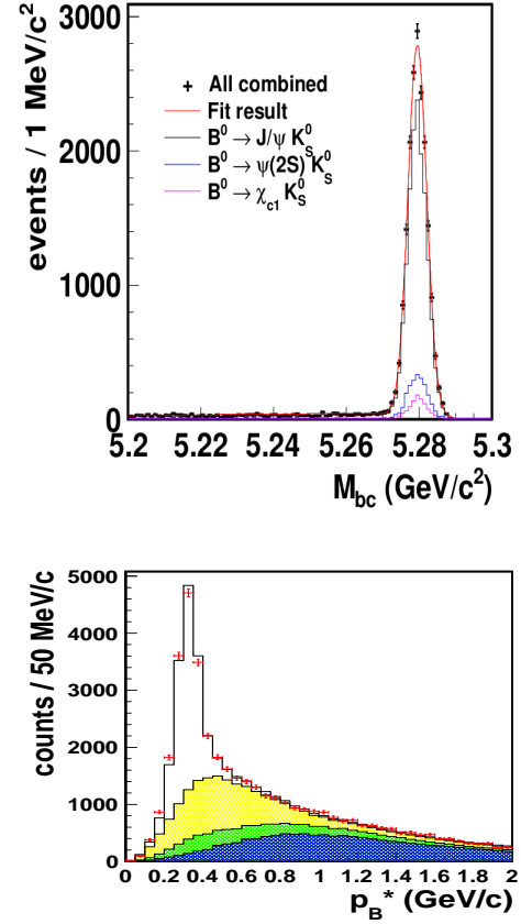
Figure 17.6.6. Distributions of m_{ES} ( = M_{bc} ) for B^0 \rightarrow (c\bar{c})K_S^0 (top) and p_B^* for B^0 \rightarrow J/\psi K_L^0 (bottom) obtained with the samples used for the Belle measurement (Adachi, 2012c) of \phi_1 . The shaded regions in the bottom plot represent the estimated background components: (from top to bottom) real J/\psi and real K_L^0 (yellow), real J/\psi and fake K_L^0 (green), and fake J/\psi (blue).
