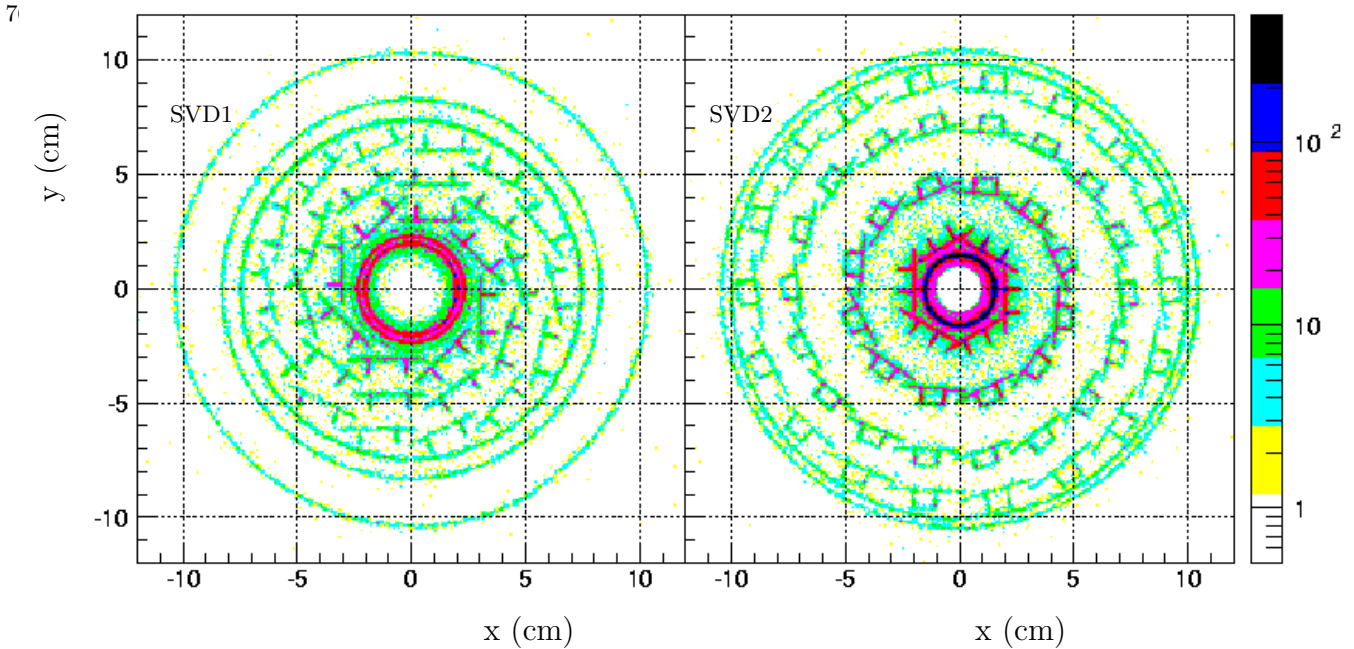
Figure 24.2.3. Distribution of reconstructed secondary pK_S^0 vertices in the Belle detector for both the SVD1 (left) and SVD2 (right) data samples, from Mizuk, Danilov (2006).
