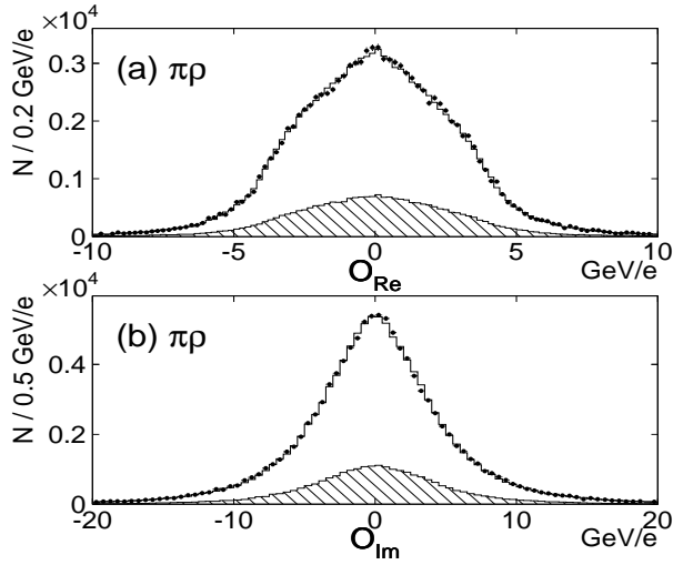
Figure 20.5.1. Distribution of optimal observables, (a) \mathcal{O}_{Re} and (b) \mathcal{O}_{Im} , for \pi\rho events \tau^-\tau^+ \rightarrow (\pi^-\bar{\nu}_\tau)(\rho^+\nu_\tau) (Inami, 2003). Dots are Belle data and white and shaded histograms show the MC simulation for signal and background, respectively. If CP is violated, mean values \langle \mathcal{O}_{Re} \rangle , \langle \mathcal{O}_{Im} \rangle are differ from zero.
