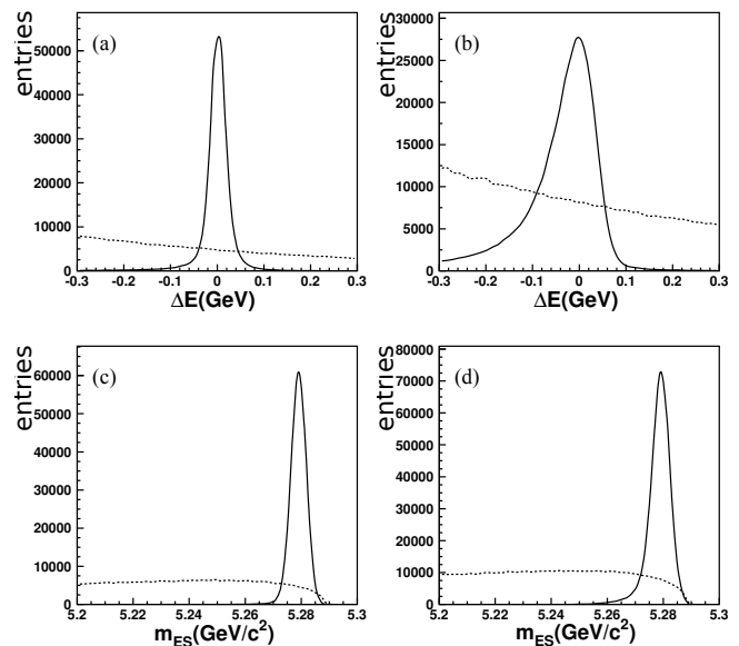
Figure 7.1.2. The \Delta E and m_{\text{ES}} distributions for (a and c) B^+ \rightarrow K_S^0 \pi^+ and (b and d) B^+ \rightarrow K^+ \pi^0 . Solid line histograms are signal events generated using GEANT Monte Carlo and dotted histograms are from the continuum MC. The signal resolution in \Delta E is much worse for B^+ \rightarrow K^+ \pi^0 , due to the neutral pion present in the final state, but the difference is less pronounced in m_{\text{ES}} as explained in the text.
