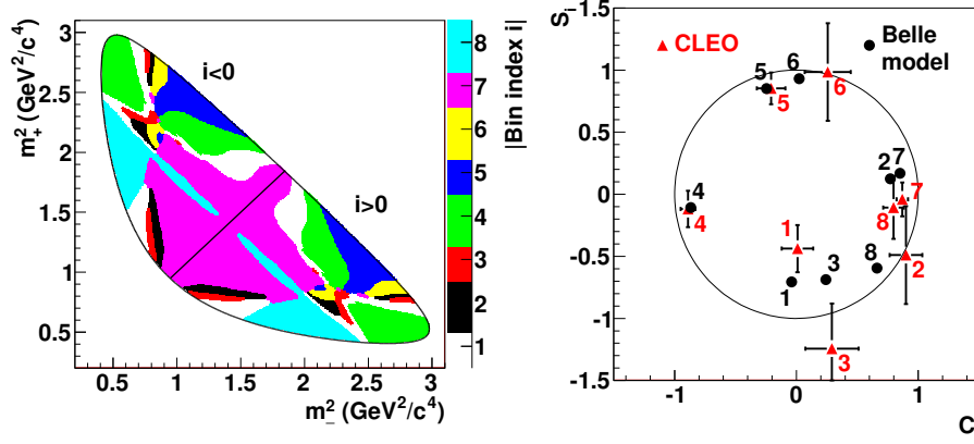
Figure 17.8.10. (a) Optimal binning of the D^0 \rightarrow K_S^0 \pi^+ \pi^- Dalitz plot and (b) comparison of phase terms c_i, s_i for the optimal binning measured by CLEO, and calculated from the Belle D^0 \rightarrow K_S^0 \pi^+ \pi^- amplitude model, taken from Aihara (2012).
