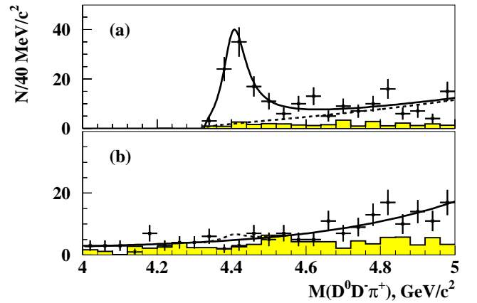
Figure 18.2.13. From Pakhlova (2008c): Mass distributions for D^0 D^- \pi^+ in e^+e^- \rightarrow \gamma_{\text{ISR}} D^0 D^- \pi^+ events. Fit results are shown by the solid curve. (a) The M_{D^0 D^- \pi^+} spectrum for the D\bar{D}_2^*(2460) signal region; the dashed curve corresponds to the non- \psi(4415) contribution. (b) The M_{D^0 D^- \pi^+} spectrum outside the D\bar{D}_2^*(2460) signal region; the dashed curve shows the upper limit on the \psi(4415) yield at the 90% C.L. In both plots, shaded histograms show the normalized contributions from M_{D^0} and M_{D^-} sidebands.
