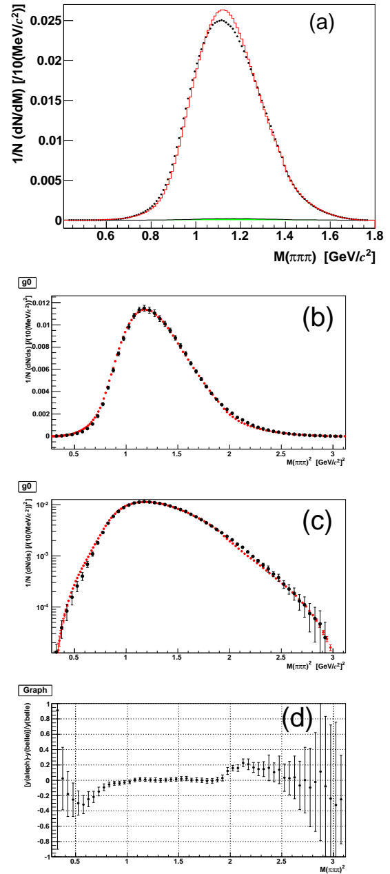
Figure 20.6.3. (color online) (a) Unfolded mass spectrum (1/N)dN/dM for the \pi^{-}\pi^{+}\pi^{-} system in \tau^{-} \rightarrow \pi^{-}\pi^{+}\pi^{-}\nu_{\tau} measured by Belle (Lee, 2010). Solid circles with error bars are the data with statistical errors; solid-red histogram is the spectra implemented in the current TAUOLA program; the horizontal green band at the zero entry line shows the size of the systematic uncertainties for data. (b) Comparison of \pi^{-}\pi^{-}\pi^{+} mass spectra as a function of mass-squared between Belle (red circle) and ALEPH (black circles). (c) in log-scale, (d) the ratio ALEPH/Belle-1.
