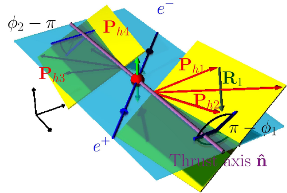
Figure 24.1.14. Azimuthal angles \phi_1 and \phi_2 defined for the two hadron pairs's planes (denoted by the yellow planes) relative to plane spanned by the lepton and thrust axis (blue).
