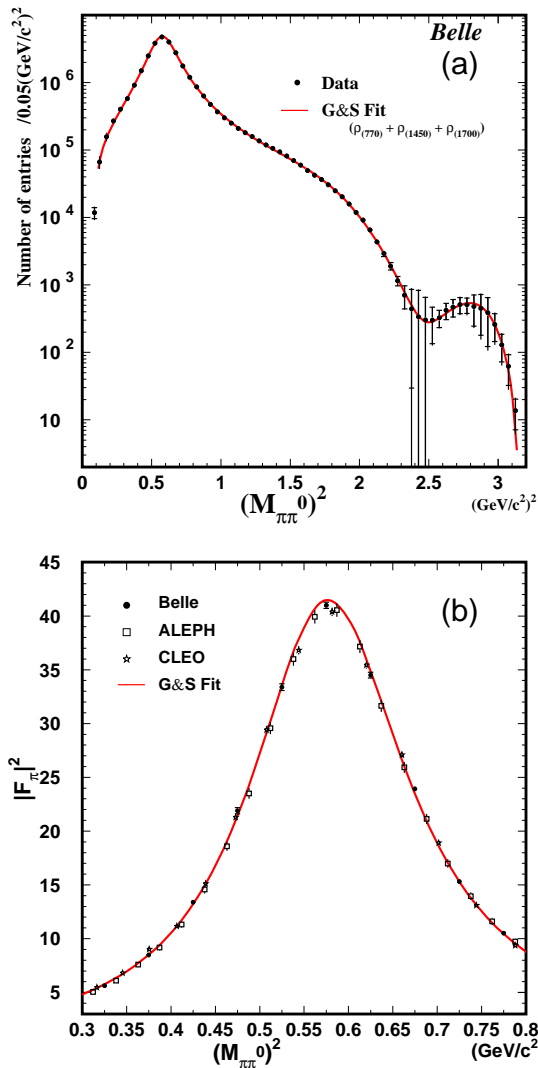
Figure 20.6.2. (a) Unfolded \pi^{\pm}\pi^0 mass spectrum for \tau^{\pm} \rightarrow \pi^{\pm}\pi^0\nu_{\tau} obtained by the Belle experiment (Fujikawa, 2008). Solid circles are the data and the solid line is a fit based on the Gounaris-Sakurai (G&S) parameterization (Gounaris and Sakurai, 1968). The error bars include both statistical and systematic errors. (b) Pion form factor |F_{\pi}(s)|^2 in the \rho(770) region derived from the \pi^{\pm}\pi^0 mass spectrum.
