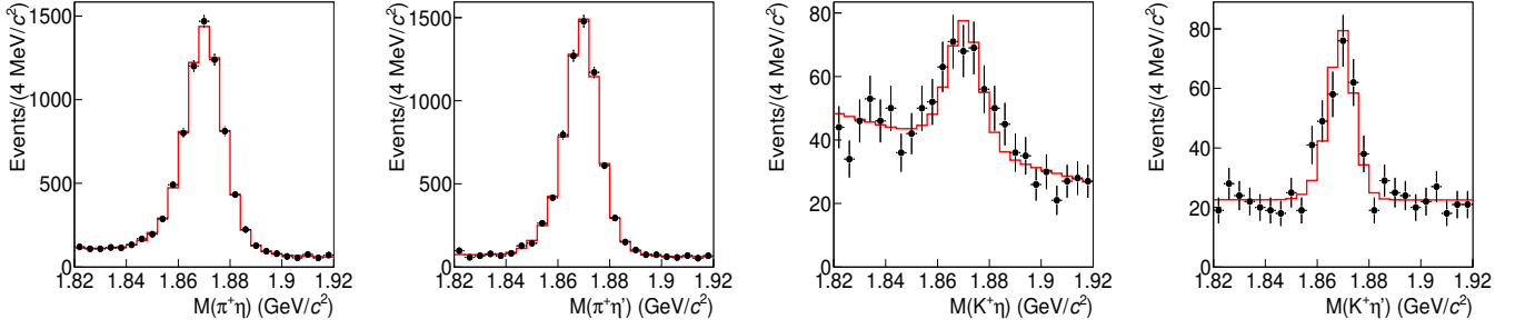
Figure 19.1.12. From (Won, 2011). Invariant mass distributions for the \pi^+\eta , \pi^+\eta' , K^+\eta and K^+\eta' final states. Points with error bars and histograms correspond respectively to the data and fit result.
