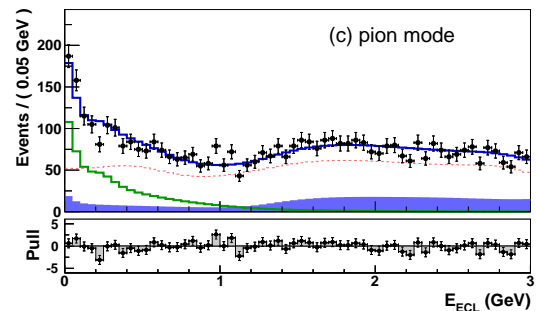
Figure 19.1.41. E_{\text{extra}} ( E_{\text{ECL}} in case of Belle) distribution for D_s^- \rightarrow \tau^- \bar{\nu}_\tau , \tau^- \rightarrow e^- \nu_\tau \bar{\nu}_e (del Amo Sanchez, 2010g) (top) and for D_s^- \rightarrow \tau^- \bar{\nu}_\tau , \tau^- \rightarrow \pi^- \nu_\tau (Zupanc, 2013b). The points represent the data with statistical error bars. In the top plot the open histogram is from the fit, and the solid histogram is the background component from the fit. For the bottom plot the lines represent different components of the fit.
