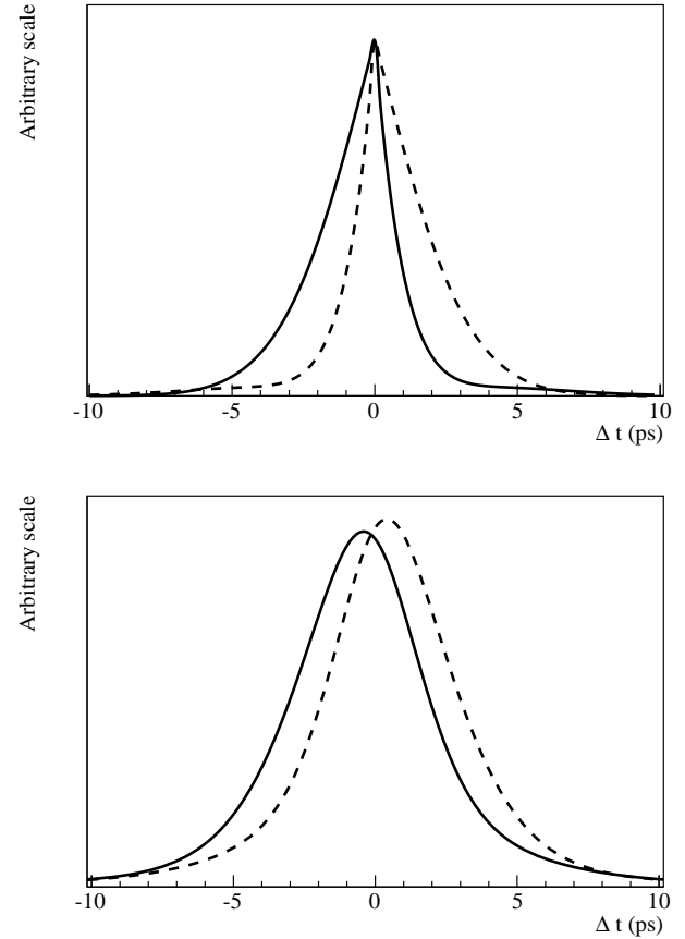
Figure 10.4.1. Distributions of (top) f_{\pm}^{\text{Phys}}(\Delta t) with S = 0.7 , and C = 0.0 for (solid) B^0 - and (dashed) \bar{B}^0 -tagged events for perfectly reconstructed decays, and (bottom) the corresponding distributions F_{\pm}^{\text{Phys}} after taking into account typical dilution and resolution effects.
