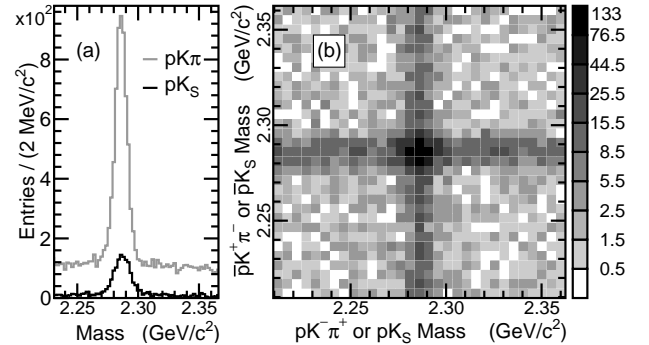
Figure 24.1.8. (a) Invariant mass distributions for \Lambda_c^+ \rightarrow pK^-\pi^+ (gray) and \Lambda_c^+ \rightarrow pK_s^0 (black) candidates in events with both a \Lambda_c^+ and a \bar{\Lambda}_c^- candidate. (b) Invariant mass of the \bar{\Lambda}_c^- candidate vs. that of the \Lambda_c^+ candidate, in 5 \text{ MeV}/c^2 \times 5 \text{ MeV}/c^2 bins (Aubert, 2010b).
