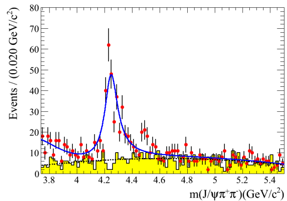
Figure 21.5.3. (upper) The \pi^+\pi^- J/\psi mass spectrum measured by Belle (Yuan, 2007). Points with errors show selected events in the J/\psi signal region, while the histogram shows the scaled J/\psi sideband distribution. The curves show the best fit (solid line) and the contribution from each component for the two solutions, as described in the text. (lower) The \pi^+\pi^- J/\psi mass spectrum measured by BABAR in a 454 \text{ fb}^{-1} data sample (Lees, 2012ab). The solid curve shows the result of a simultaneous fit to the data (points with errors) and to the background control sample obtained from the J/\psi sidebands (shaded histogram).
