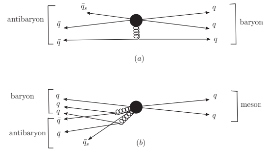
Figure 17.12.12. Short-distance picture in terms of quarks and antiquarks for (a) two-body baryonic decay and (b) three-body baryonic decay. The slow spectator antiquark is denoted by the short line \overline{q}_s .
