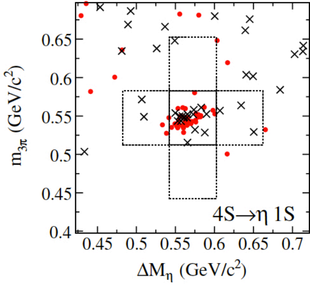
Figure 18.4.20. The distribution of M_{3\pi} vs \Delta M_\eta = M_{3\pi l l} - M_{ll} for \eta\Upsilon(1S) candidate events, demonstrating the observed signal (Aubert, 2008bc). Solid lines delimit the signal region, while dashed lines delimit the sideband regions used for the background estimate. Crosses represent the data from the \Upsilon(1S) \rightarrow e^+e^- sample and dots the data from the \Upsilon(1S) \rightarrow \mu^+\mu^- sample.
