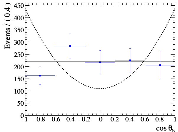
Figure 19.4.4. The helicity angle distribution for \Sigma_c(2455)^0 candidates in B^- \rightarrow \Sigma_c(2455)^0 \bar{p} at BABAR , corrected for efficiency (Aubert, 2008aa). The distributions expected for the spin-1/2 hypothesis (solid, horizontal line) and spin-3/2 hypothesis (dashed curve) are shown. The data are consistent with J = 1/2 and exclude J = 3/2 at the 4\sigma level.
