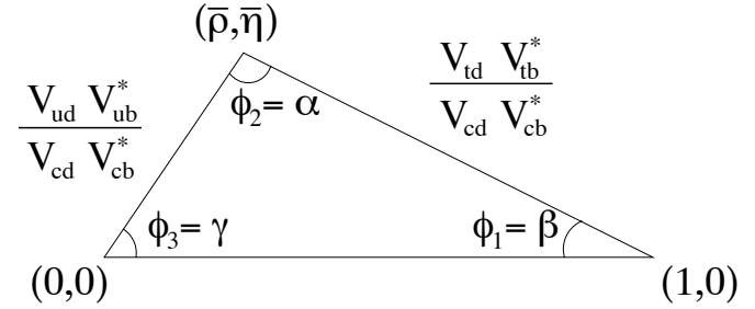
Figure 16.5.1. The Unitarity Triangle.
