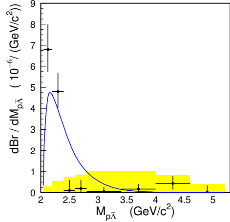
Figure 17.12.20. Differential branching fractions for B^- \rightarrow \Lambda \bar{p} \gamma as a function of baryon-antibaryon pair mass from Belle (Wang, 2007b). The shaded distribution shows the expectation from a phase-space MC simulation. The theoretical prediction from Geng and Hsiao (2005) is overlaid as a solid line for comparison. The area of the shaded distributions and areas under the theoretical curves are scaled to match the measured branching fractions from data. The uncertainties are statistical only.
