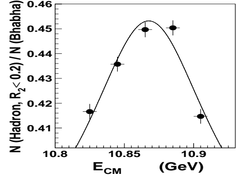
Figure 23.2.2. The ratio of the number of hadronic events ( R_2 < 0.2 ) to the number of Bhabha events as a function of the e^+e^- CM energy, from Drutskoy (2007a). Only statistical errors are shown. The curve is the result of the fit to a sum of a Breit-Wigner function and a constant.
