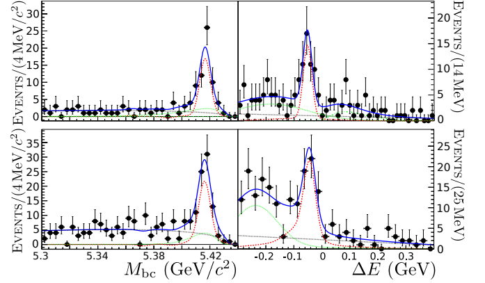
Figure 23.3.4. Left (right): M_{bc} = m_{ES} ( \Delta E ) distributions for B_s^0 \rightarrow D_s^- \pi^+ (top) and B_s^0 \rightarrow D_s^- \rho^+ (bottom) candidates with \Delta E ( m_{ES} ) restricted to the \pm 2.5\sigma B_s^{*0} \bar{B}_s^{*0} signal region. The blue solid curve is the total fitted p.d.f. , while the green (black) dotted curve is the peaking (continuum) background and the red dashed curve is the signal. Plots are from Louvot (2010).
