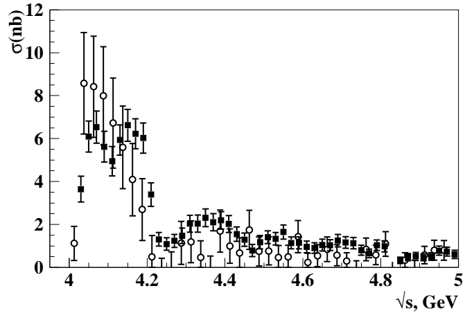
Figure 21.4.5. The exclusive cross sections for e^+e^- \rightarrow D^{*+}D^{*-} measured by Belle (Abe, 2007d; solid squares) and e^+e^- \rightarrow D^*D^* measured by BABAR (Aubert, 2009n; open circles).
