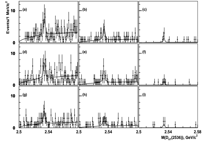
Figure 19.3.23. From (Aushev, 2011): The D_{s1}(2536)^+ mass distributions for: B^+ \rightarrow \bar{D}^0 D_{s1}(2536)^+ (a,b,c), B^0 \rightarrow D^- D_{s1}(2536)^+ (d,e,f), B^0 \rightarrow D^{*-} D_{s1}(2536)^+ (g,h,i) decays followed by the D_{s1}(2536)^+ decays to: D^{*0}K^+ with D^{*0} \rightarrow D^0\gamma (a,d,g); D^{*0}K^+ with D^{*0} \rightarrow D^0\pi^0 (b,e,h) and D^{*+}K_S^0 with D^{*+} \rightarrow D^0\pi^+ (c,f,i). The curves show results of the simultaneous fit.
