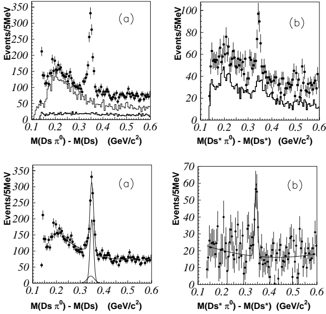
Figure 19.3.15. From (Abe, 2004a): Distributions of \Delta M(D_s^+ \pi^0) (left) and \Delta M(D_s^{*+} \pi^0) (right). In the upper plots data from mass sidebands are also shown: the D_s^+ (left) and D_s^{*+} (right) sideband regions (solid lines), \pi^0 sidebands (dashed). The bottom plots show fits to the \Delta M(D_s^+ \pi^0) (left) and \Delta M(D_s^{*+} \pi^0) distributions after subtraction of the D_s^{*+} sidebands.
