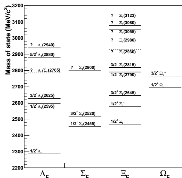
Figure 19.4.1. Summary of the known charmed baryon states. The spin-parity J^P is given, or marked “?” if not known. States whose existence is unclear (one-star rating in PDG) are marked with a dashed line.
