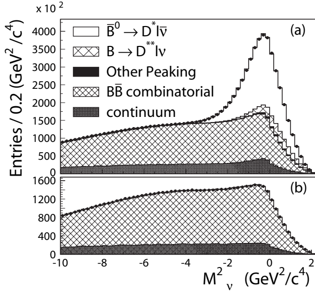
Figure 19.1.2. From (Aubert, 2008p). The M_\nu^2 distribution of the inclusive sample, for right-charge (a) and wrong-charge (b) samples. The data are represented by solid points with uncertainty. The MC fit results are overlaid on the data, as explained in the figure.
