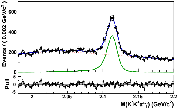
Figure 19.1.5. From (Zupanc, 2013b). M(K^+K^-\pi^+\gamma) mass distribution of exclusively reconstructed D_s^+ \rightarrow K^+K^-\pi^+\gamma decays within the inclusive D_s sample, with the fit result superimposed and including fitted signal contribution (solid green line), reflection from D_s^+ \rightarrow D_s\pi^0 \rightarrow K^+K^-\pi^+\gamma\gamma with one of the photons missing (full dark gray histogram) and combinatorial background (dashed red line).
