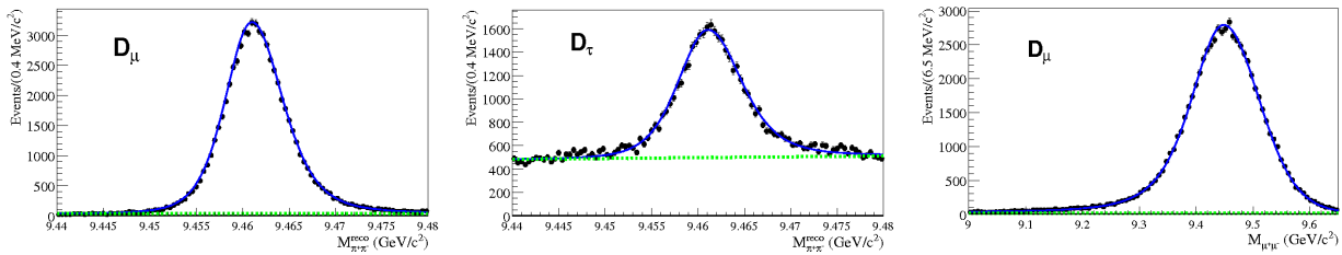
Figure 18.4.28. The recoil mass distribution for the dimuon (left) and di-tau (center) final states, and the dilepton mass for the dimuon final state (del Amo Sanchez, 2010r).
