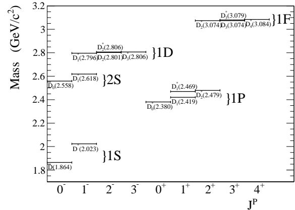
Figure 19.3.1. Modified Godfrey-Isgur predictions (Godfrey and Isgur, 1985). The plot shows the c\bar{u} spectrum where the masses have been scaled down so that the ground state matches the D^0 mass. Also, the 2^- states, not shown in the original paper, have been inserted following the splitting structure of the 1P states.
