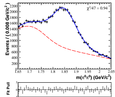
Figure 19.1.45. From (Lees, 2012u). The \pi^0\pi^0 mass distribution for D^0 \rightarrow \pi^0\pi^0 candidates in data (data points). The curves show the result of the unbinned maximum likelihood fit to the measured mass distribution. The solid (blue) line shows the result of the fit. The long-dashed (red) curve corresponds to the combinatoric background component. The \chi^2 value is determined from binned data and is provided as a goodness-of-fit measure. The pull distribution shows differences between the data and the solid blue curve with values and errors normalized to the Poisson error.
