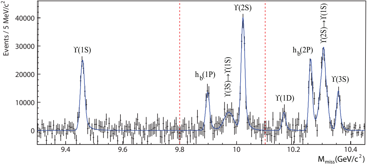
Figure 18.4.9. The spectrum of recoil mass M_{\text{miss}} \equiv M_{\text{recoil}}(\pi^+\pi^-) , used by the Belle Collaboration (Adachi, 2012a) to search for \Upsilon(5S) \rightarrow \pi^+\pi^- h_b(nP) , shown after subtracting the smooth combinatoric background (black points).
