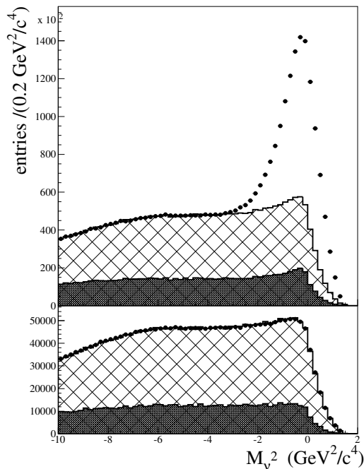
Figure 7.3.3. M_\nu^2 distribution for right-charge, \ell^\pm\pi_s^\mp , (top) and wrong-charge, \ell^\pm\pi_s^\pm , (bottom) events. The points correspond to on resonance data. The distributions of continuum events (dark histogram), obtained from luminosity-rescaled off-resonance events, and B\bar{B} combinatorial background events (hatched area), obtained from the simulation, are overlaid. Monte Carlo events are normalized to the difference between on-resonance and rescaled off peak data in the region M_\nu^2 < -4.5 \text{ GeV}^2/c^4 (Aubert, 2006s).
