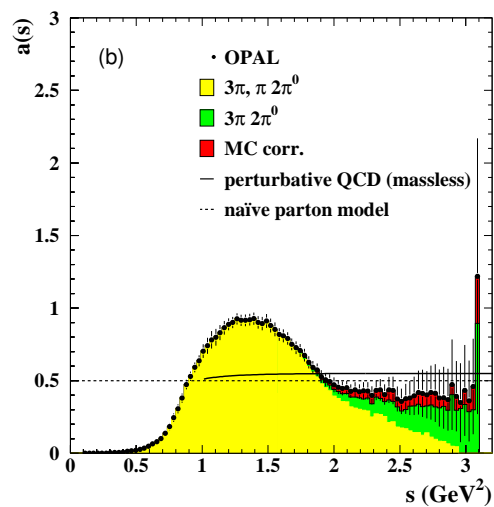
Figure 20.6.8. Axial Vector spectral functions measured by (a) ALEPH (Davier, Hoecker, and Zhang, 2006; Schael et al., 2005) and (b) OPAL (Ackerstaff et al., 1999) experiments.
