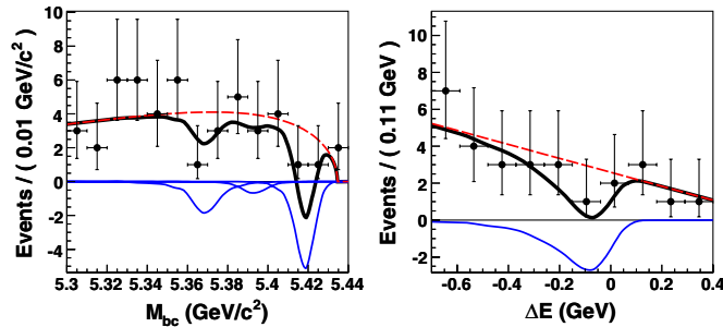
Figure 17.11.5. m_{\text{ES}} (left; called M_{bc} on the plot) and \Delta E (right) data yield (points) and fit results for B_s^0 \rightarrow \gamma\gamma in the Belle analysis (Wicht, 2008). The solid black curve represents the overall fit, while the dashed red and solid blue curves represent the continuum/combinatorial background and signal components of the fit, respectively. See Chapter 23 for an explanation of the structure of the m_{\text{ES}} distribution. On the \Delta E projection, m_{\text{ES}} > 5.4 \text{ GeV}/c^2 is required to select only the B_s^* \bar{B}_s^* contributions from \Upsilon(5S) . The fit returns a slight negative yield, consistent with zero within the data statistical uncertainties.
