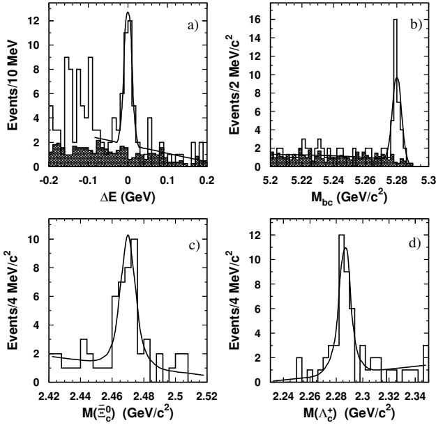
Figure 17.12.4. The \Delta E (a) and m_{\text{ES}} = M_{bc} (b) distributions for the B^+ \rightarrow \Xi_c^0 \Lambda_c^+ candidates from Belle (Chistov, 2006a). The hatched histograms show the combined \Xi_c^0 and \Lambda_c^+ mass sidebands normalized to the signal region. Also shown are the \Xi_c^0 (c) and \Lambda_c^+ (d) mass distributions for the B^+ \rightarrow \Xi_c^0 \Lambda_c^+ candidates taken from the B signal region of |\Delta E| < 0.025 GeV and m_{\text{ES}} > 5.272 GeV/ c^2 . For the \Xi_c^0 ( \Lambda_c^+ ) distribution \Lambda_c^+ ( \Xi_c^0 ) is required to be within \pm 15 MeV/ c^2 of the nominal mass. The overlaid curves are the fit results.
