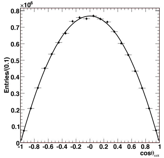
Figure 20.6.10. Distribution of \cos \theta_{\omega\pi} from \tau \rightarrow \omega(782)\pi^- \nu_\tau events in BABAR (Aubert, 2009ap). Here \theta_{\omega\pi} is the angle, in the \omega\pi^- rest frame, between the normal to the \omega \rightarrow \pi^+\pi^-\pi^0 decay plane and the direction of the pion. The curve shows a fit to determine the relative contributions from first-class and second-class currents.
