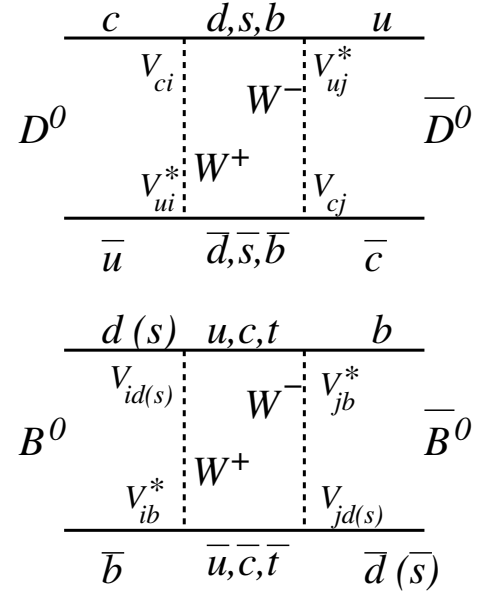
Figure 10.1.1. Box diagrams corresponding to the short-distance contributions to neutral meson mixing for (top) D and (bottom) B_{d,s}^0 mesons. Each of these contributions is matched by a diagram where the quark triplet, and W bosons are interchanged. The V_{ij} are CKM matrix elements discussed in Chapter 16.
