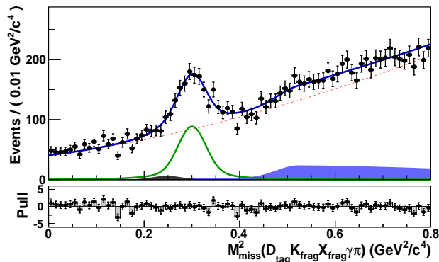
Figure 19.1.7. From (Zupanc, 2013b). M^2_{miss}(D_{tag} K X_{frag} \gamma \pi) distribution of partially reconstructed D_s^+ \rightarrow \eta \pi^+ decays within the inclusive D_s sample. The fit result is superimposed and includes fitted signal contribution (solid green line), reflections from charged pion originating from D_s^+ \rightarrow K^0 \pi^+ (full grey histograms) and other true D_s decays ( D_s^+ \rightarrow \rho K^+ \rightarrow \pi^+ \pi^- K^+ and D_s^+ \rightarrow \bar{K}^0 K^+ due to K - \pi mis-reconstruction) (full blue histogram), and combinatorial background (dashed red line).
