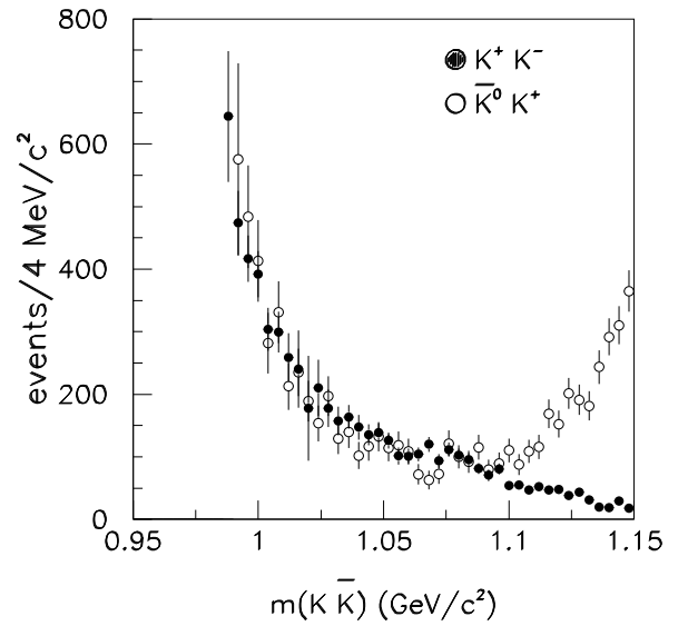
Figure 19.1.20. (Aubert, 2005f). Comparison between the phase-space-corrected K^+K^- and \bar{K}^0 K^+ normalised to the same area in the mass region between 0.992 and 1.05 \text{GeV}/c^2 .
