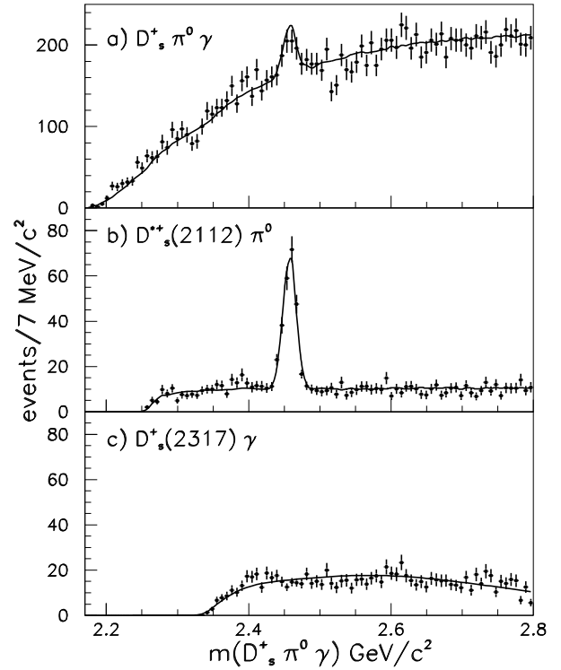
Figure 19.3.16. From (Aubert, 2004t). Maximum likelihood fit results overlaid on the D_s^+ \pi^0 \gamma mass distribution with a) no weights and after applying weights corresponding to b) the D_s^{*+} \pi^0 and c) the D_{s0}^*(2317)^+ \gamma decays.
