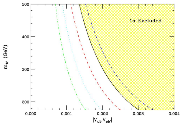
Figure 19.2.6. Contours of x in the fourth generation b' quark mass and CKM elements ( |V_{ub'}V_{cb'}| ) plane (see text for explanation). Contours are shown for x = [15.0, 11.7, 8.0, 5.0, 3.0] \times 10^{-3} (from right to left). From (Golowich, Hewett, Pakvasa, and Petrov, 2007).
