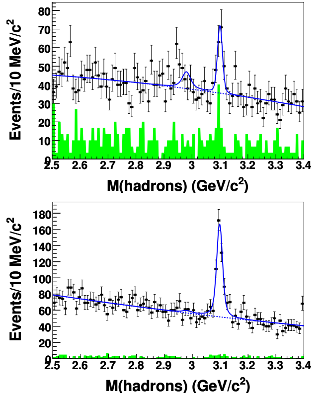
Figure 18.4.19. The mass distributions for a sum of the five \eta_c decay modes (top) from \Upsilon(1S) (Shen, 2010b) and (bottom) \Upsilon(2S) (Wang, 2011) data, respectively. The solid curve is a sum of the corresponding functions obtained from a simultaneous fit to all the \eta_c decay modes, and the dashed curve is a sum of the background functions from the fit. The shaded histogram is a sum of the continuum events (not normalized in \Upsilon(2S) data). The J/\psi signal is produced via ISR rather than from a radiative decay of an \Upsilon(nS) resonance.
