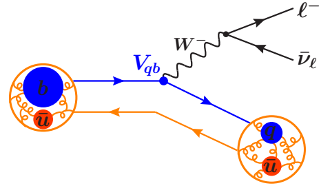
Figure 17.1.1. Illustration of semileptonic decay B^- \rightarrow X \ell^- \bar{\nu}_\ell .
