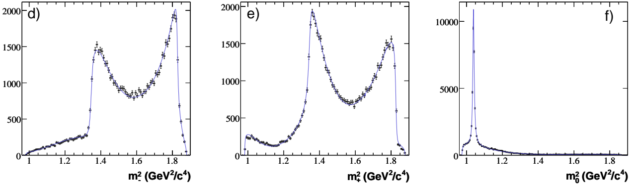
Figure 19.1.21. From (Aubert, 20081). D^0 \rightarrow K_S^0 K^+ K^- Dalitz plot projections from D^{*+} \rightarrow D^0 \pi^+ events on (d) m_-^2 , (e) m_+^2 , and (f) m_0^2 . The curves are the reference model fit projections.
