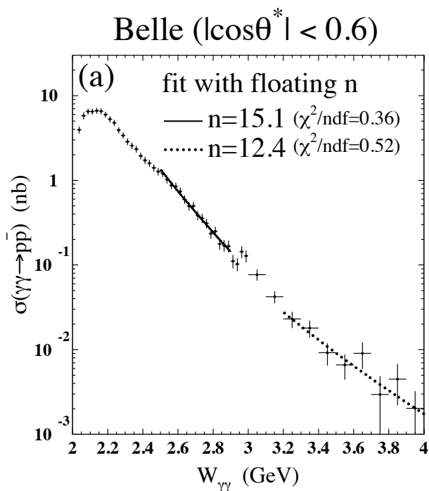
Figure 22.5.1. Cross section for \gamma\gamma \rightarrow p\bar{p} . The solid and dotted lines show the results of separate fits with \sigma \propto W^{-n} to the data in the range of W = 2.5 - 2.9 \text{ GeV} and 3.2 - 4.0 \text{ GeV} , respectively. The error bars include statistical and systematic errors. The \chi^2/\text{ndf} values for each fit are indicated in the figure. From (Kuo, 2005).
