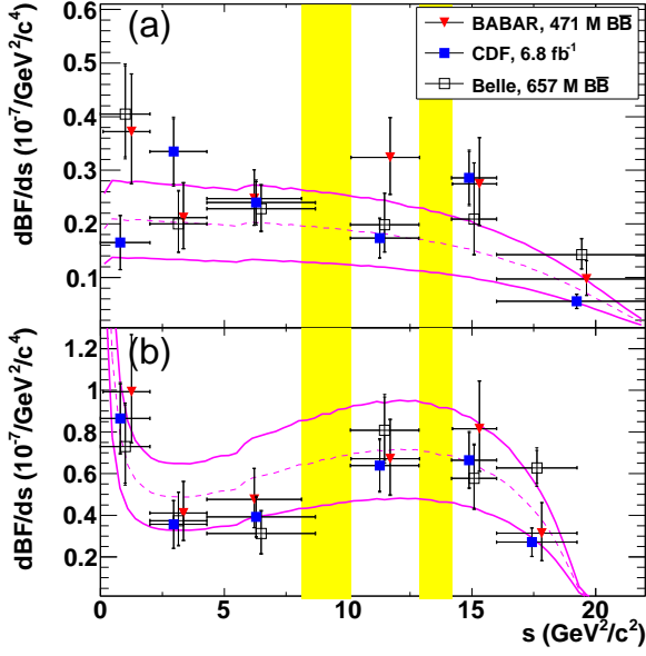
Figure 17.9.12. From (Lees, 2012i). Branching fractions d\mathcal{B}/dq^2 for (a) B \rightarrow K\ell^+\ell^- and (b) B \rightarrow K^*\ell^+\ell^- from Belle, CDF and BABAR vs. s \equiv q^2 . The yellow bands correspond to the J/\psi and \psi' veto windows used by BABAR . The magenta curves show the range of the SM predictions from (Ali, Lunghi, Greub, and Hiller, 2002).
