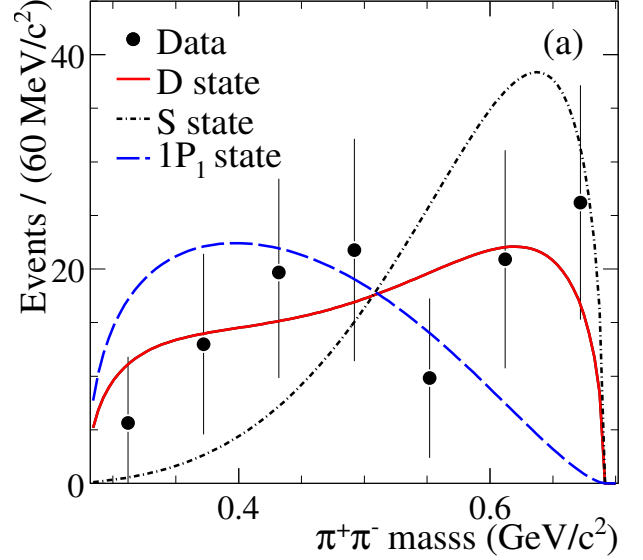
Figure 18.4.12. The dipion mass spectrum for the background-subtracted data in the region 10.155 < m_{\pi^+\pi^-\ell^+\ell^-} < 10.68 \text{ GeV}/c^2 . The shapes expected from S -wave, D -wave, and 1P_1 states are shown (del Amo Sanchez, 2010k).
