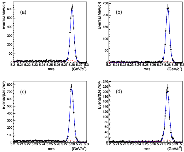
Figure 17.3.4. The m_{ES} distributions for (a) B^0 \rightarrow D^- \pi^+ , (b) B^0 \rightarrow D^{*-} \pi^+ , (c) B^+ \rightarrow D^0 \pi^+ , and (d) B^+ \rightarrow D^{*0} \pi^+ (from Aubert, 2007g). In the figures the solid line is the fit to the data while the background component (including peaking background) is shown as a dashed line.
