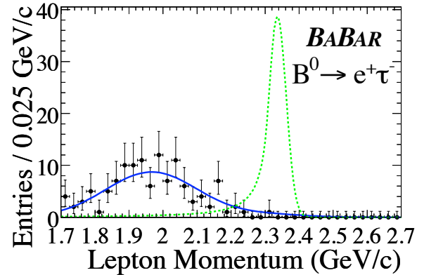
Figure 17.11.7. Signal electron candidate momentum in the signal B rest frame for B^0 \rightarrow \tau^\pm e^\mp (Aubert, 2008az). The points with errors are BABAR data, the solid blue curve is the fitted background p.d.f. and the dashed green curve shows the expected signal shape.
