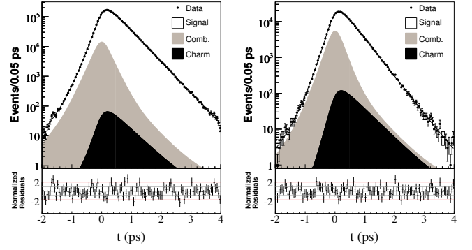
Figure 19.2.16. From (Aubert, 2009v). BABAR results of the simultaneous fit to decay time distributions of untagged samples: D^0 \rightarrow K^-\pi^+ (left) and D^0 \rightarrow K^+K^- (right).
