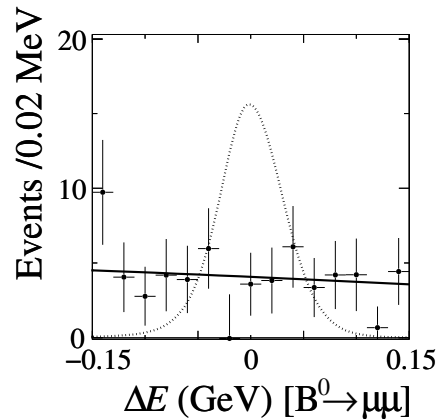
Figure 17.11.2. \Delta E distribution of selected B^0 \rightarrow \mu^+ \mu^- candidates (Aubert, 2008as). The solid curve is the background sPlot (see Section 11.2.3) and the dashed curve is the expected distribution of signal with an arbitrary normalization.
