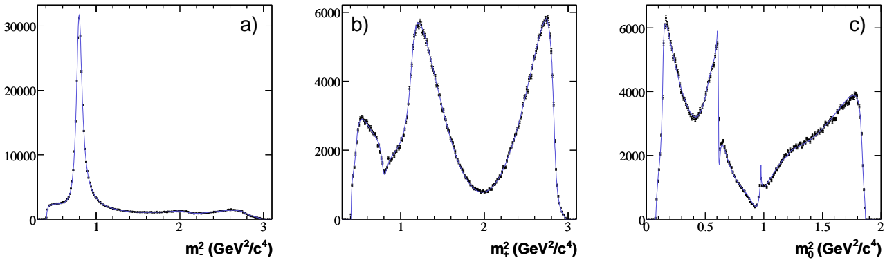
Figure 19.1.22. From (Aubert, 20081). D^0 \rightarrow K_S^0 \pi^+ \pi^- Dalitz plot projections from D^{*+} \rightarrow D^0 \pi^+ events on (a) m_-^2 , (b) m_+^2 , and (c) m_0^2 . The curves are the reference model fit projections.
