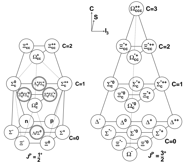
Figure 19.4.3. The SU(4) multiplets containing the ground state baryons, arranged by spin-parity ( J^P ), isospin projection ( I_3 ), strangeness ( S ), and charm ( C ). A double ring indicates that two states have the same J^P, I_3, S, and C quantum numbers.
