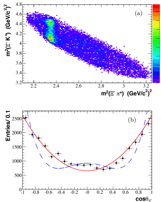
Figure 19.4.15. \Lambda_c^+ \rightarrow \Xi^- \pi^+ K^+ events at BABAR , showing (a) the Dalitz plot, and (b) the angular distribution in the \Xi(1530) region. Curves are superimposed for the \Xi(1530) spin hypotheses J = 3/2 (solid, p-value 3 \times 10^{-4} ) and J = 5/2 (dashed, p-value 6 \times 10^{-44} ). The hypothesis J = 1/2 would correspond to a flat distribution. Color online. (Aubert, 2008w)
