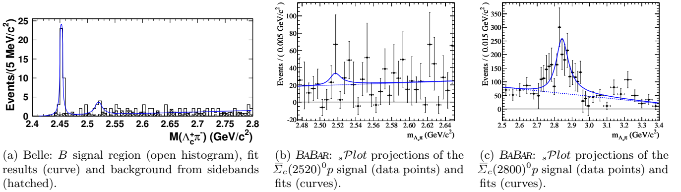
Figure 17.12.3. m(\Lambda_c^+ \pi^-) distributions from (a) Belle (Gabyshev, 2006), and (b,c) BABAR (Aubert, 2008aa); for the s Plot technique, see Section 11.2.3. Three \Sigma_c resonances are visible at 2.455 GeV/ c^2 (a), 2.52 GeV/ c^2 (a and b, not significant) and 2.80 GeV/ c^2 (c).
