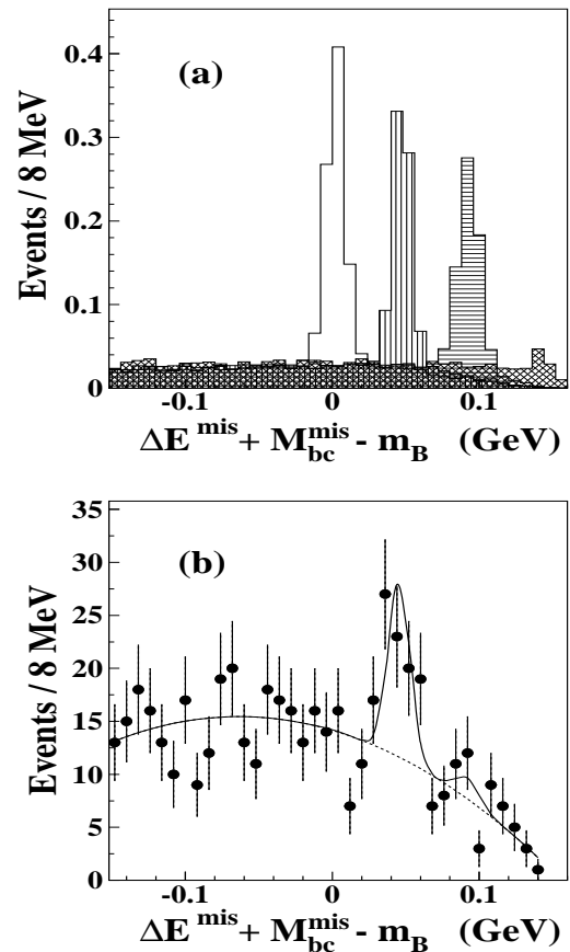
Figure 23.2.6. (a) The \Delta X = \Delta E^{\text{mis}} + m_{ES}^{\text{mis}} - m_B distribution normalized to unity for MC simulated B^+ \rightarrow J/\psi K^+ decays in the (peaks from left to right) B\bar{B}\pi^+ , B\bar{B}^*\pi^+ + B^*\bar{B}\pi^+ , B^*\bar{B}^*\pi^+ , and B\bar{B}\pi\pi channels. (b) The \Delta X = \Delta E^{\text{mis}} + m_{ES}^{\text{mis}} - m_B data distribution for right-sign B^{-/0}\pi^+ combinations for the sum of the five studied B modes. Plots are from Drutskoy (2010).
