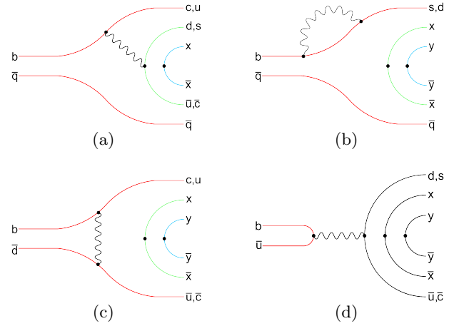
Figure 17.12.5. Quark diagrams for two-body baryonic B decay \bar{B} \rightarrow \mathfrak{B}_1 \mathfrak{B}_2 . The wavy line represents a W , while gluon lines are omitted. Quark antiquark pairs from the vacuum are denoted as x, y and determine the flavor of the two final baryons. In this and subsequent figures, the colors of the quark lines are significant: see the discussion in Section 17.12.2.2.
