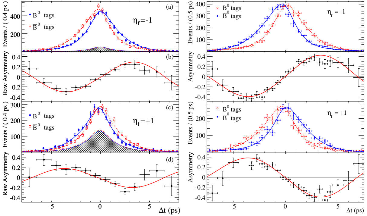
Figure 17.6.7. Flavor-tagged \Delta t distributions (a,c) and raw CP asymmetries (b,d) for the BABAR (left, (Aubert, 2009z)) and Belle (right, (Adachi, 2012c)) measurements of \sin 2\phi_1 . The top two plots show the B \rightarrow (c\bar{c})K_s^0 ( \eta_f = -1 ) samples, and the bottom two show the B \rightarrow J/\psi K_L^0 ( \eta_f = +1 ) sample. The shaded regions for BABAR represent the fitted background, while the Belle distributions are background subtracted. The two experiments adopt the opposite color code in \Delta t distribution plots.
