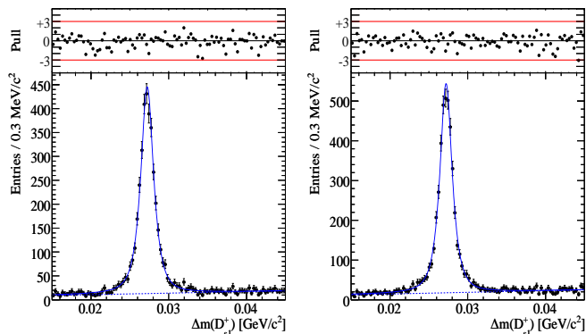
Figure 19.3.24. From (Lees, 2011d). \Delta m(D_{s1}(2536)^+) distribution for (left) the D^0 \rightarrow K^-\pi^+ and (right) the D^0 \rightarrow K^-\pi^+\pi^+\pi^- decay modes. The solid line is the fit function as described in the text, the dotted line indicates the background contribution. The normalized fit residuals are shown on top.
