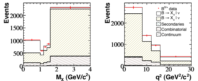
Figure 17.1.19. Belle (Urquijo, 2010): Projections of measured distributions (data points) of (a) m_X and (b) q^2 with varying bin size, compared to results of a two-dimensional m_X - q^2 distribution for the sum of scaled MC contributions. The data are not efficiency corrected.
