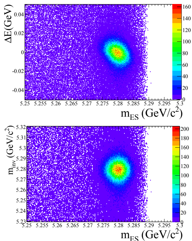
Figure 7.1.4. Distributions from \bar{B}^0 \rightarrow \Lambda_c^+ \bar{p} \pi^+ \pi^- events (Monte Carlo). The top plot is for \Delta E vs m_{ES} showing a strong correlation, and the bottom is for the invariant mass m_B vs m_{ES} which is only weakly correlated through measurement errors. BABAR internal, from the Lees (2013h) analysis.
