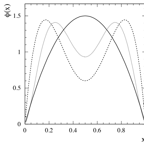
Figure 22.7.2. The pion distribution amplitudes at Q^2 = 5.76 \text{ GeV}^2 for three models: asymptotic (Lepage and Brodsky, 1979a) [solid line], Chernyak and Zhitnitsky (1982) [dashed line], and Bakulev, Mikhailov, and Stefanis (2001) [dotted line].
