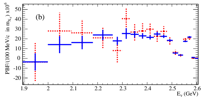
Figure 17.9.6. From (Lees, 2012f). Photon spectrum in the B rest frame from BABAR 's sum of exclusive final states analysis (blue solid lines), compared to the results from the older (super-seeded) similar BABAR analysis (red dashed lines). The bin widths are defined in terms of the X_s mass, and converted to E_\gamma using Eq. (17.9.22). The peak at 2.56 GeV is from exclusive B \rightarrow K^*\gamma decays.
