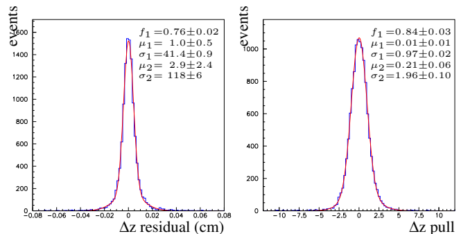
Figure 6.3.1. Residual (left) and pull (right) of the decay vertex z position of reconstructed B^0 \rightarrow J/\psi K_s^0 candidates in a BABAR simulated data sample. Fits to a double Gaussian are superimposed.
