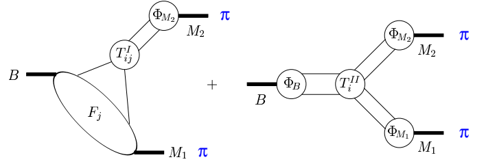
Figure 17.4.2. Graphical representation of the factorization formula given Eq. 17.4.6 (Beneke, Buchalla, Neubert, and Sachrajda, 2000).
