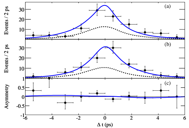
Figure 17.7.6. The \Delta t distributions of events enriched in signal for (a) B^0 and (b) \bar{B}^0 tagged B \rightarrow \rho^+\rho^- events. The solid lines are the sum of signal and backgrounds and the dashed lines are the sum of backgrounds. The time-dependent CP asymmetry is presented in (c). (As there is no entry in the second bin from the left in (b), the corresponding point is at 1 in (c).) The curve corresponds to the measured asymmetry (from Aubert (2007b)).
