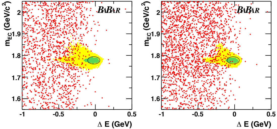
Figure 20.4.2. The 2\sigma elliptical signal-box for \tau^\pm \rightarrow e^\pm \gamma (Left) and \tau^\pm \rightarrow \mu^\pm \gamma (Right) decays in the m_{\text{EC}} vs. \Delta E plane in the BABAR analysis. m_{\text{EC}} is the invariant mass of the lepton-photon pair as discussed in the text. Data are shown as red dots and contours containing 90% (50%) of signal MC events are shown as the yellow (green) shaded regions (Aubert, 2010i).
