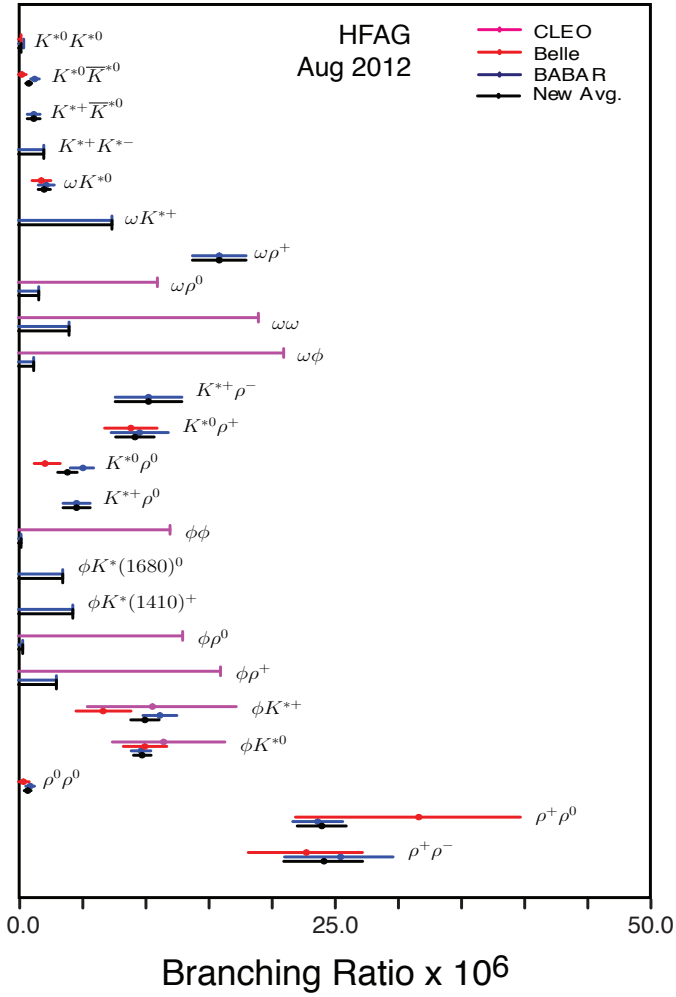
Figure 17.4.9. Summary of branching fraction measurements ( \times 10^{-6} ) and HFAG averages for Vector-Vector (VV) decays (Amhis et al. (2012)).
