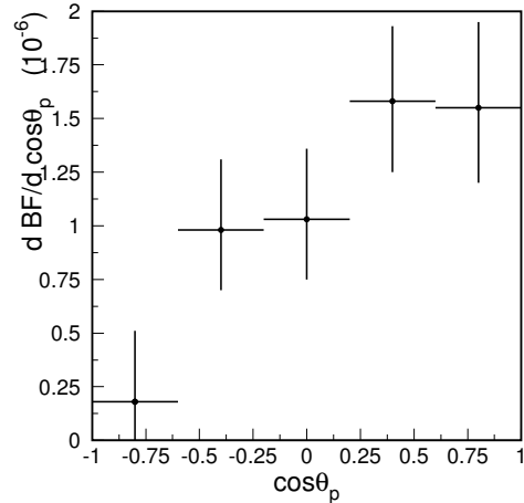
Figure 17.12.21. Differential branching fractions vs \cos \theta_p for B^- \rightarrow \Lambda \bar{p} \gamma in the region near threshold (baryon-antibaryon mass < 2.8 \text{ GeV}/c^2 ) from Belle (Wang, 2007b). The uncertainties are statistical only.
