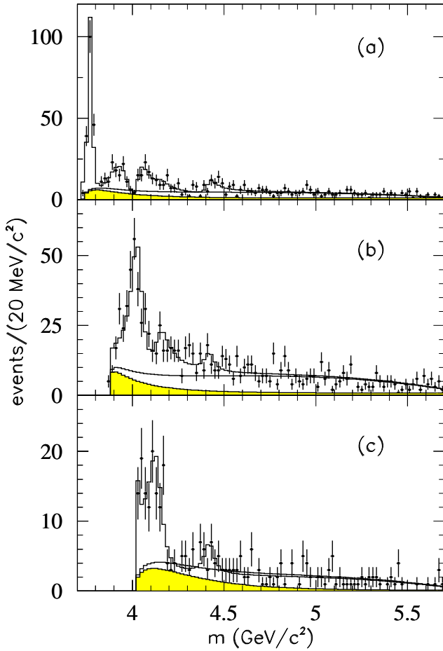
Figure 18.2.11. From Aubert (2009n): The (a) DD\bar{D} , (b) DD^*\bar{D}^* , and (c) D^*D^*\bar{D}^* mass spectra in the e^+e^- \rightarrow \gamma_{\text{ISR}} D^{(*)}\bar{D}^{(*)} process. The curves represent the fitted functions as described in the text. The shaded histogram corresponds to the smoothed incoherent background. The second smooth solid line represents the non-resonant contribution.
