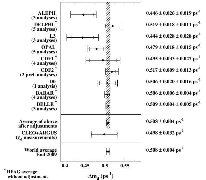
Figure 17.5.6. The B^0\bar{B}^0 oscillation frequency \Delta m_d as measured by the different experiments along with their average. Averages are also given separately for the time-dependent measurements by the B Factories and the LEP and Tevatron experiments, and the time-integrated measurements by CLEO and ARGUS (Asner et al., 2010).
