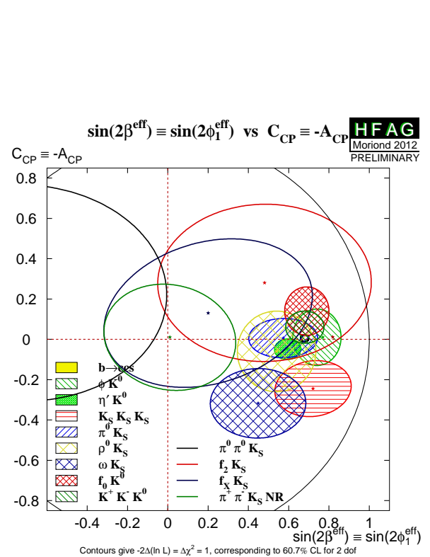
Figure 17.6.14. Summary of C vs. \sin 2\phi_1^{\text{eff}} measurements from charmless B^0 decays (Amhis et al., 2012).
