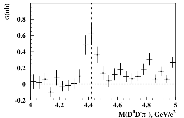
Figure 21.4.8. The exclusive cross section for e^+e^- \rightarrow D^0 D^- \pi^+ measured by Belle (Pakhlova, 2008c). The dotted line corresponds to the mass of the \psi(4415) .
