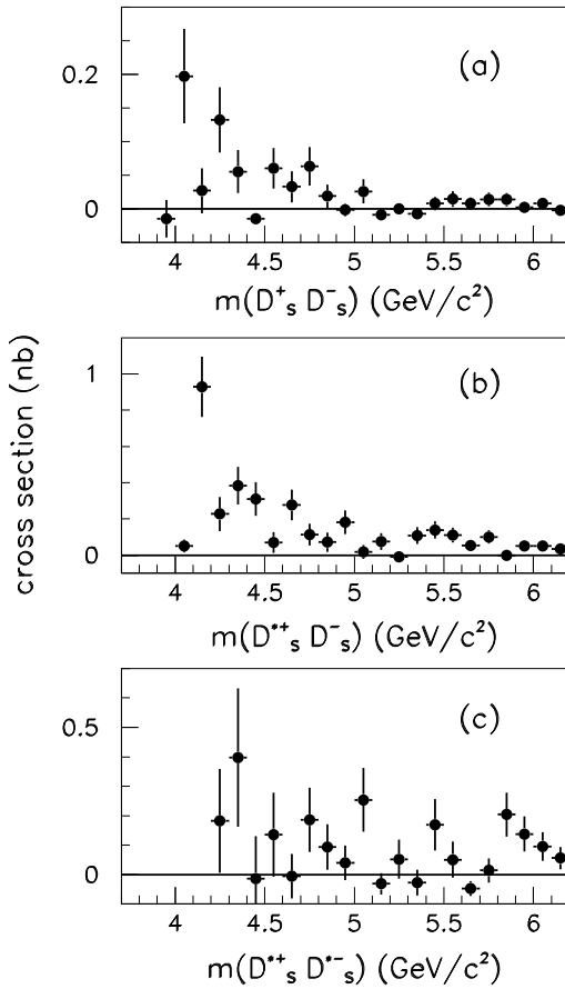
Figure 21.4.6. Exclusive cross sections for (a) e^+e^- \rightarrow D_s^+ D_s^- , (b) e^+e^- \rightarrow D_s^+ D_s^{*-} (and charge conjugate), and (c) e^+e^- \rightarrow D_s^{*+} D_s^{*-} , from BABAR data (del Amo Sanchez, 2010d). The error bars correspond to statistical errors only.
