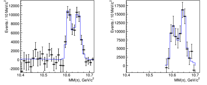
Figure 18.4.15. The (a) h_b(1P) and (b) h_b(2P) yields as a function of M_{\text{recoil}}(\pi) (points with error bars) and results of the fit (histogram). From (Bondar, 2012).
