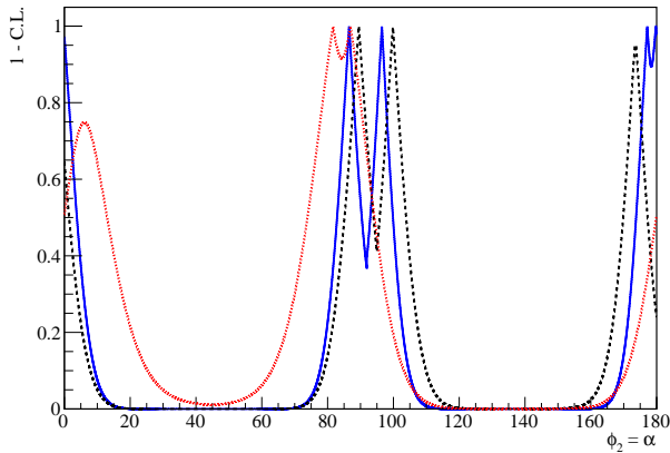
Figure 17.7.10. The 1 - C.L. function obtained on \phi_2 = \alpha from the B Factories (solid blue) using B^0 \rightarrow \rho^+\rho^- , and B^+ \rightarrow K^{*0}\rho^+ decays and the BGRS method discussed in the text. The constraints from BABAR (dashed black) and Belle (dotted red) are also shown. The curves shown include solutions for all possible values of \delta_{PT} .
