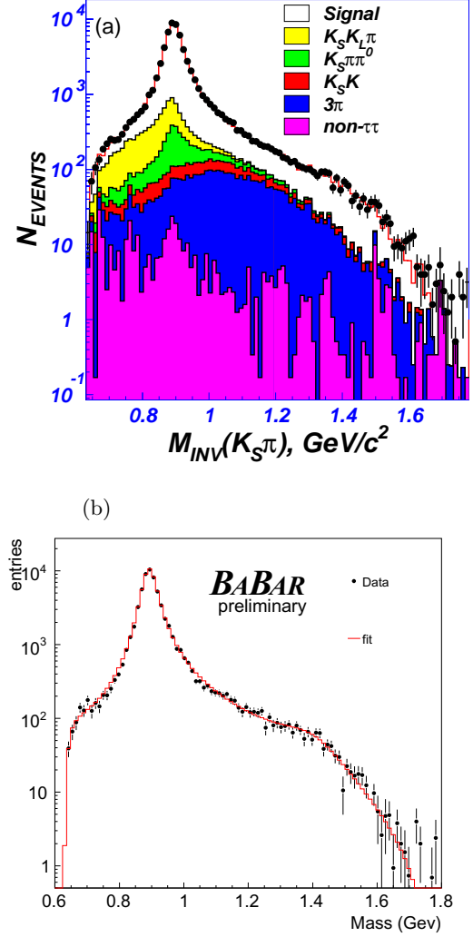
Figure 20.6.5. K_S\pi^- mass distribution measured by (a) Belle (Epifanov, 2007) and by (b) BABAR (Adametz, 2011). Points with error bars in both figures are data, the histogram shows the fitted result for the spectrum expected in the model incorporating the K^*(892) + K_0^*(800) + K^*(1410) model. In Belle data, different types of background are also shown, while in the BABAR plot, the background is already subtracted.
