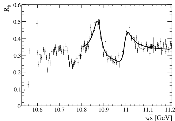
Figure 23.1.1. Measured ratio of hadronic to e^+e^- \rightarrow \mu^+\mu^- cross-sections, R_b , as a function of the CM energy, from an energy scan performed by the BABAR collaboration (Aubert, 2009x). The result of a fit to a function including background and \Upsilon(5S) and \Upsilon(6S) resonances is shown by the curve. The error bars represent the statistical and the uncorrelated systematic uncertainties added in quadrature.
