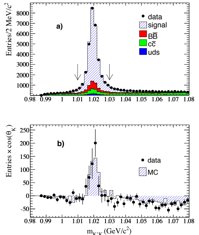
Figure 19.1.39. From (Aubert, 2008be). a) K^+ K^- invariant mass distribution from D_s^+ \rightarrow K^+ K^- e^+ \nu_e data and simulated events. MC events have been normalized to the data luminosity according to the different cross sections. The arrows indicate the selected K^+ K^- mass interval. In b), each event is weighted by the measured value of \cos \theta_K . Negative entries are produced by the c\bar{c} background asymmetry in \cos \theta_K .
