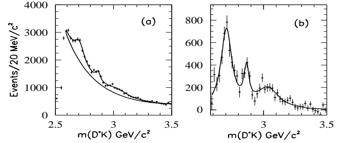
Figure 19.3.31. From (Aubert, 2009au). (a) Fit to the D^* K invariant mass spectrum, (b) residuals after subtraction of the fitted background.
