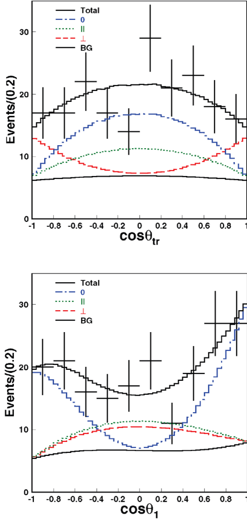
Figure 12.2.1. Angular distributions in the transversity frame for (top) \cos \theta_{tr} and (bottom) \cos \theta_1 , shown in the example of the B^0 \rightarrow D^{*+} D^{*-} analysis (Miyake, 2005). The points with error bars represent the data. The dot-dashed, dotted, and dashed lines correspond to the A_L , A_{\parallel} , and A_{\perp} amplitudes respectively. The lower solid line is the background (BG), while the upper solid line shows the sum of all contributions. The asymmetry in the \cos \theta_1 distribution is due to an inefficiency for low momentum track reconstruction.
