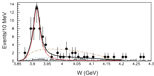
Figure 18.3.7. The J/\psi distribution in \gamma\gamma events as measured by Belle (Uehara, 2010b). The black curve is the result of a fit to the data to determine the Y(3915) mass and width. The dot-dashed curve (brown) represents the result of the fit without the resonant contribution.
