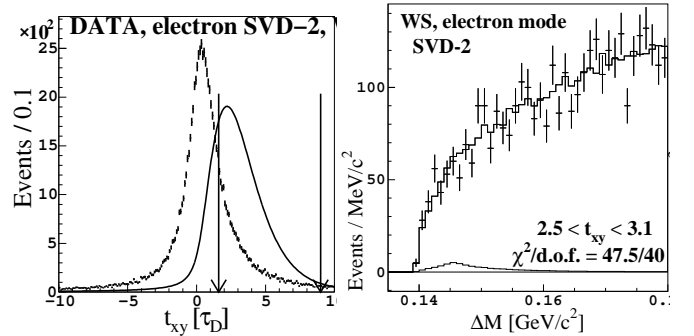
Figure 19.2.23. Left: The distribution of the decay time in the transverse plane for selected WS events (dots). The solid line shows the simulated distribution of signal events and the vertical arrows the interval selected for the signal. Right: An example of the fit to the \Delta M data distribution (points) in a single t_{xy} bin for the WS e-2 data subsample. The histogram is the fit to the distribution, with the contribution of signal shown along the horizontal axis. From (Bitenc, 2008).
