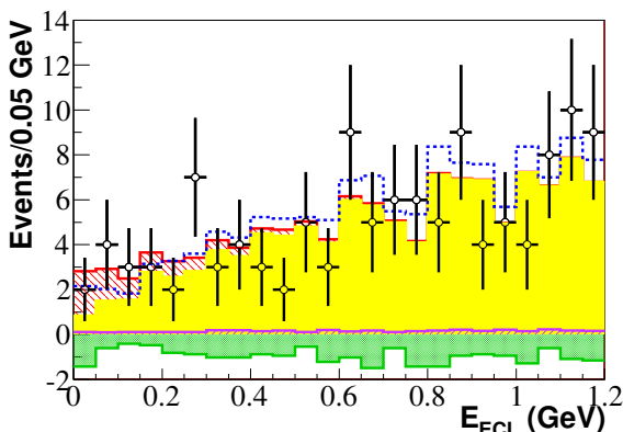
Figure 17.11.4. Distribution of E_{\text{extra}} in the BABAR search for B^0 \rightarrow invisible using semileptonic tagged events (Lees, 2012g). Lines represent the result of the fit. Distribution of a similar quantity (bottom, called E_{\text{ECL}} at Belle) for the search in the same decay mode using hadronic tagged events (Hsu, 2012). Lines are the result of the fit (lightly hatched yellow region is the background contribution and the solid red line the total).
