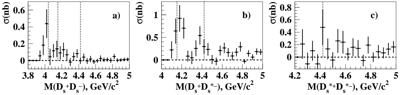
Figure 21.4.7. Exclusive cross sections for (a) e^+e^- \rightarrow D_s^+ D_s^- , (b) e^+e^- \rightarrow D_s^+ D_s^{*-} (and charge conjugate), and (c) e^+e^- \rightarrow D_s^{*+} D_s^{*-} , from Belle data (Pakhlova, 2011). Error bars show statistical uncertainties only. The dotted lines show the masses of the \psi(4040) , \psi(4160) and \psi(4415) states.
