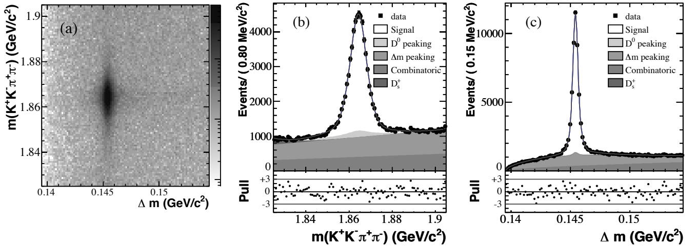
Figure 19.2.32. From (del Amo Sanchez, 2010n). The distribution of selected events in the m(K^+K^-\pi^+\pi^-) vs. \Delta m plane (a) is shown together with the projections of the events with overlaid the fit results for m(K^+K^-\pi^+\pi^-) (b) and \Delta m (c), with the shaded areas indicating the different contributions. In the bottom, the distribution of the normalized residuals (Pull), is shown for each fit projection.
