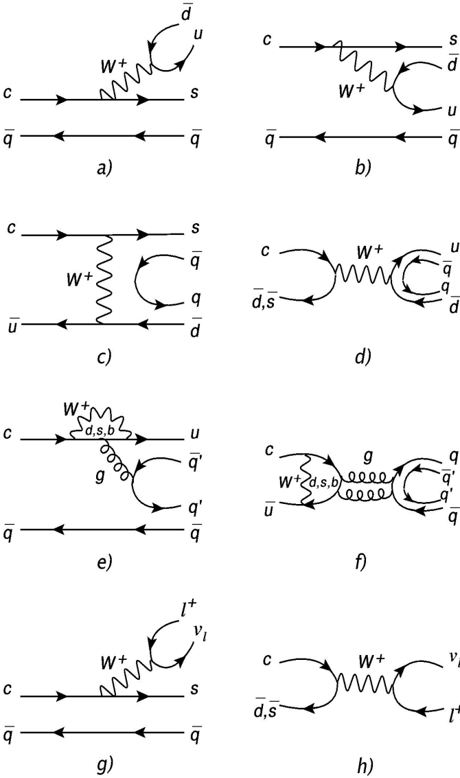
Figure 19.1.1. Quark diagrams for charm meson decays: hadronic (a-f), semileptonic (g), leptonic (h). Diagrams underlying hadronic decays: external W emission (a), internal W emission (b), W exchange (c), W annihilation (d), W -loop penguin (e) and W -loop penguin annihilation (f).
