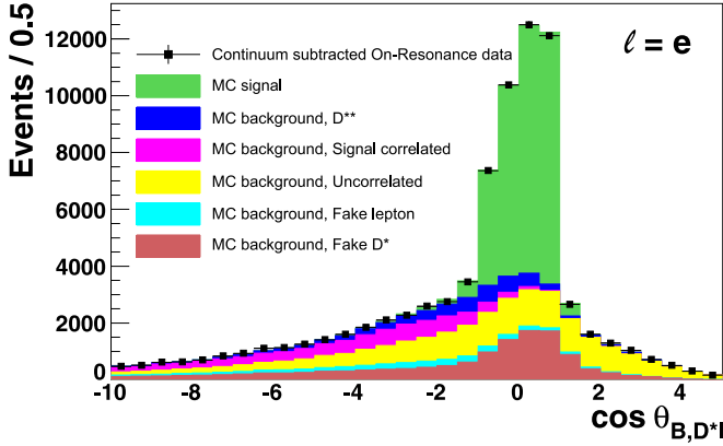
Figure 7.2.1. The \cos \theta_{B,D^* \ell} distribution for B^0 \rightarrow D^{*-} e^+ \nu_e decays (Dungel, 2010). The points with error bars are data and full histograms are, top to bottom, the signal component and different types of background. Signal decays are constrained to lie in the interval (-1, 1) , while background decays populate a much wider region.
