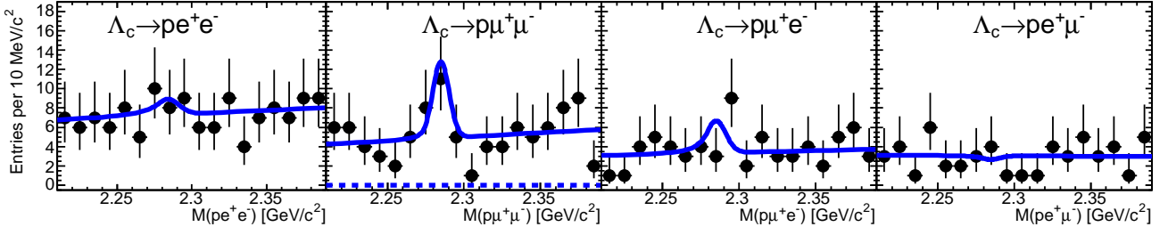
Figure 19.1.46. From (Lees, 2011k). Invariant-mass distributions for \Lambda_c^+ \rightarrow p \ell^+ \ell'^- candidates. The solid lines are the results of the fits. The background component for the dimuon mode in which muon candidates arise from hadrons misidentified is shown as a dashed curve.
