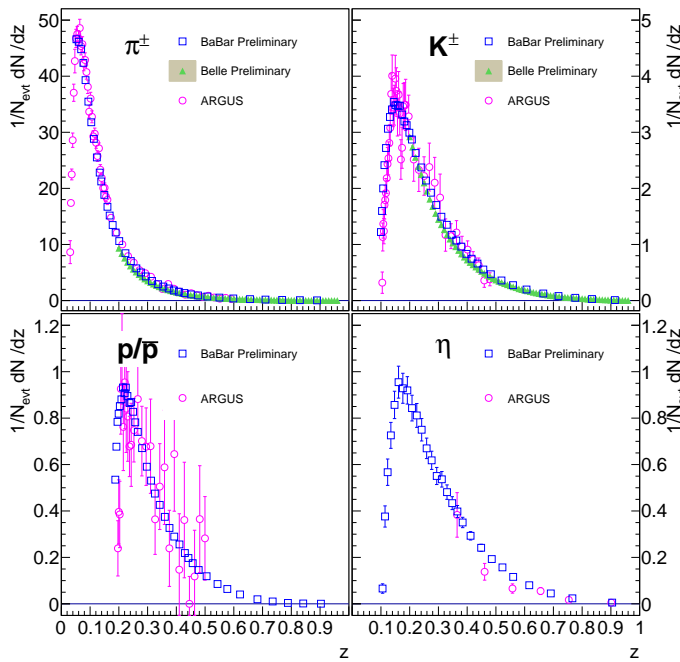
Figure 24.1.2. Comparison of the multiplicities for \pi^\pm , K^\pm , p/\bar{p} , and \eta , measured by BABAR at \sqrt{s} = 10.54 GeV (compiled from Muller, 2004 and Lees, 2013f), Belle at 10.52 GeV (compiled from Leitgab, 2012 and Leitgab, 2013), and ARGUS at 9.98 GeV (Albrecht et al., 1989a, 1990b).
