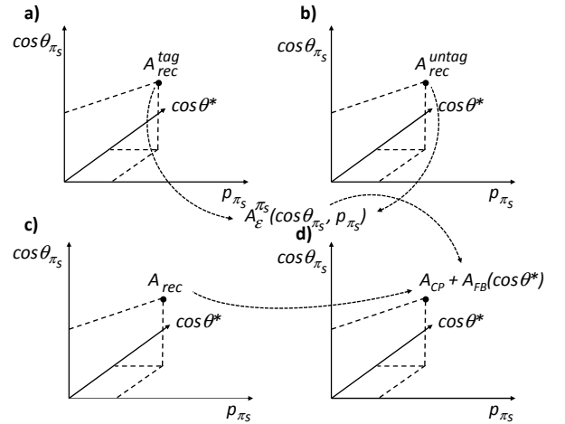
Figure 19.2.27. Graphical presentation of the method to correct the measurement of the CP asymmetry in D meson decays. In the case of D^0 \rightarrow h^+h^- the difference between the measured asymmetries for D^{*+} \rightarrow D^0(\rightarrow K^-\pi^+)\pi_s^+ (a) and D^0 \rightarrow K^-\pi^+ (b) decays in a given bin of \pi_s momentum, its polar angle \theta_{\pi_s} and the D meson polar angle in the CM system \theta^* , yields the detector induced asymmetry A_{\epsilon}^{\pi_s} . This can be used to correct the measured asymmetry for the decays D^{*+} \rightarrow D^0(\rightarrow h^-h^+)\pi_s^+ (c) resulting in the sum A_{CP} + A_{FB} (d). The latter can be distinguished according to their \cos\theta^* dependence.
