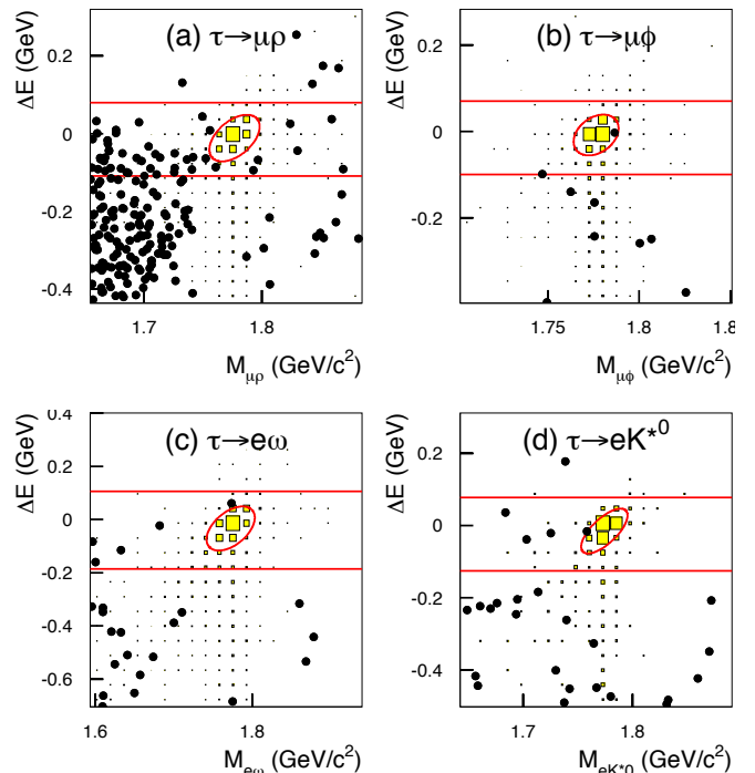
Figure 14.4.1. M_{\ell V} - \Delta E signal region (see text) for four typical lepton-number-violating decays: (a) \tau^- \rightarrow \mu^- \rho^0 (b) \tau^- \rightarrow \mu^- \phi (c) \tau^- \rightarrow e^- \omega , and (d) \tau^- \rightarrow e^- K^{*0} from Miyazaki (2011). Data points are shown as solid circles, and MC signal distributions are shown as yellow boxes (with arbitrary normalization). Red ellipses denote blinded regions, and horizontal lines denote the regions used for estimating background within the blinded ellipses.
