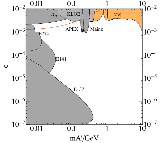
Figure 21.6.1. Adopted from (Bjorken, Essig, Schuster, and Toro, 2009). Constraints on the mixing strength, \epsilon , as a function of the dark photon mass. The red line shows the value of the coupling required to explain the discrepancy between the calculated and measured anomalous magnetic moment of the muon (Pospelov, 2009). The excluded regions obtained by reinterpreting the upper limits on the Y(2S, 3S) \rightarrow A^0\gamma , A^0 \rightarrow \ell^+\ell^- (Aubert, 2009an) branching fractions are shown as a yellow band.
