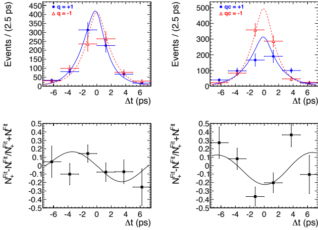
Figure 17.7.9. Background subtracted time-dependent fit results for B^0 \rightarrow a_1^\pm(1260)\pi^\mp (Dalseno, 2012). (a) and (b) show the \Delta t distributions for the B_{\text{tag}}^0 flavor q and the product of the B_{\text{tag}}^0 flavor and a_1 charge qc , respectively. The left plot shows the effect of flavor-dependent CP violation while the plot on the right shows the effects of the CP conserving parameters. The solid blue and dashed red curves represent the \Delta t distributions for q = +1 and q = -1 , respectively. (c) and (d) show the asymmetry of the plots immediately above them, (N_+^{\text{Fit}} - N_-^{\text{Fit}}) / (N_+^{\text{Fit}} + N_-^{\text{Fit}}) , where N_+^{\text{Fit}} ( N_-^{\text{Fit}} ) is the measured signal yield of positive (negative) quantities in bins of \Delta t . All curves are the expected ones for the values in Eqs (17.7.28) and (17.7.29).
