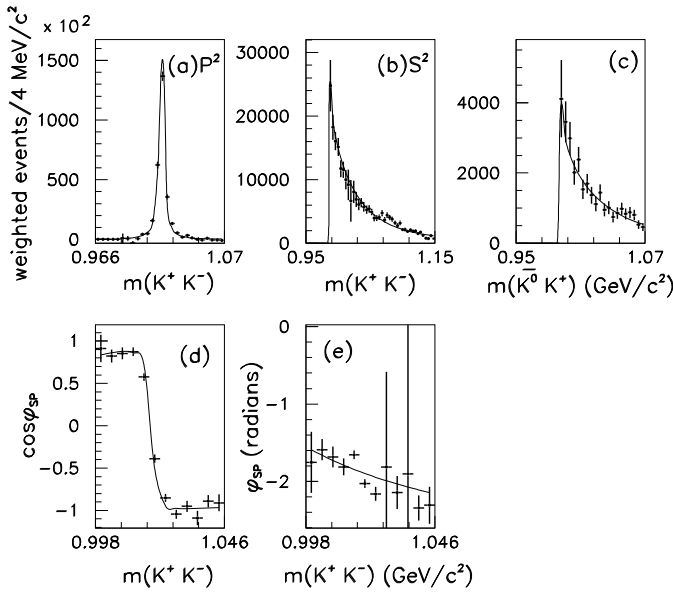
Figure 19.1.19. From (Aubert, 2005f). Results from the K^+K^- Partial Wave Analysis corrected for phase space. (a) P -wave strength, (b) S -wave strength. (c) m(\bar{K}^0 K^+) distribution, (d) \cos \phi_{SP} in the \phi(1020) region. (e) \phi_{SP} in the threshold region after having subtracted the fitted \phi(1020) phase motion shown in (d).
