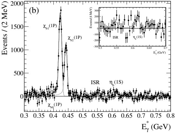
Figure 18.4.16. The converted-photon energy spectrum, after subtracting the smooth background (Lees, 2011m). These data were taken at the \Upsilon(2S) resonance.
