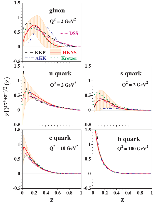
Figure 24.1.6. Determined fragmentation functions for the pion and their comparison with other parameterizations (Hirai, Kumano, Nagai, and Sudoh, 2007a,b). The shaded bands indicate estimated uncertainties of the HKNS.
