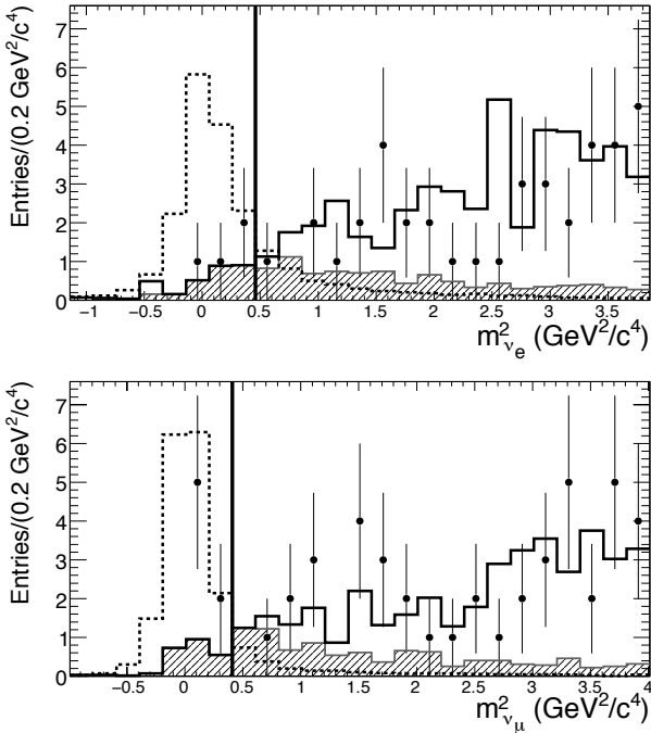
Figure 17.10.7. m_\nu^2 distribution in B^+ \rightarrow \ell^+ \nu_\ell \gamma , from Aubert (2009a), after all selection criteria are applied, in the electron (top) and muon (bottom) modes. The m_{ES} -peaking (shaded) and non-peaking (solid) background contributions are shown stacked, along with signal MC (dashed) normalized to \mathcal{B} = 40 \times 10^{-6} , and data (points). Events to the left of the vertical lines are selected.
