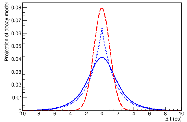
Figure 11.3.1. Visualization of exponential decay time difference distribution before (blue dashed) and after (blue solid) convolution with a Gaussian resolution function (red, long dashes).
