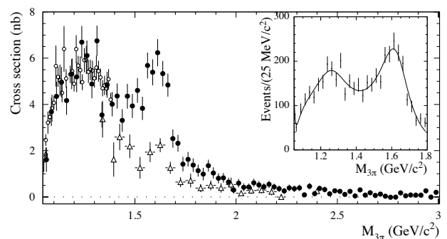
Figure 21.3.8. The e^+e^- \rightarrow \pi^+\pi^-\pi^0 cross section measured by the BABAR experiment (Aubert, 2004af; full circles) in the 1\text{--}3 \text{ GeV}/c^2 range compared with the SND (Achasov et al., 2002; open circles) and DM2 (Antonelli et al., 1992; triangles) data. The inset shows the result of a fit to the mass distribution as explained in the text.
