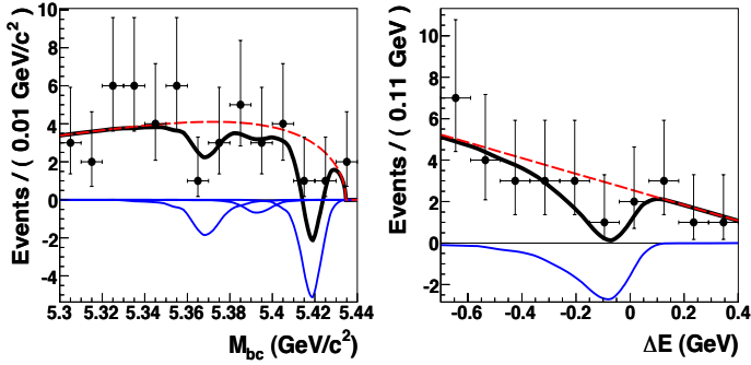
Figure 23.3.11. M_{bc} = m_{ES} and \Delta E projections for B_s^0 \rightarrow \gamma\gamma . The points with error bars show the data; the thin solid curves show the signal contribution; the dashed curves show the continuum contribution; and the thick solid curves show the total. In the m_{ES} figure, the signals (negative) from e^+e^- \rightarrow B_s^0\bar{B}_s^0 , B_s^{*0}\bar{B}_s^0 , and B_s^{*0}\bar{B}_s^{*0} appear from left to right. Plots are from Wicht (2008).
