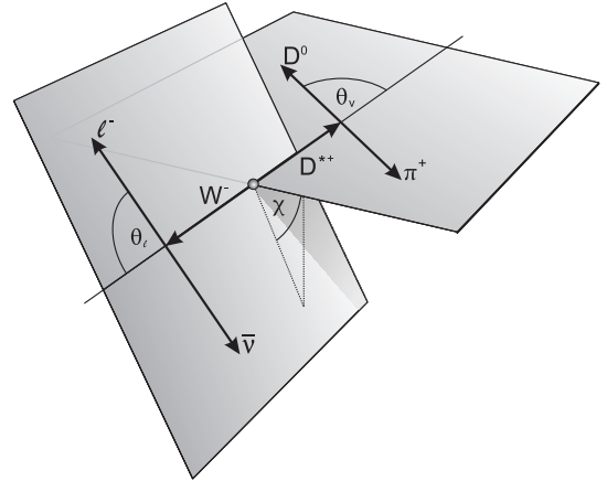
Figure 17.1.5. Definition of the angles \theta_\ell , \theta_V and \chi for the decay \bar{B}^0 \rightarrow D^{*+}\ell^-\bar{\nu} with D^{*+} \rightarrow D^0\pi^+ (Dungel, 2010).
