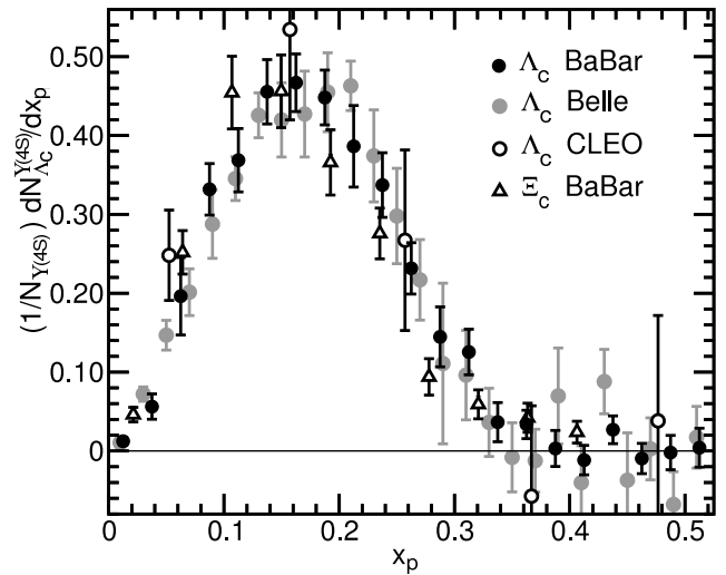
Figure 17.12.1. Differential B \rightarrow \Lambda_c^+ X production rate per \Upsilon(4S) from BABAR (Aubert, 2007p), Belle (Seuster, 2006), and CLEO (Crawford et al., 1992) versus the momentum fraction x_p = p/p_{\max} in the \Upsilon(4S) rest frame. Also shown is the differential \Xi_c^0 production rate normalized to match the peak of the \Lambda_c^+ rate.
