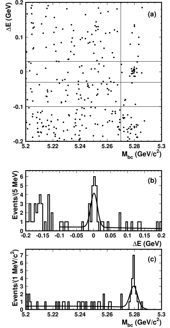
Figure 17.12.2. Candidate events for the decay \bar{B}^0 \rightarrow \Lambda_c^+ \bar{p} from Belle (Gabyshev, 2003): (a) scatter plot of \Delta E versus m_{ES} = M_{bc} , (b) \Delta E distribution for m_{ES} > 5.270 \text{ GeV}/c^2 , and (c) m_{ES} distribution for |\Delta E| < 0.030 \text{ GeV} . The curves indicate the result of a two-dimensional fit.
