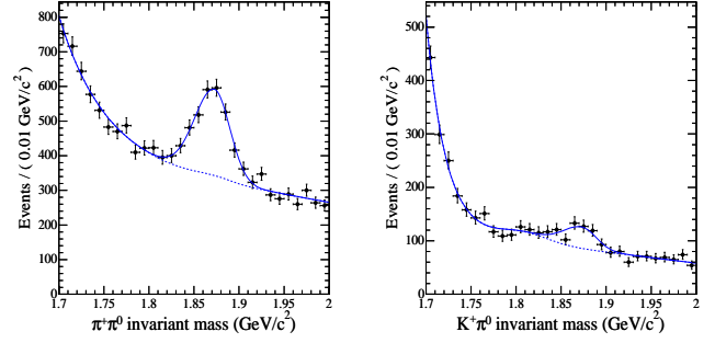
Figure 19.1.10. From (Aubert, 2006v). M(\pi^+\pi^0) and M(K^+\pi^0) with the likelihood fit results. The dashed lines show the projected backgrounds in the D^+ signal region.
