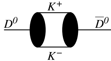
Figure 19.2.2. K^+ K^- as an example of an intermediate state accessible to both D^0 and \bar{D}^0 , contributing to D^0 - \bar{D}^0 mixing. Black circles represent quark processes for D^0 \rightarrow K^+ K^- and its charge conjugate, similar to the process shown in Fig. 19.2.4.
