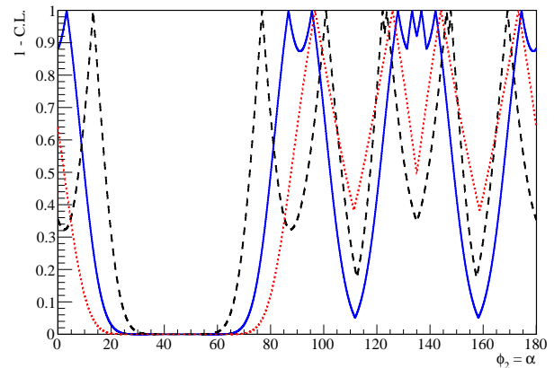
Figure 17.7.11. The solid (blue) curve shows the 1 - C.L. function obtained on \phi_2 = \alpha from the B Factories using the Gronau-London isospin analysis for B \rightarrow \pi\pi decays. The dashed (black) curve shows the BABAR only constraint, the dotted (red) curve shows the Belle only constraint. As discussed in the text, the solutions near \phi_2 = 0 are unphysical and can be removed by extending the isospin analysis.
