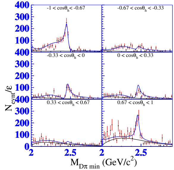
Figure 19.3.5. From (Abe, 2004f). Efficiency-corrected M(D^+\pi^-)_{\min} distribution in B^- \rightarrow D^+\pi^-\pi^- for different helicity angle ranges. Curves correspond to the fit to the total distribution (upper blue) and background (lower black) component.
