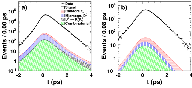
Figure 19.2.20. From (del Amo Sanchez, 2010f). Decay time distributions for (a) D^0 \rightarrow K_S^0 \pi^- \pi^+ , (b) D^0 \rightarrow K_S^0 K^+ K^- decays with the time-dependent Dalitz plot fits described in the text.
