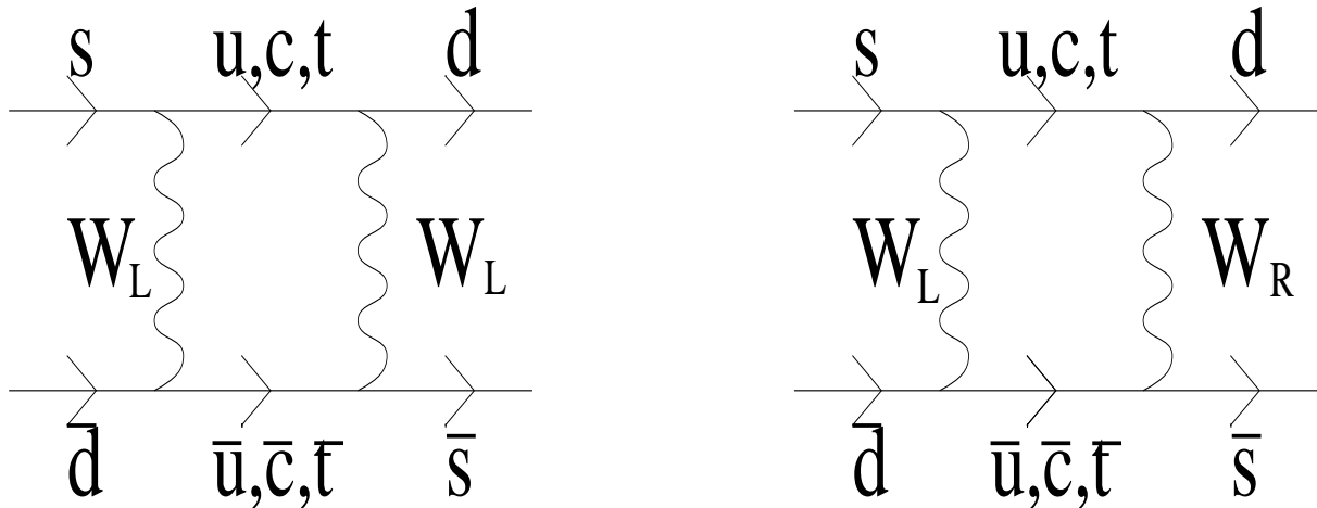
Figure 1: Diagrams showing the dominant box-diagrams contributions to the \Delta S = 2 effective Lagrangian in left-right models.
