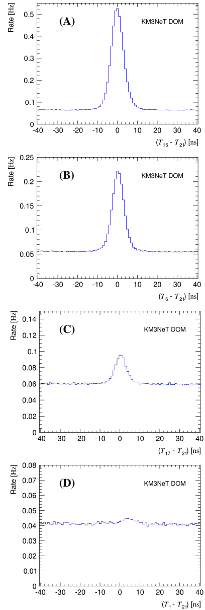
Fig. 4 Distribution of time differences between two PMTs of the DOM, with an angular separation of (A) 33^\circ , (B) 65^\circ , (C) 120^\circ and (D) 165^\circ .
