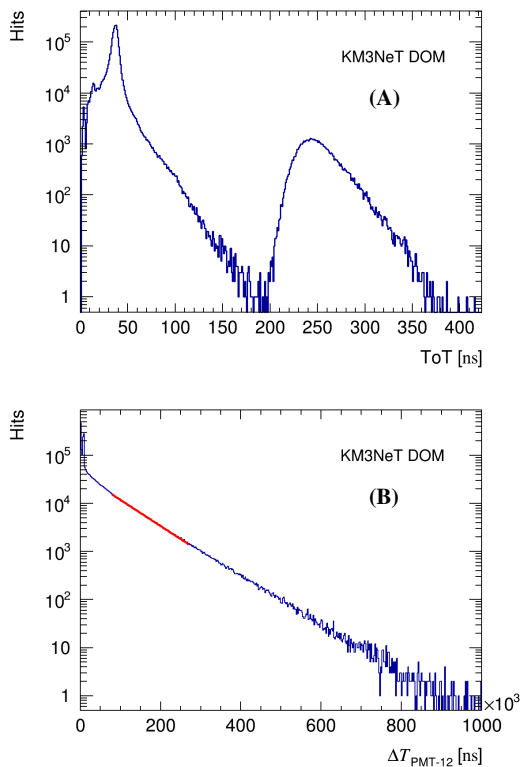
Fig. 2 (A) Numbers of hits as a function of ToT for one of the PMTs. The broad ToT peak corresponds to the large pulse height caused by the laser calibration. (B) Histogram of the time difference between two consecutive hits. The exponential fit, as indicated by the red line, gives a characteristic time \tau = 1.05 \times 10^{-4} s.
