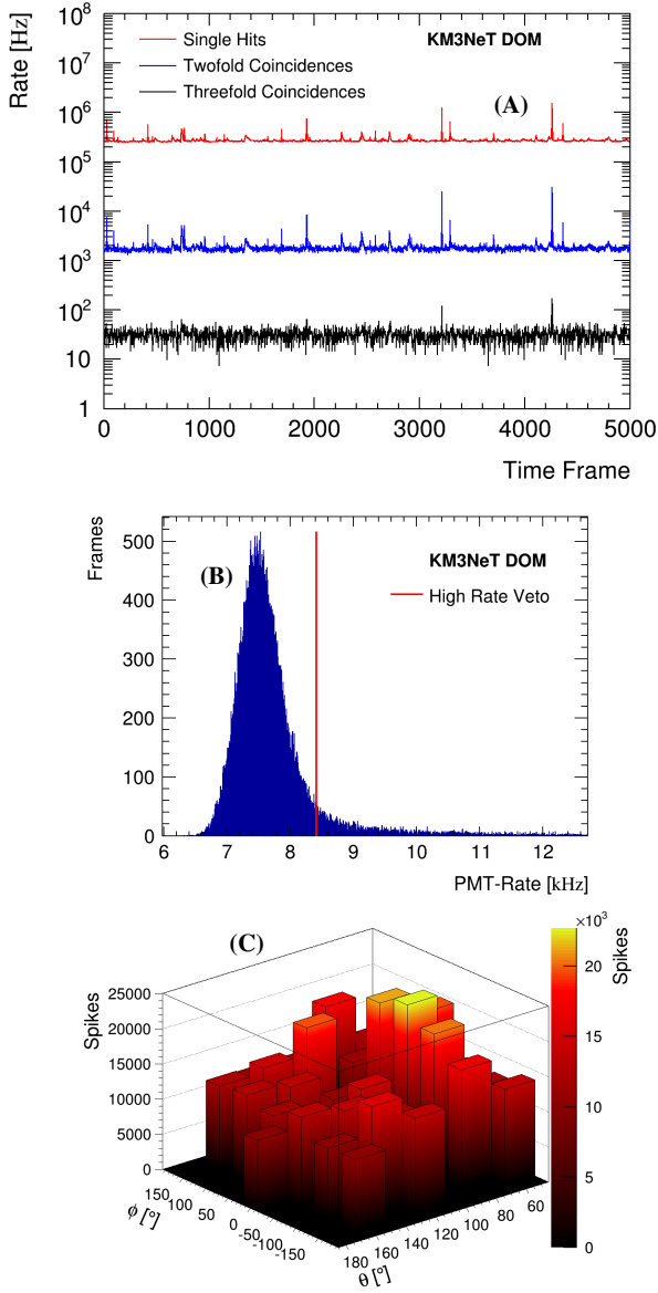
Fig. 3 (A) Aggregate hit rates as a function of the time measured in \sim 134 ms bins. The top trace is for single hits, while the lower traces are for two- and threefold coincidences within a 20 ns window. (B) Histogram of the rate measured in 134 ms timeframe bins for a representative PMT. The rising edge of the histogram is fit to a Gaussian and the cutoff used in the further analysis is set at the mean plus 3 times the standard deviation (indicated by the red line). The cut-off is determined for each PMT separately. (C) The rate of bioluminescent bursts as a function of azimuth and zenith angles. The support structure is viewed by PMTs at small \theta and near \phi = 0^\circ .
