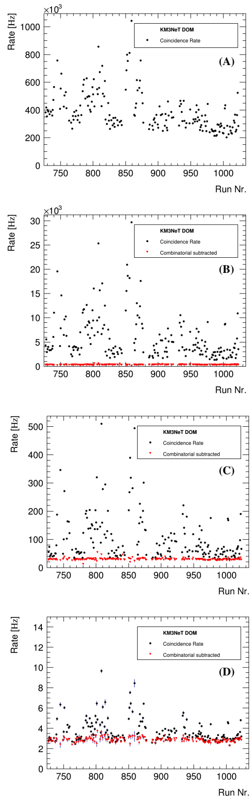
Fig. 6 Aggregate rates as a function of run number for (A) singles, (B) twofold coincidence, (C) threefold coincidence and (D) fourfold coincidence rates. The lower red points show the rates with combinatorial background subtracted and gives the true coincidences from ^{40}\text{K} . The runs cover the period from July to December 2013.
