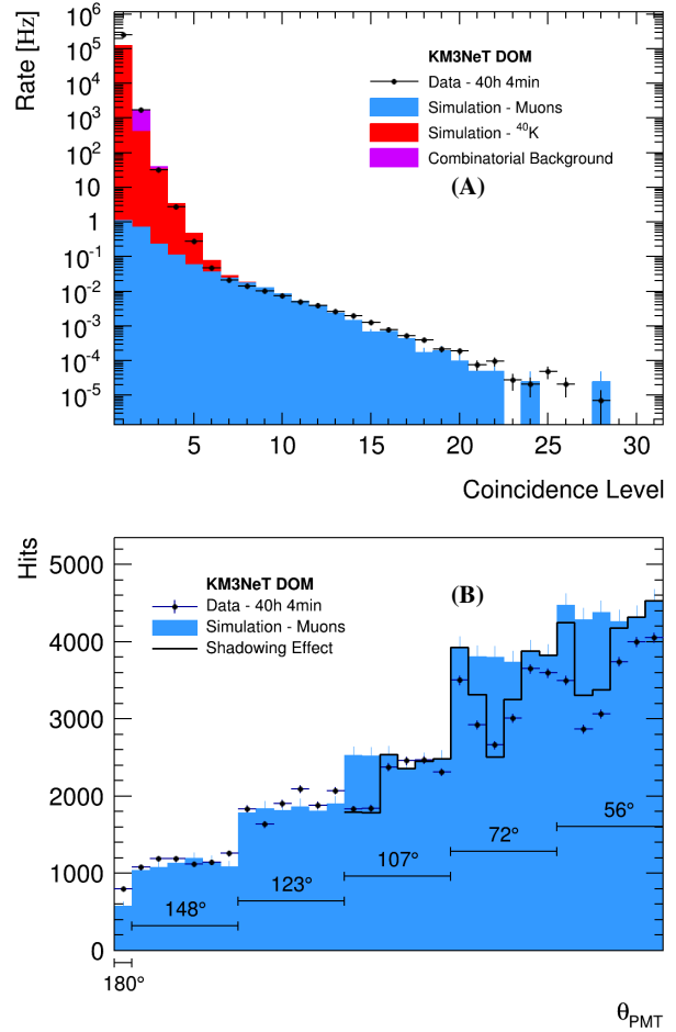
Fig. 7 (A) The rate of events as a function of the coincidence level (number of PMTs with signal in a 20 ns time window). Black dots correspond to data while coloured histograms represent simulations (muons in blue, ^{40}\text{K} in red and accidental coincidences in purple). (B) The number of hits as a function of the zenith position of the centre of the PMT for coincidence levels above seven. One PMT is looking downward ( 180^\circ ). The others are grouped by six at five different angles. The black dots are data, the blue histogram is simulation of atmospheric muons and the black histogram show the calculated effect of the shadowing by the ANTARES electronics cylinder.
