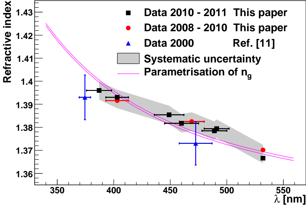
Fig. 5. Index of refraction corresponding to the group velocity of light as a function of the wavelength. Also shown are results from measurements made in [11]. The grey band shows the systematic uncertainty. The two solid lines correspond to a parametrisation of the index of refraction evaluated at a pressure of 200 atm (lower line) and 240 atm (upper line) (see text).
