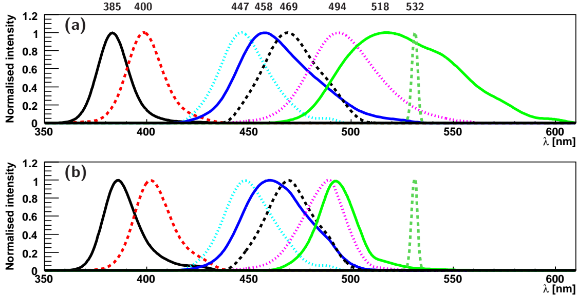
Fig. 2. (a) Wavelength spectra of the light sources used in this work as measured with a calibrated spectrometer. The spectrometer measurements are made in air. The data points have been smoothed and the highest value of each spectrum is set equal to one. On the top of the Figure the peak wavelengths are indicated in units of nm. (b) Simulated light spectra at a distance of 120 m in sea water with the highest value renormalized to one. The differences between the spectra are due to the variation of the absorption length as a function of the wavelength.
