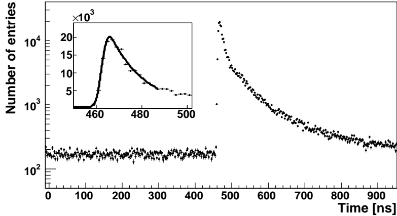
Fig. 3. Example of a distribution of arrival times observed at a distance of 100 m from an LED. The inset shows a zoom around the signal region. The solid curve corresponds to a fit function as described in the text and given in Equation 2.
