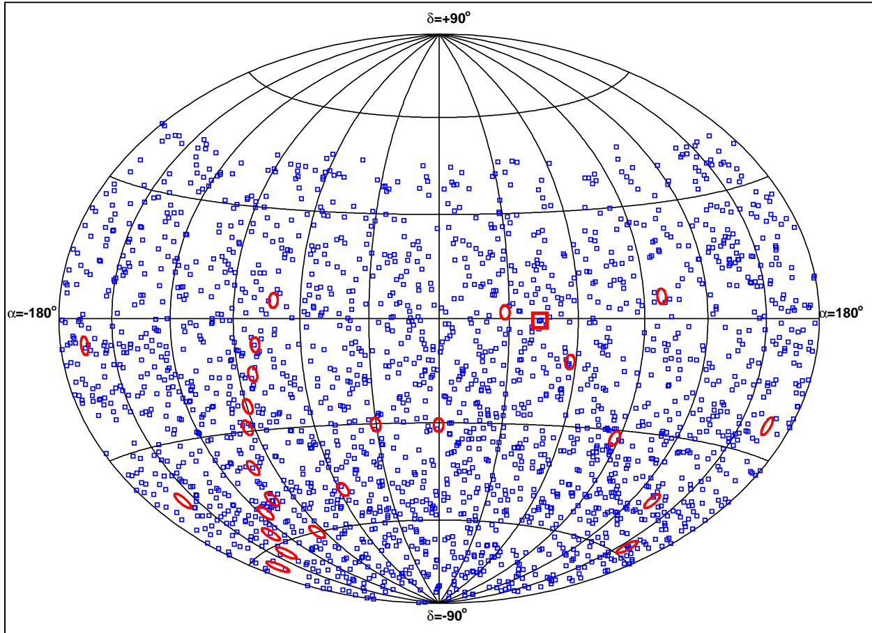
Fig. 3.— Map in equatorial coordinates of the 2190 selected neutrino candidates. The position of the most significant cluster (see text) is indicated by the square. The circles denote the positions of the 24 sources from the candidate list.
