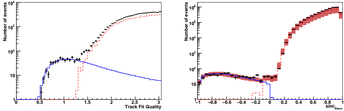
Figure 5: Left : track fit quality for all upward reconstructed multi-line tracks for 2008 data (points with error bars) compared to a Monte Carlo sample of downward-going atmospheric muons (dashed histogram) and upward-going atmospheric neutrinos (solid histogram); right : Elevation angle distribution for events with \bar{Q} < 1.4 . The grey band indicates the error band of the combined prediction from neutrino and muon simulations.
