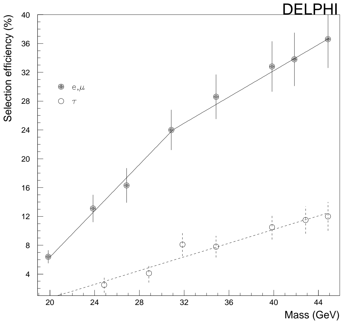
Figure 3: The selection efficiency for a heavy neutrino event as a function of the mass ( r=0.01 cm).
