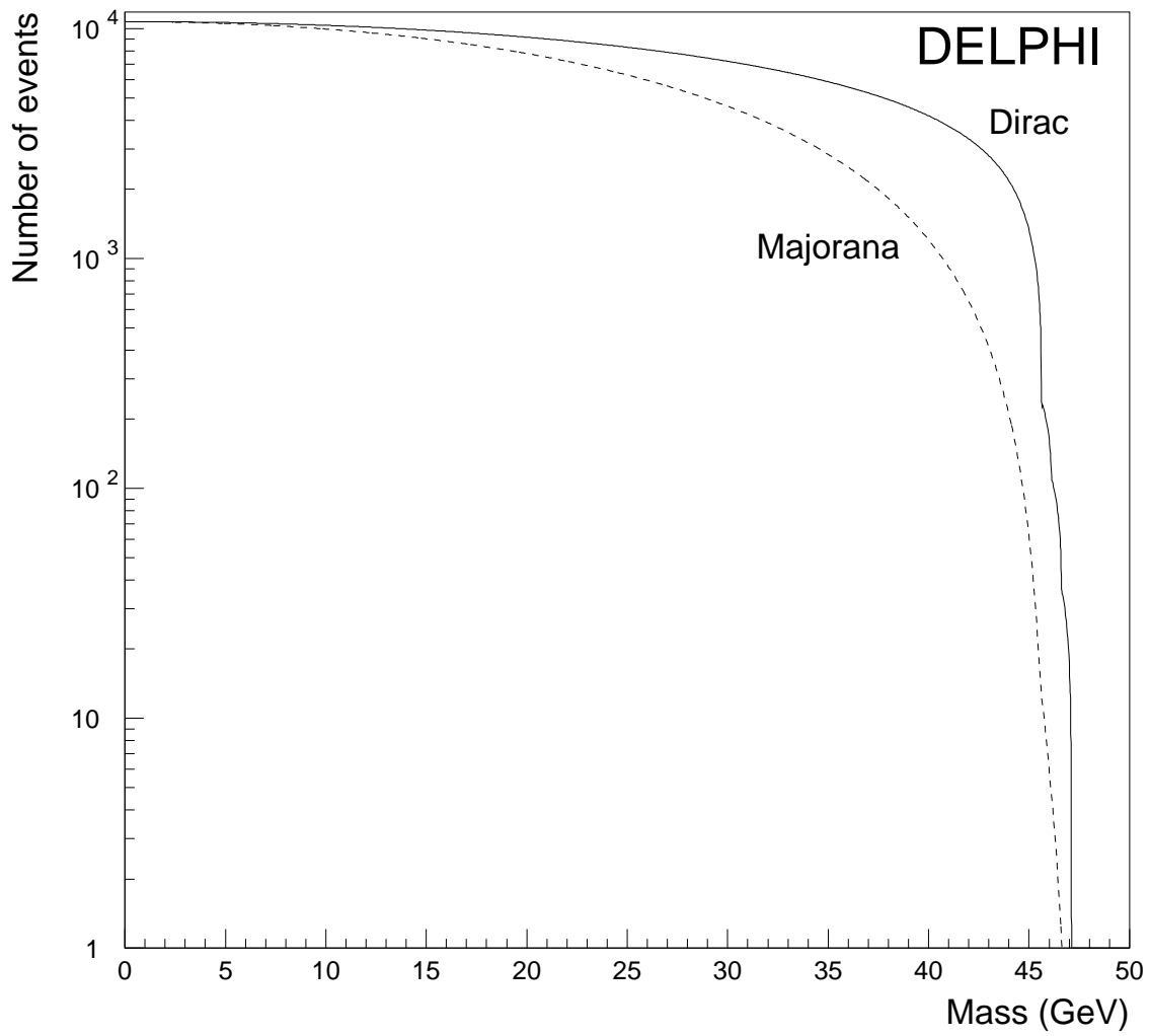
Figure 2: The number of produced heavy neutrino events as a function of the mass of the neutrino.
