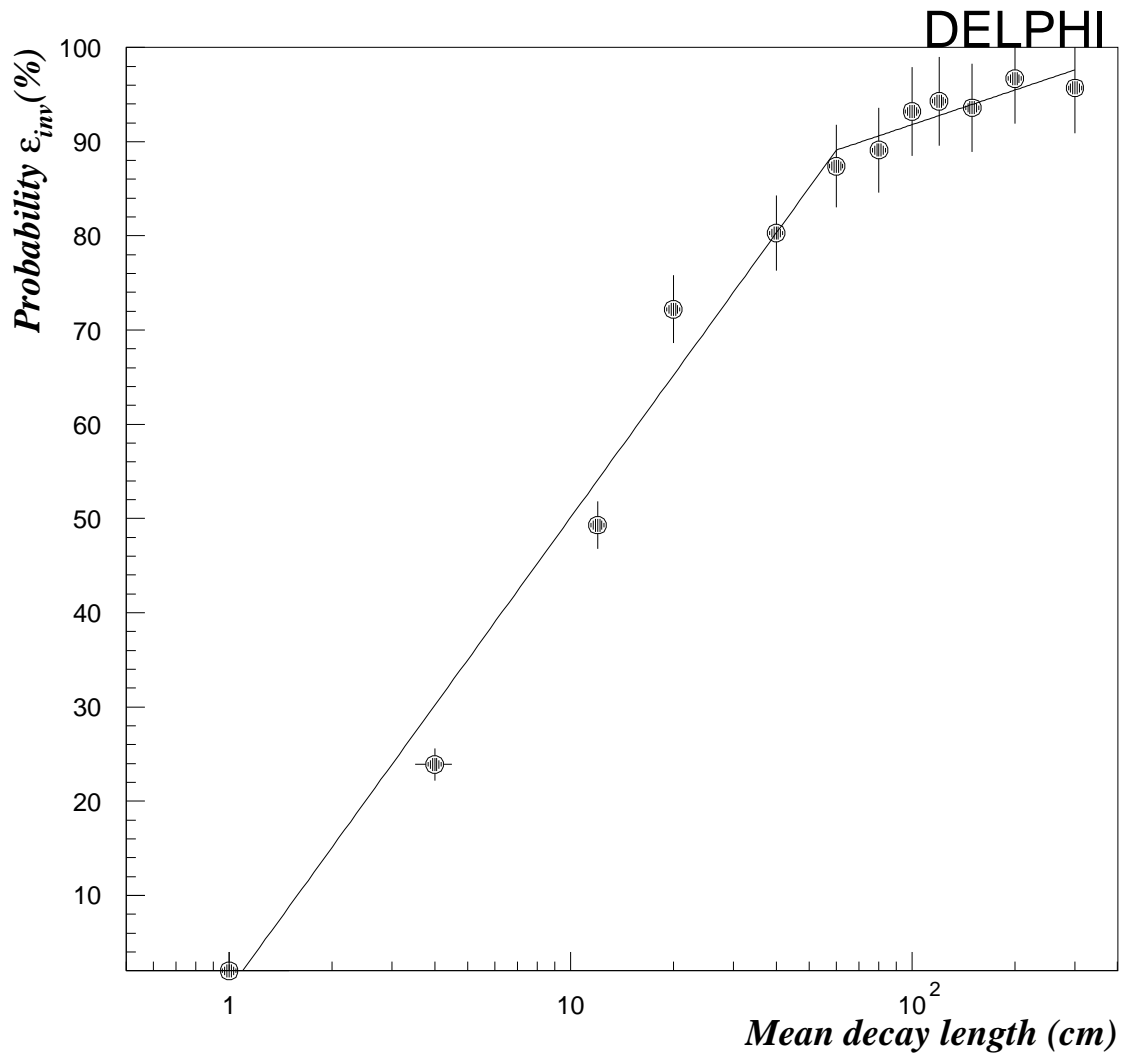
Figure 1: The probability that a heavy neutrino event contributes to the \Gamma_{inv} as a function of the logarithm of the mean decay length of the neutrino.
