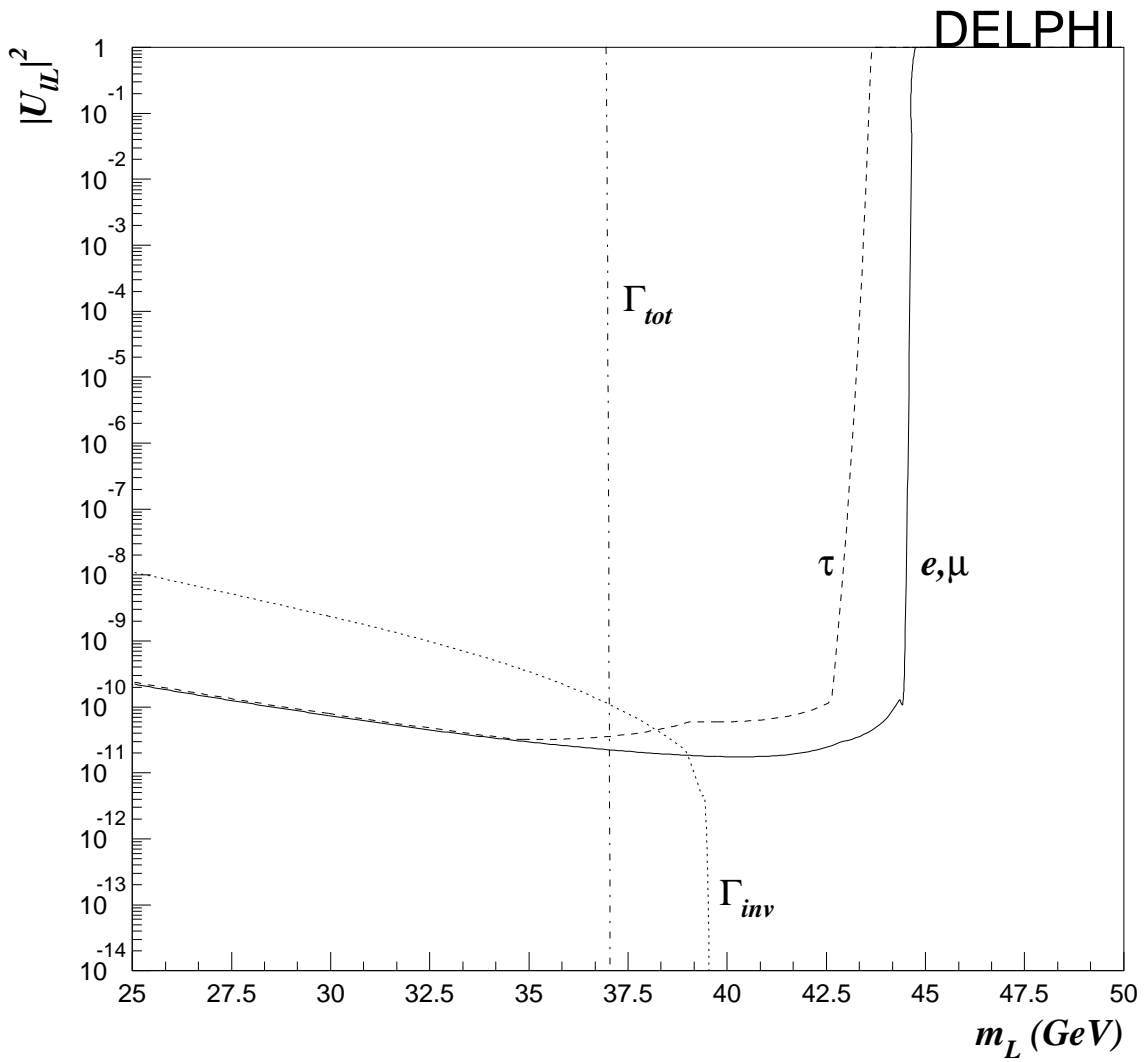
Figure 6: The 95 % CL limits on |U_{lL}|^2 as a function of m_L for e, \mu and \tau mixing for a Majorana neutrino, assuming mixing with one family.
