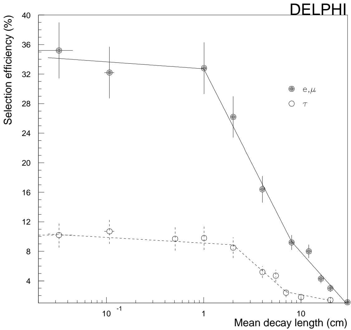
Figure 4: The selection efficiency for a heavy neutrino event as a function of the logarithm of the mean decay length ( m_L = 40 GeV).
