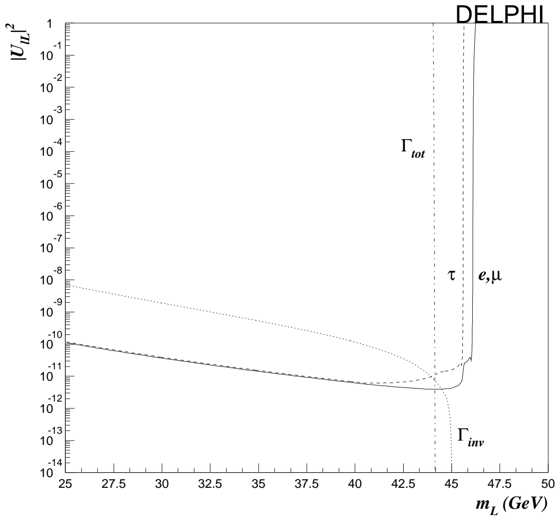
Figure 5: The 95 % CL limits on |U_{lL}|^2 as a function of m_L for e, \mu and \tau mixing for a Dirac neutrino, assuming mixing with one family.
