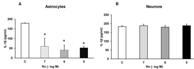
Fig 4. Cytokine IL-1 \beta determination. Astrocytes (panel A) or neurons (panel B) were incubated without Rn (control, C) or with Rn ( 10^{-7} , 10^{-6} , 10^{-5} M) and cell culture supernatants were harvested. IL-1 \beta secretion were determined by ELISA. Values are means \pm SD of replicate experiments from four independent experiments (four different rats). * p < 0.05 vs control.
