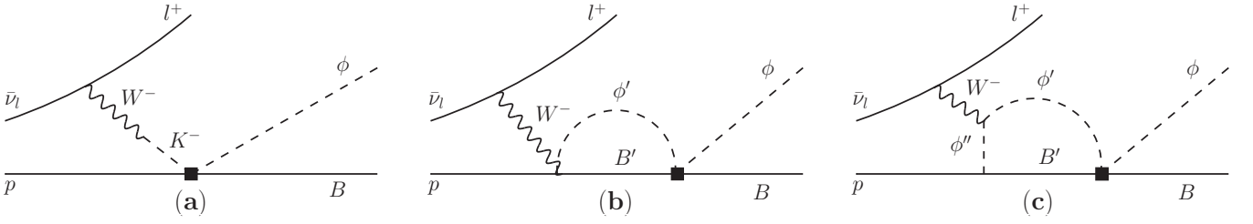
FIG. 2. Iterated loop diagrams for \bar{\nu}_\mu p \rightarrow \mu^+ \phi B . The solid boxes represent the T matrix of the ten coupled channels.
