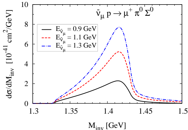
FIG. 3. (color online). Differential cross section for the reaction \bar{\nu}_\mu p \rightarrow \mu^+ \pi^0 \Sigma^0 as a function of the invariant mass M_{\text{inv}} of the final meson baryon system for three different incident antineutrino energies.
