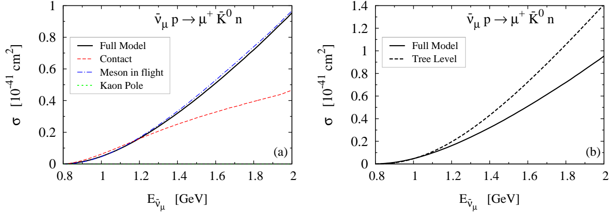
FIG. 8. (color online). Integrated cross section for the \bar{\nu}_\mu p \rightarrow \mu^+ \bar{K}^0 n reaction. The line styles have the same meanings as in Fig. 7.
