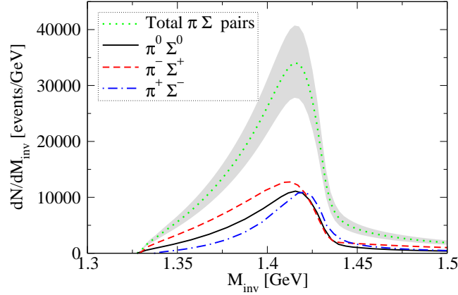
FIG. 9. (color online). Invariant mass distribution of \pi\Sigma events, primarily produced at the MINER \nu A scintillator detector. The grey band corresponds to a 10% error in the form factor parameter M_F .
