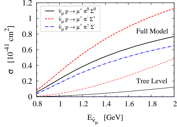
FIG. 6. (color online). Cross sections as a function of the antineutrino energy for the three \bar{\nu}_\mu p \rightarrow \mu^+ \pi \Sigma reaction channels. The three upper curves have been obtained with the full model while the two lower ones with tree level contributions alone. The later is absent for the \pi^+ \Sigma^- channel.
