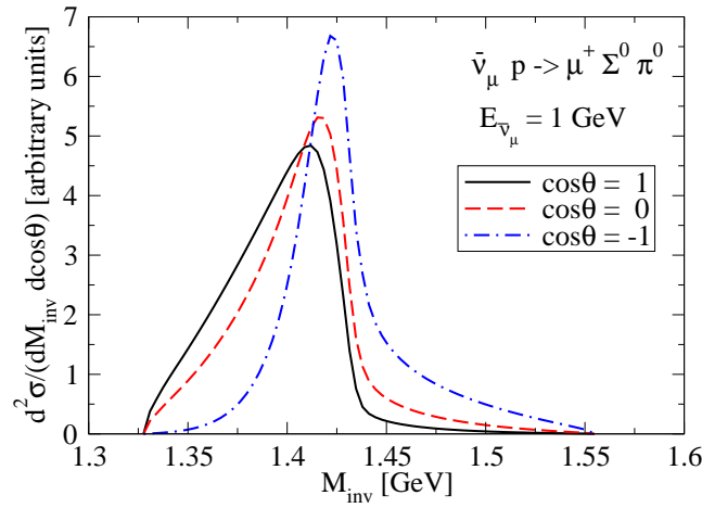
FIG. 4. (color online). Area normalized double differential cross section for \bar{\nu}_\mu p \rightarrow \mu^+ \pi^0 \Sigma^0 at E_{\bar{\nu}_\mu} = 1 GeV, as a function of M_{inv} for three different values of the angle ( \theta ) between the incoming neutrino and the outgoing muon in the reaction CM frame.
