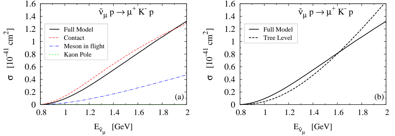
FIG. 7. (color online). Integrated cross section for the \bar{\nu}_\mu p \rightarrow \mu^+ K^- p reaction as a function of the antineutrino energy. Left panel: contribution of the different terms to the full model result. The KP contribution is negligible and cannot be discerned in the plot. Right panel: comparison between the full model and tree level calculations.
