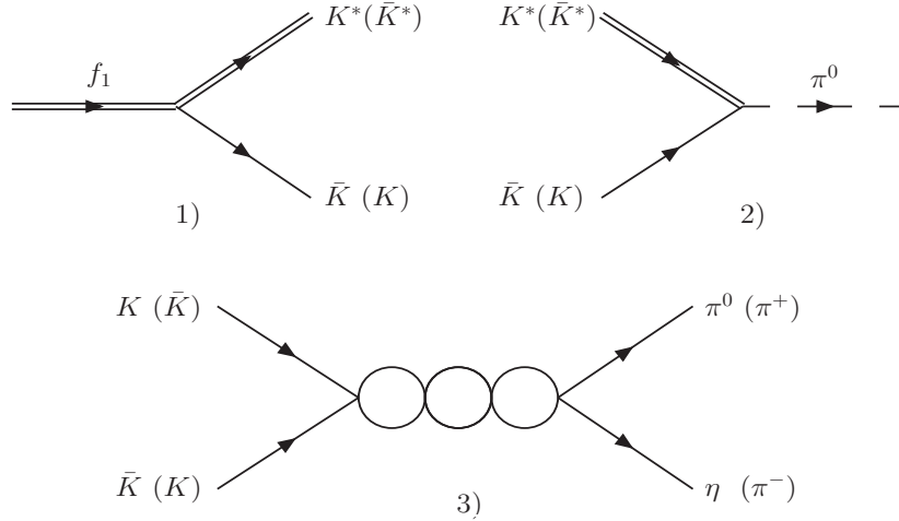
FIG. 2. Vertices involved in the decay of the f_1(1285) to \pi^0 \eta or \pi^+ \pi^- , the f_1(1285) \rightarrow K^* \bar{K} 1) and the VPP vertex 2), and amplitude for a_0(980) and f_0(980) production 3).
