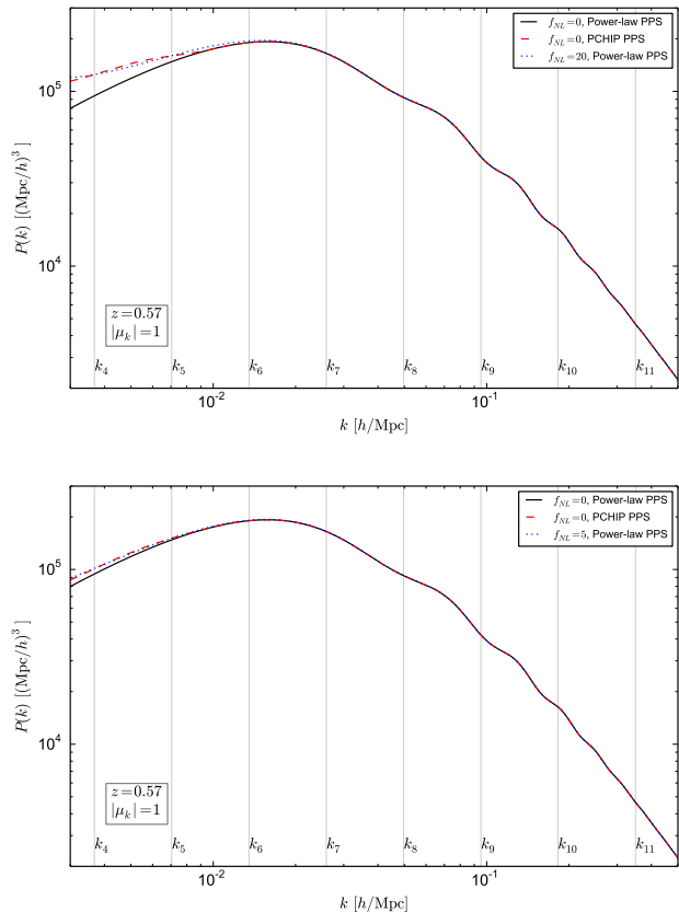
FIG. I: The upper panel depicts the galaxy power spectrum for the standard PPS power law case, for f_{\text{NL}} = 0 (black solid curve) and f_{\text{NL}} = 20 (blue dotted curve), together with a PCHIP PPS case (red dashed lines) for f_{\text{NL}} = 0 . The values of the PCHIP PPS nodes are chosen accordingly to match the predictions of the f_{\text{NL}} = 20 case. The lower panel shows the equivalent but for f_{\text{NL}} = 5 . We have also changed accordingly the value of the PCHIP PPS nodes. We also show with k_i for i = 4, \dots, 11 the k position of five of the nodes considered in our analysis ( i = 5, \dots, 9 ), plus k_{4,10,11} that lie outside the k range probed by the DESI experiment. The galaxy power spectra are obtained for z = 0.57 , |\mu_k| = 1 and assuming a constant gaussian bias b_G .
