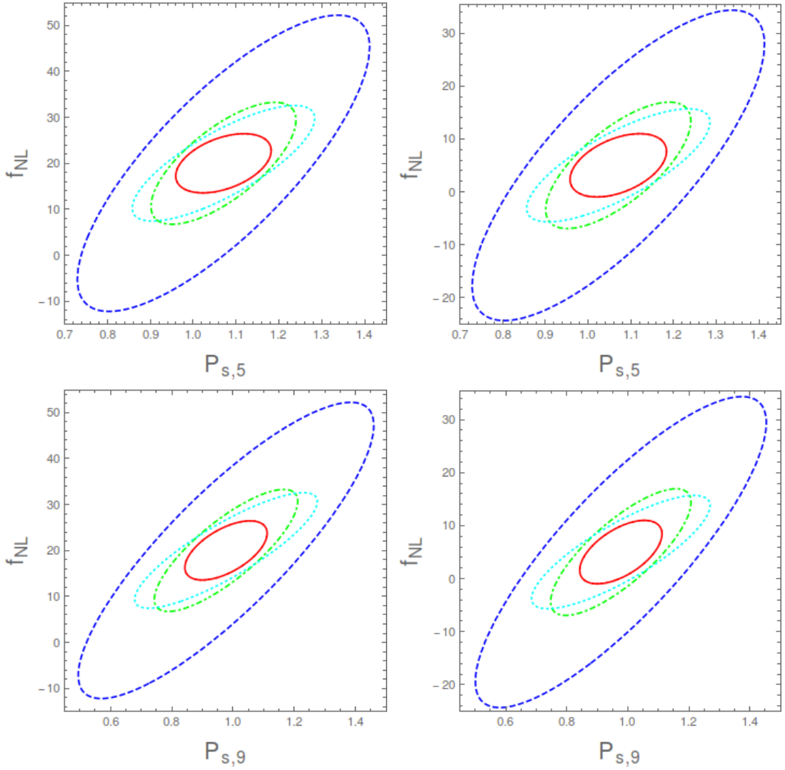
FIG. II: The upper left (right) panel shows the f_{\text{NL}} - P_{s,5} degeneracy, for a fiducial cosmology with f_{\text{NL}} = 20 ( f_{\text{NL}} = 5 ), assuming k_{\text{max}} = 0.1h/\text{Mpc} . We show the 1 - \sigma marginalized contours associated to the LRGs (in dashed blue lines), ELGs (in dot-dashed green lines), QSOs (in dotted cyan lines) and multi-tracer (in solid red) Fisher matrix analyses. The bottom panels shows the analogous but in the (f_{\text{NL}} - P_{s,9}) plane.
