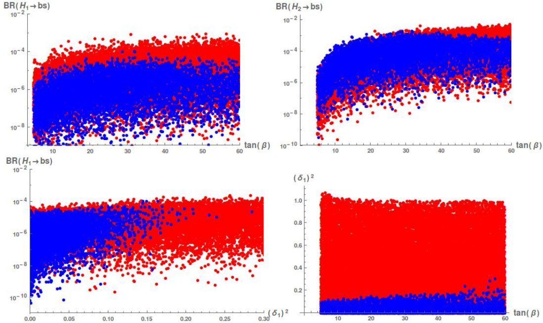
FIG. 3: A generic supersymmetric SM with L insertion with \delta_L \neq 0 and \delta_{A_u} = \delta_R = 0 : The upper frames show the dependence of the estimated branching ratios for H_{1,2} \rightarrow \bar{b}s + \bar{s}b on \tan\beta . The lower-left frame is for the dependence of \text{B}(H_1 \rightarrow bs) on \delta_1^2 and the lower-right frame for the \delta_1^2 dependence on \tan\beta . Blue (dark) points satisfy all the constraints considered, while red (light) points violate one or several of these constraints.
