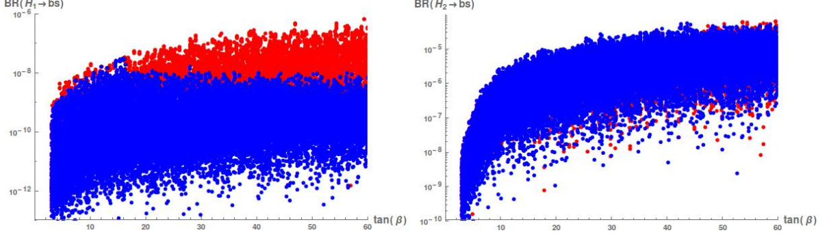
FIG. 2: A full MSSM framework with RR insertion with \delta_R \neq 0 and \delta_{A_u} = \delta_L = 0 : The left frame shows the dependence of \text{BR}(H_1 \rightarrow bs) on \tan\beta and the right frame shows the dependence of \text{BR}(H_2 \rightarrow bs) on \tan\beta . Again, blue (dark) points satisfy all the constraints considered, while red (light) points violate one or several of these constraints.
