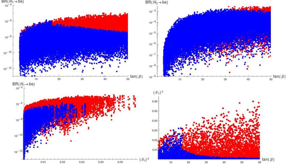
FIG. 1: A full MSSM framework with LL insertion with \delta_L \neq 0 and \delta_{A_u} = \delta_R = 0 : The upper frames show the dependence of the estimated branching ratios for H_{1,2} \rightarrow \bar{b}s + \bar{s}b on \tan\beta . The lower-left frame is for the dependence of B(H_1 \rightarrow bs) on \delta_1^2 and the lower-right frame for the \delta_1^2 dependence on \tan\beta . Blue (dark) points satisfy all the constraints considered, while red (light) points violate one or several of these constraints.
