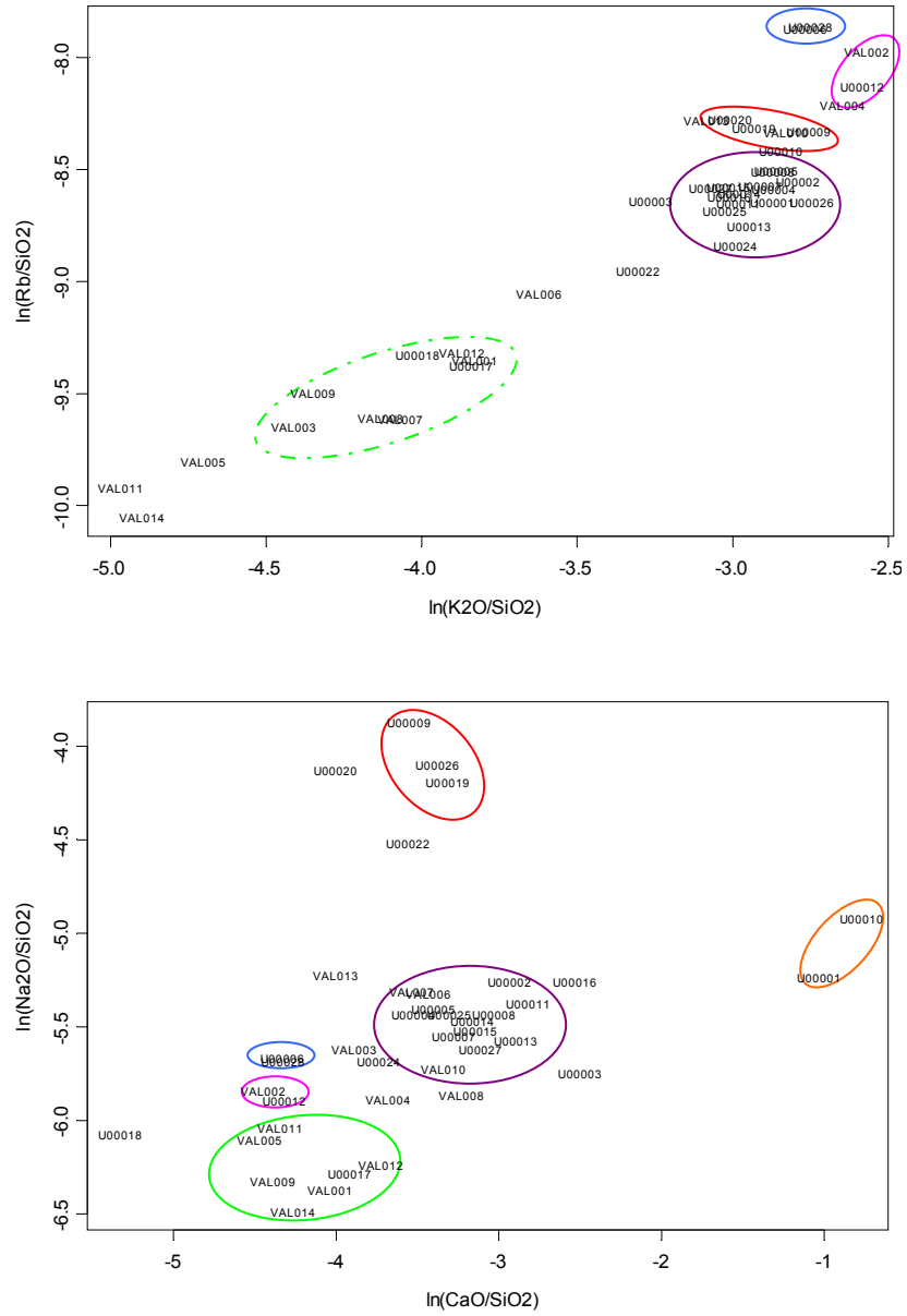
Figura3. Diagrames bivariants. Dalt: \ln(\text{K}_2\text{O}/\text{SiO}_2) - \ln(\text{Rb}/\text{SiO}_2) . Baix: \ln(\text{CaO}/\text{SiO}_2) - \ln(\text{Na}_2\text{O}/\text{SiO}_2)
