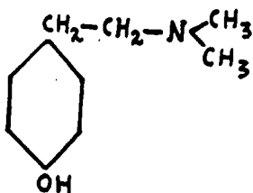
Hordenina
