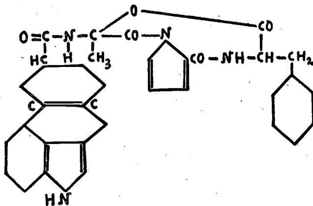
Ergotamina
