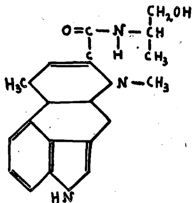
Ergobasina
