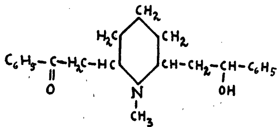
Lobelina
