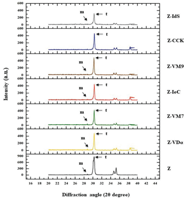
Fig. 9: X-Ray diffraction analysis pattern of zirconia (Z) and zirconia veneered with VITADur® alpha (Z- VDα), VITAVM®7 (Z-VM7), IPSe.max® ceram (Z-IeC), VITAVM®9 (Z-VM9), Cercon® ceramkiss (Z-CCK), and IPS dSIGN® (Z-IdS).
