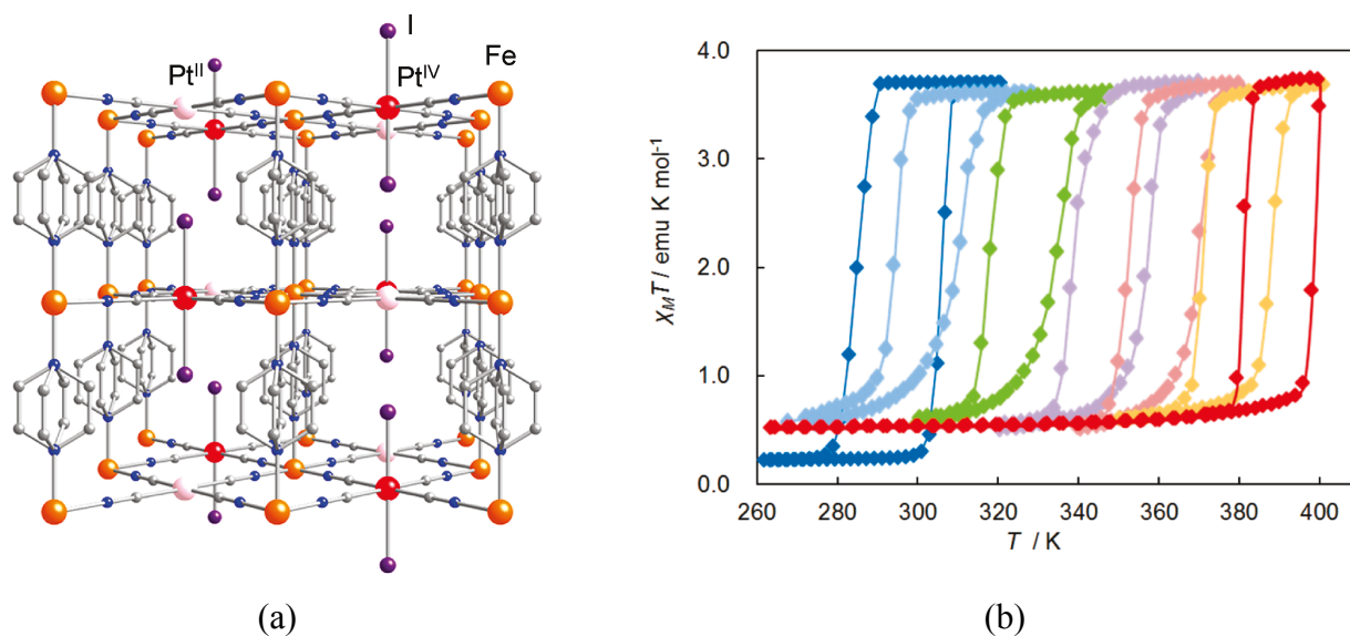
Figure 21. a) Crystal structure of \{\text{Fe}(\text{pz})[\text{Pt}^{\text{II/IV}}(\text{CN})_4(\text{I})]\} . Atoms: Fe (orange), \text{Pt}^{\text{II}} (pink), \text{Pt}^{\text{IV}} (red), I (purple), C (gray), N (blue). b) Magnetic behavior of \{\text{Fe}(\text{pz})[\text{Pt}(\text{CN})_4(\text{I})_n]\} n = 0.0 (blue); 0.1 (sky blue); 0.3 (green); 0.5 (violet); 0.7 (pink); 0.9 (orange); 1.0 (red). Reprinted with permission from reference 68, Copyright 2011 American Chemical Society.
