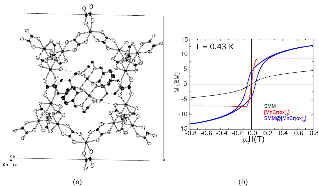
Figure 30. a) Crystal structure of [\text{Mn}^{\text{III}}(\text{salen})(\text{H}_2\text{O})]_2[\text{Mn}^{\text{II}}\text{Cr}^{\text{III}}(\text{ox})_3]_2 \cdot (\text{MeOH})_3 \cdot (\text{CH}_3\text{CN}) . Hydrogen atoms and disordered solvent molecules have been omitted for clarity. b) Magnetization hysteresis loops of the hybrid SMM@MnCr (blue), the SMM in a diamagnetic network (black) and MnCr (red) measured at T = 0.43 K. The sweeping field rate was 6 \text{ mTs}^{-1} . Adapted from reference 115, with permission of John Wiley and Sons.
