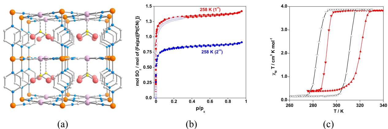
Figure 20. a) Fragment of the structure of {Fe(pz)[Pt II (CN) 4 ]}·SO 2 . Colour code: Fe (orange), Pt (light pink), S (yellow), N (blue), C (grey). b) SO 2 sorption–desorption isotherms for {Fe(pz)[Pt II (CN) 4 ]} at 293 K (○) and at 258 K (●). Red and blue colour codes refer to the first and second sorption–desorption cycles, respectively. c) Magnetic properties of {Fe(pz)[Pt II (CN) 4 ]} (black line) and {Fe(pz)[Pt II (CN) 4 ]}·SO 2 (red line). Reprinted with permission from reference 66, Copyright 2013 American Chemical Society.
