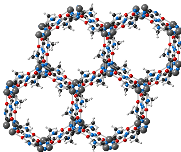
Figure 8. Crystal structure of Co(imidazolate-4-amide-5-imidate)·0.5DMF. Adapted from reference 38, with permission from The Royal Society of Chemistry.
