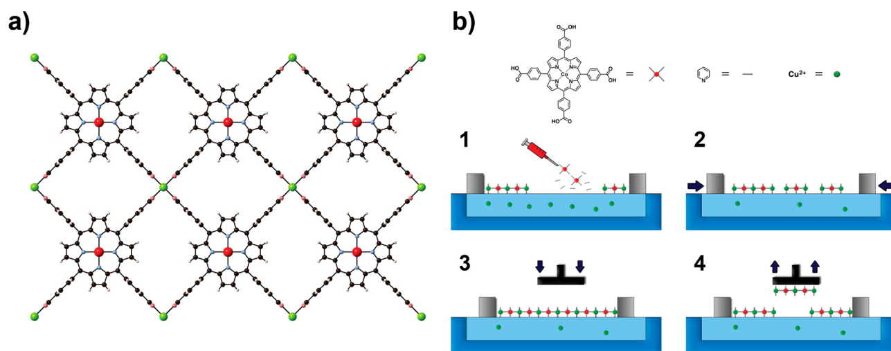
Figure 31. NAFS-1 structure (a) and Langmuir–Blodgett (LB) transfer process (b). Reprinted with permission from reference 128, Copyright 2016 American Chemical Society.
