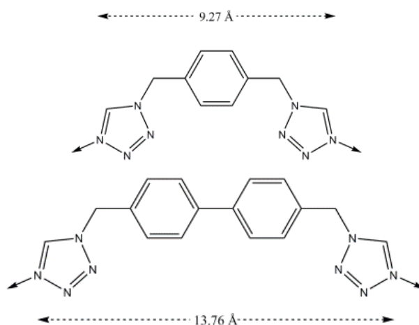
Figure 18. Chemical structures of the ligands btzx (top) and btzbp (bottom). The dashed arrows
