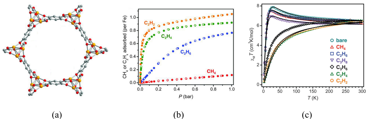
Figure 12. a) Crystal structure of MOF-74; b) Gas adsorption isotherms for methane, ethane, ethylene, and acetylene in Fe-MOF-74 at 318 K; c) Variable-temperature magnetic susceptibility data in an applied field of 1 kOe for samples of Fe-MOF-74 in a vacuum (bare) and under 1 bar of the indicated hydrocarbon (black lines represent magnetic fits). Adapted from reference 43, with permission of the AAAS.
