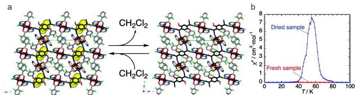
Figure 15. a) Reversible \text{CH}_2\text{Cl}_2 extrusion/uptake in [\{\text{Ru}_2(\text{O}_2\text{CPh}-\text{o}-\text{Cl})_4\}_2\text{TCNQ}(\text{MeO})_2]\cdot\text{CH}_2\text{Cl}_2 provokes subtle changes that affect the pendant ligand (the \text{CH}_2\text{Cl}_2 molecules are represented by a yellow CPK model); b) effects of the desolvation in the magnetic properties of the Ru coordination polymer: variation of 1 Hz ac susceptibilities \chi'' (zero dc field and 3 Oe ac oscillating field) of the solvated and desolvated compounds. Reprinted with permission from reference 55, Copyright 2010 American Chemical Society.
