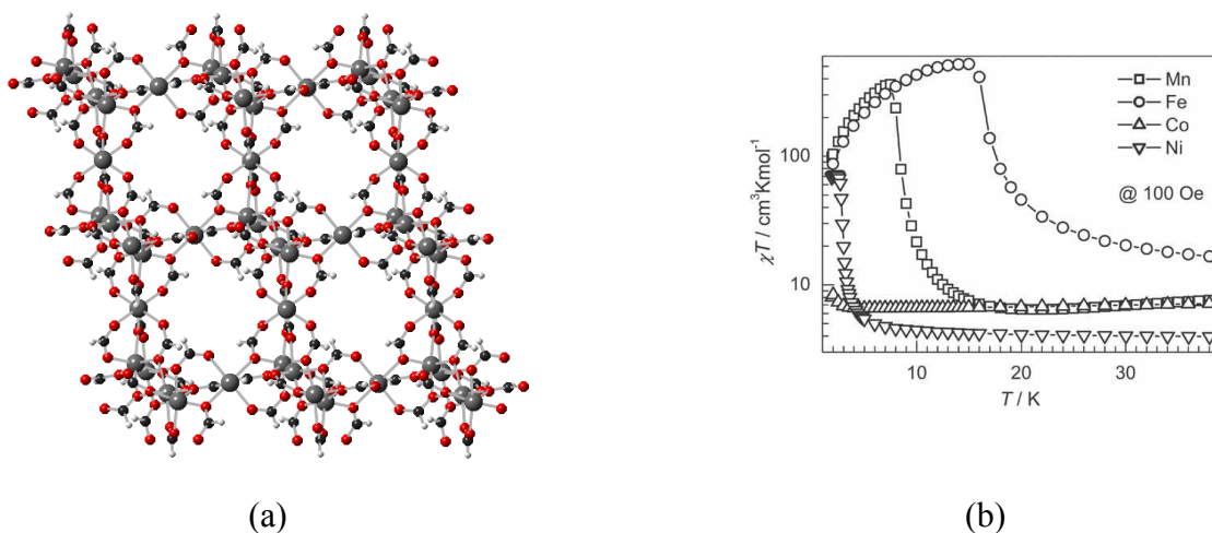
Figure 5. Crystal structure of M_3(\text{HCOO})_6 ; b) Temperature dependence of susceptibility for [M_3(\text{HCOO})_6] of M=\text{Mn, Fe, Co, and Ni} between 2–40 K. Note that the \chi T scale is logarithmic for easy representation of the large difference in \chi T values for different compounds. Adapted from reference 26, with permission from Wiley.
