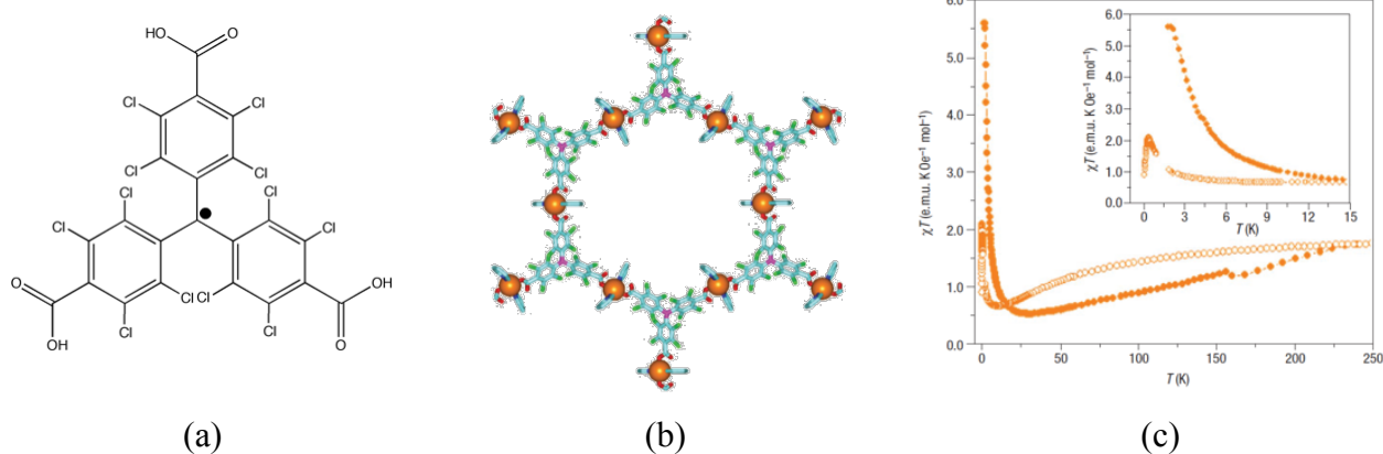
Figure 14. a) Schematic representation of the ptmtc radical ligand; b) Structure of \{[\text{Cu}_3(\text{ptmtc})_2(\text{py})_6(\text{EtOH})_2(\text{H}_2\text{O})]\} showing the open-framework; c) Value of \chi T as a function of the temperature for MOROF-1 (orange filled circle, MOROF-1; open circle, evacuated MOROF-1). Adapted from reference 52, with permission from the Nature Publishing Group.
