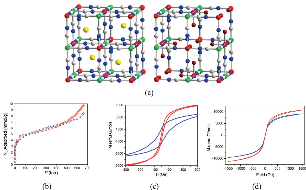
Figure 6. a) Crystal structure of \text{CsNi}[\text{Cr}(\text{CN})_6] (left) and \text{Cr}_3[\text{Cr}(\text{CN})_6]_2 \cdot 6\text{H}_2\text{O} (right); b) Nitrogen adsorption isotherms for \text{CsNi}[\text{Cr}(\text{CN})_6] (red squares) and \text{Cr}_3[\text{Cr}(\text{CN})_6]_2 \cdot 6\text{H}_2\text{O} (blue circles), as measured at 77 K; c) Magnetic hysteresis loops, measured at 5 K, of \text{Cr}_3[\text{Cr}(\text{CN})_6]_2 \cdot 6\text{H}_2\text{O} (blue) and \text{Cr}_3[\text{Cr}(\text{CN})_6]_2 \cdot 6\text{H}_2\text{O} sealed in a quartz tube containing 2.9 molecules of \text{O}_2 per formula unit (red); d) Magnetic hysteresis loops, measured at 2 K of \text{CsNi}[\text{Cr}(\text{CN})_6] (blue) and \text{CsNi}[\text{Cr}(\text{CN})_6] sealed in a quartz tube containing 1.8 molecules of \text{O}_2 per formula unit (red). Reproduced from reference 30, Copyright 2008 American Chemical Society. Further permissions related to this material should be directed to the ACS.
