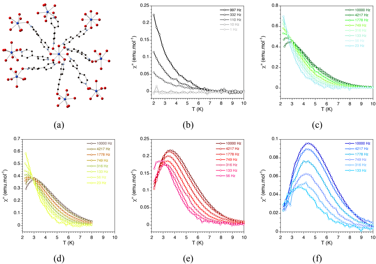
Figure 23. a) Crystal structure of \text{Ln}(\text{bipyNO})_4(\text{TfO})_3 . Out-of-phase dynamic susceptibility under different external dc magnetic fields: b) 4 G; c) 1000 G; d) 2000 G; e) 5000 G; and f) 10000 G. Solid lines are eye-guides. Adapted from reference 76, with permission of John Wiley and Sons.
