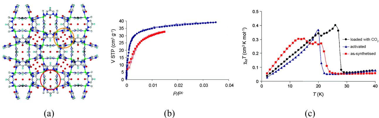
Figure 10. a) Crystal structure of [\text{Cu}(\text{F-pymo})_2(\text{H}_2\text{O})_{1.25}]_n ; b) \text{CO}_2 adsorption isotherm of activated sample of [\text{Cu}(\text{F-pymo})_2]_n at 273 K (circles) and 298 K (squares), with the open symbols denoting desorption; c) Effect of the \text{CO}_2 sorption in the magnetic behavior of [\text{Cu}(\text{F-pymo})_2]_n at an external magnetic field of 100 Oe. Reprinted with permission from reference 40, Copyright 2008 American Chemical Society.
