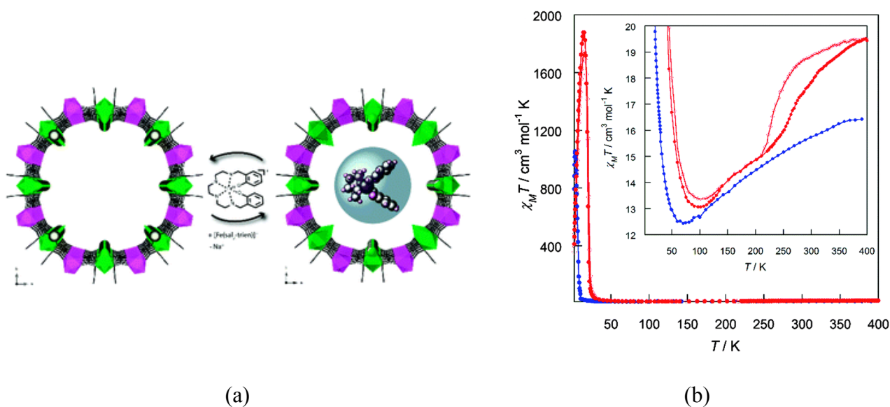
Figure 29. a) Schematic representation of the SC to SC cation exchange process leading to the hybrid \text{Fe}(\text{sal}_2\text{-trien})@\text{Mn}^{\text{II}}\text{Cu}^{\text{II}} MOF. b) \chi_M T versus T plot for \text{Mn}^{\text{II}}\text{Cu}^{\text{II}} MOF (blue) and \text{Fe}(\text{sal}_2\text{-trien})@\text{Mn}^{\text{II}}\text{Cu}^{\text{II}} MOF (red). The inset shows the minima and the high temperature region in detail, emphasising the thermal hysteresis loop. The full and empty circles represent the \text{Fe}(\text{sal}_2\text{-trien})@\text{Mn}^{\text{II}}\text{Cu}^{\text{II}} MOF data recorded in the heating and cooling modes respectively. Adapted from reference 114, with permission from The Royal Society of Chemistry.
