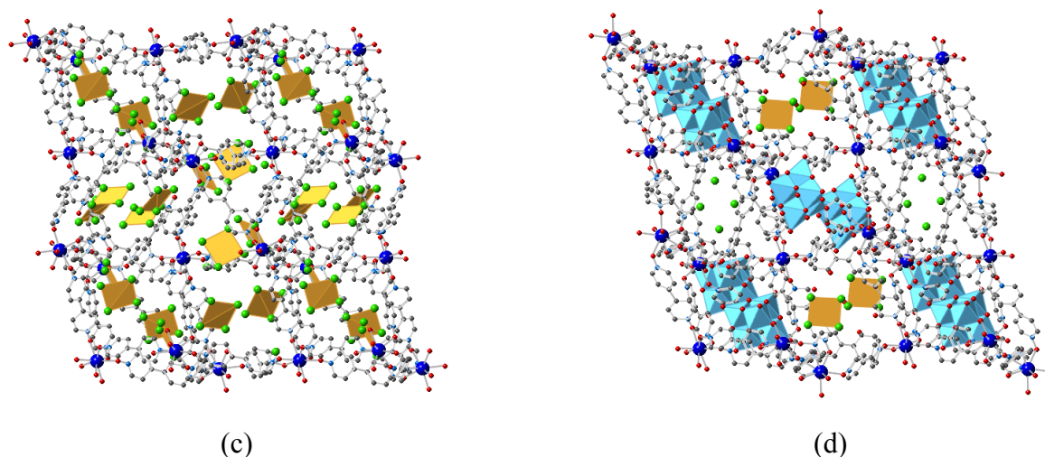
Figure 24. Crystal structures after anion exchange in \text{Ln}(\text{bipyNO})_4(\text{TfO})_3 with different anions: a) [\text{W}_6\text{O}_{19}]^{2-} ; b) [\text{Mo}_6\text{O}_{19}]^{2-} ; c) [\text{AuCl}_4]^- ; and d) the mixed system [\text{W}_6\text{O}_{19}]^{2-} , and [\text{AuCl}_4]^- . [\text{W}_6\text{O}_{19}]^{2-} , [\text{Mo}_6\text{O}_{19}]^{2-} , [\text{AuCl}_4]^- and \text{Cl}^- anions shown in blue, purple, orange and green, respectively.
