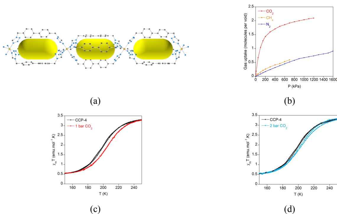
Figure 19. a) Crystal structure of CCP-4 viewed along the b -axis. The \text{BF}_4^- anions and hydrogen atoms have been removed for clarity. Key: Fe, orange; C, gray; N, blue. The yellow ellipsoids are placed in the structure to represent the empty space of the internal voids; b) Gas sorption isotherms at 298 K for \text{CO}_2 , \text{CH}_4 and \text{N}_2 for CCP-4 ; c) Temperature dependence product of the magnetic susceptibility times the temperature ( \chi_m T ) for activated CCP-4 (black) and CCP-4 loaded with one molecule of \text{CO}_2 in each void (red line). d) Temperature dependence product of the magnetic susceptibility times the temperature ( \chi_m T ) for activated CCP-4 (black) and CCP-4 loaded with two molecules of \text{CO}_2 in each void (blue line). Adapted from reference 64, with permission from The Royal Society of Chemistry.
