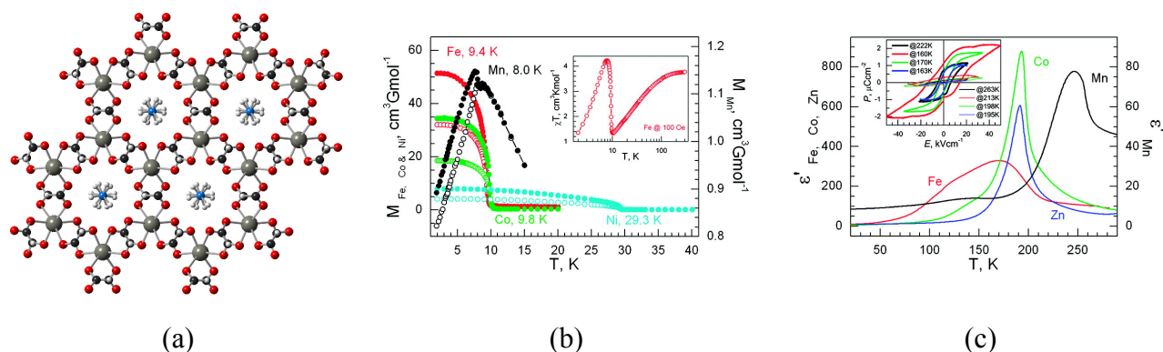
Figure 4. a) Crystal structure of [NH 4 ][M(HCOO) 3 ]; b) Zero-field-cooled (open symbols) and field-cooled (filled symbols) magnetization plots of the Mn, Fe, Co, and Ni derivatives under 5 or 10 Oe fields. Inset: temperature dependence of the magnetic susceptibility of the Fe derivative under 100 Oe field; c) Temperature-dependent traces of the real part of the dielectric permittivities, \epsilon' , for the Mn, Fe, Co, and Zn derivatives, with E//c at 10 kHz. Inset: electric hysteresis loops for the four materials at temperatures below and above the transition points, with E//c . Reprinted with permission from reference 18, Copyright 2011 American Chemical Society.
