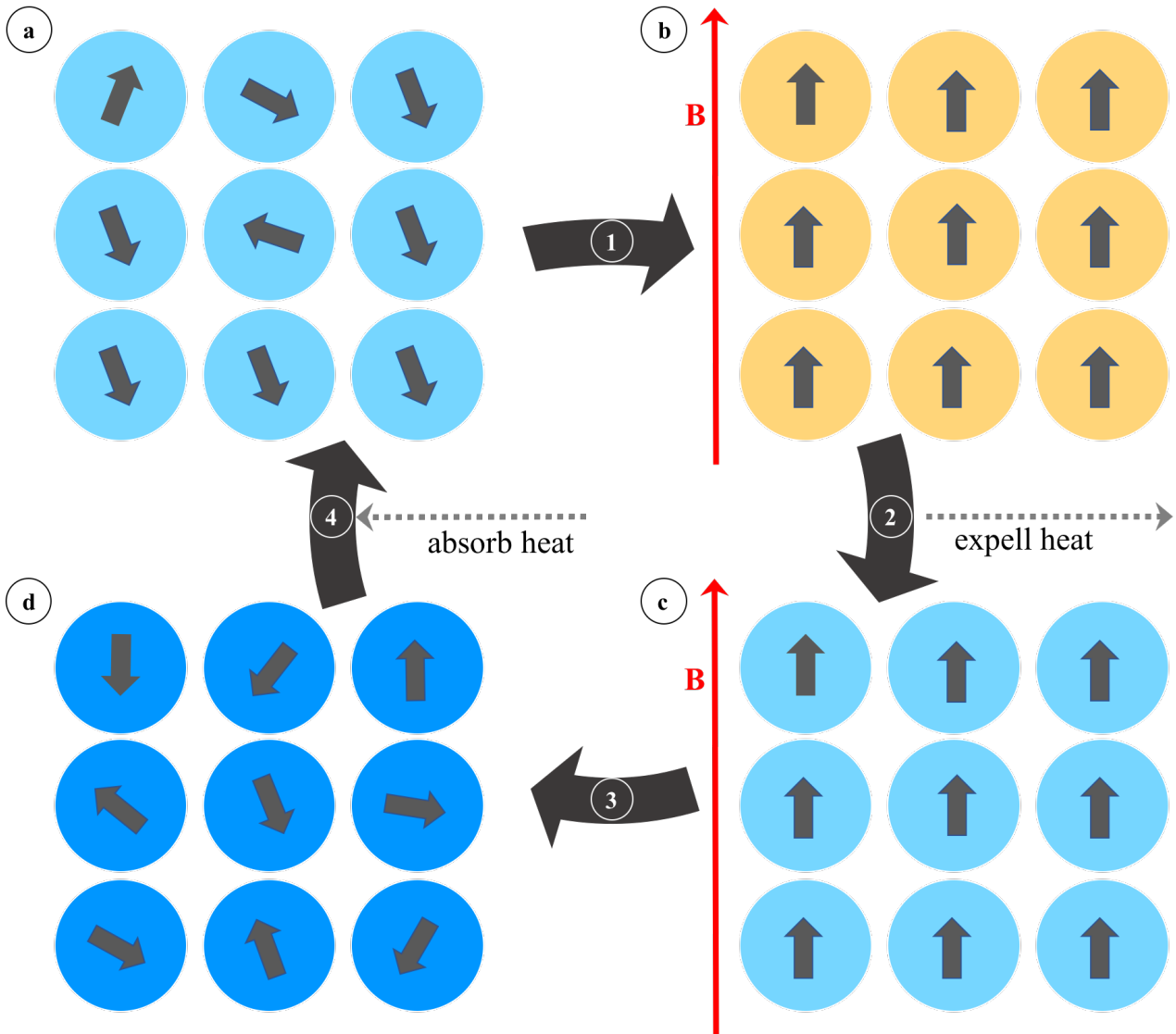
Figure 25. The magnetocaloric cooling cycle consists of four steps: 1) First, the magnetic material (part “a” of the figure) is exposed to a magnetic field, B (represented which a red arrow), resulting in a heating of the material (part “b” of the figure) as consequence of the reduction in the magnetic entropy; 2) The heat excess caused by the alignment of all the spins is expelled to the surroundings, thus yielding to the magnetic material at the same temperature as in the beginning, but with the spins aligned (part “c” of the figure); 3) The removal of the magnetic field causes a cooling of the refrigerant due to the increase of magnetic entropy caused by the spin relaxation (part “d” of the figure); 4) heat can be absorbed from the cooling compartment. The orange colour represents an increase in temperature of the magnetic material, and the dark blue colour represents a decrease in temperature of the magnetic material. The grey arrows represent the large spin of the magnetic material, whose orientation can be modified upon application of a magnetic field (represented as red arrows).
