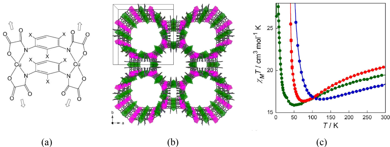
Figure 13. a) Example of an oxamate-based dinuclear metalloligand; b) Crystal structure of [Na(H 2 O) 3.25 ] 4 {Mn 4 [Cu 2 (Me 3 mpba) 2 (H 2 O) 3.33 ] 3 } · 37H 2 O, viewed along the crystallographic c axis showing the pillared square/octagonal layer architecture. Copper and manganese atoms are represented by green and purple octahedra respectively. Free water molecules and Na + counterions have been omitted for clarity; c) Temperature dependence of the product of the direct current (dc) molar magnetic susceptibility by the temperature (χ M T) the activated MOF (green), with methanol molecules filling the pores (red), and with water molecules filling the pores (blue). Reprinted with permission from reference 50, Copyright 2012 American Chemical Society.
