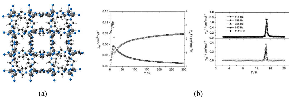
Figure 7. a) Crystal structure of \text{Co}(\text{imidazolate})_2 ; b) Plots of temperature dependence of \chi_M and \chi_{MT} for \text{Co}(\text{imidazolate})_2 measured at 10 kOe field (left) and temperature dependence of AC susceptibility \chi' (top) and \chi'' (bottom) obtained at 20 Oe field. Adapted from reference 36, with permission from Wiley.
