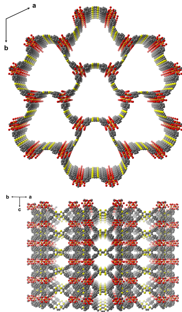
Figure 2. Overview of the crystal structure of MUV-2 showing the hexagonal mesoporous channels along the c -axis (top) and microporous channels orthogonal to the mesoporous ones (bottom). The grey, yellow, red and orange balls represent the C, S, O and Fe atoms, respectively. For simplicity, hydrogens are omitted.
