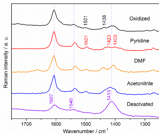
Figure 11. 633 nm Raman spectra of desolvated MUV-2 (purple line), and solvated with acetonitrile (blue line), DMF (orange line), and pyridine (red line), and electrochemically oxidized ox-MUV-2 (black line) at 298 K in solid state. See Figure S29 for a larger spectral range.
