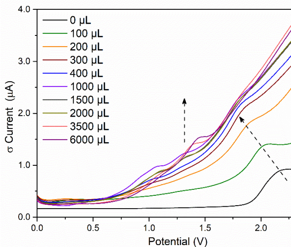
Figure 10. Differential Pulse Voltammetry (DPV) of MUV-2 in \text{CH}_3\text{CN} after consecutive addition of aliquots of pyridine using \text{TBAPF}_6 0.1 M as electrolyte. Platinum wire was used as the counter electrode and silver wire as the pseudoreference electrode.
