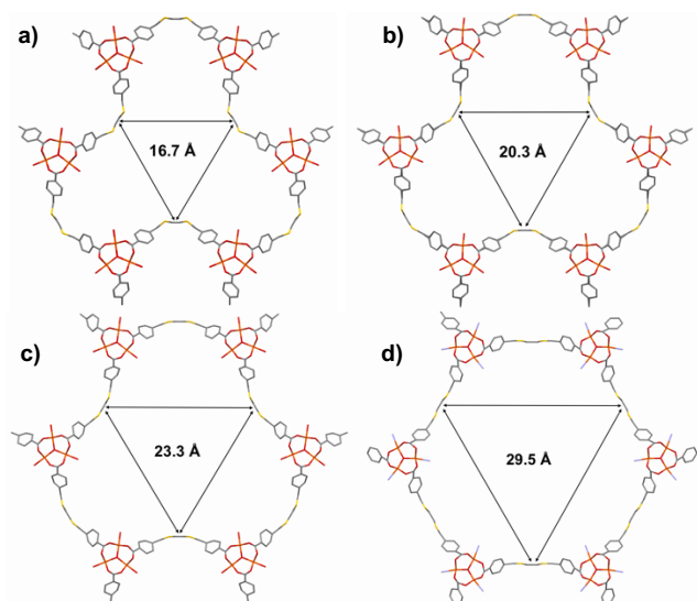
Figure 3. Crystal view of the pore opening evolution of a) MUV-2(29) ( a = b = 29.4 Å; c = 12.5 Å), b) MUV-2(31) ( a = b = 31.9 ; c = 12.5 Å), c) MUV-2(33) ( a = b = 33.3 ; c = 12.4 Å), and d) MUV-2(35) ( a = b = 35.4 Å; c = 12.1 Å) forms. The grey, yellow, red, orange and blue ellipsoids represent the C, S, O, Fe and N atoms, respectively. For simplicity, hydrogens are omitted.
