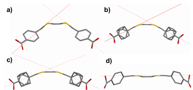
Figure 4. Partial views of the TTFTB ligand for the crystal structures of a) MUV-2(29) ; b) MUV-2(31) ; c) MUV-2(33) and d) MUV-2(35) highlighting the dihedral angles between the planes formed by the two dithiole rings ( \theta = 69^\circ , 54^\circ , 41^\circ and 9^\circ , respectively).
