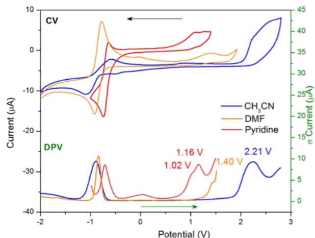
Figure 9. Solid-state Cyclic Voltammetry (CV) and Differential Pulse Voltammetry (DPV) of MUV-2 in \text{CH}_3\text{CN} (blue line), DMF (orange line) and pyridine (red line) using \text{TBAPF}_6 0.1 M as electrolyte and 0.1 V/s scan rate. Platinum wire was used as the counter electrode and silver wire as the pseudoreference electrode. Ferrocene was added as internal standard. All potentials are reported versus \text{Ag}/\text{AgCl} .
