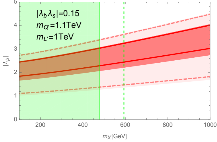
Figure 5: Required values for \lambda_L^\mu (denoted as \lambda_\mu in this figure) and m_X to explain the observed values of R_K and R_{K^*} in the model of [13]. This figure has been obtained with fixed |\lambda_Q^b \lambda_Q^s| = 0.15 , m_L = 1 TeV and m_Q = 1.1 TeV. The light (dark) red region corresponds to the R_K measurement at 1\sigma ( 2\sigma ), whereas the red lines indicate the same regions for R_{K^*} . The green region is excluded due to B_s - \overline{B}_s mixing for m_Q = 1.1 TeV. The excluded region would extend up to the dashed green line for m_Q = 1 TeV. Figure taken from [13].
