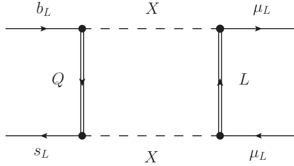
Figure 4: Generation of \mathcal{O}_9 and \mathcal{O}_{10} in the model of [13]. Semileptonic four-fermion operators are generated at the 1-loop level.
