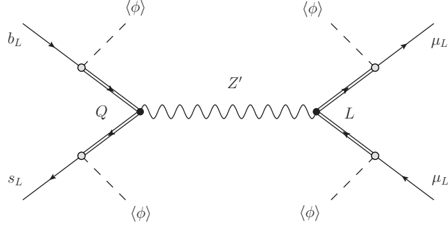
Figure 1: Generation of \mathcal{O}_9 and \mathcal{O}_{10} in the model of [2]. The mixing between the SM fermions and the vector-like ones induce semileptonic four-fermion interactions.
