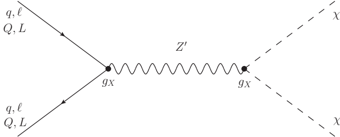
Figure 2: DM production via the Z' portal in the model of [2]. We notice that the vertex on the left of the diagram also participates in the explanation of the b \rightarrow s anomalies (see Fig.1).
