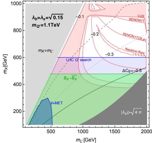
Figure 6: Contours of constant C_9^{\mu, \text{NP}} in the m_L - m_X plane for the model of [13]. This figure has been obtained with fixed \lambda_Q^b = \lambda_Q^s = \sqrt{0.15} and m_Q = 1.1 TeV, choosing \lambda_L^\mu in order to reproduce the observed DM relic density. The colored regions are excluded by various constraints: heavy quark and lepton searches at the LHC (blue), B_s - \bar{B}_s mixing (green) and direct DM detection experiments (red). The grey regions are excluded due to perturbativity constraints (dark grey region) or by demanding that X is the lightest U(1)_X -charged state (light grey region). Future direct DM detection prospects are also shown in this plot. Figure taken from [13].
