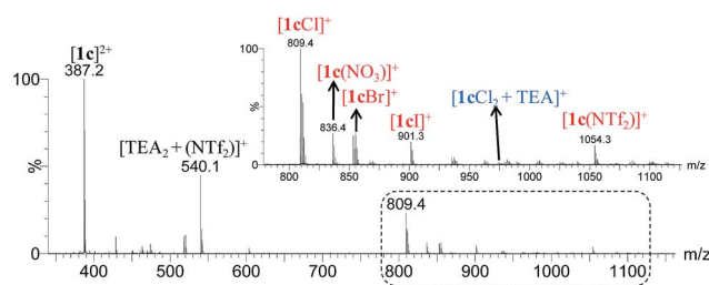
Fig. 4 Competitive ESI mass spectrum of an equimolar mixture of [ 1c ](NTf 2 ) 2 and TEAX (X = \text{Cl}^- , \text{Br}^- , \text{I}^- and \text{NO}_3^- ) in MeCN. The inset shows the expanded region in the m/z 750–1150 range illustrating the ion abundances of the species [ 1c X] + .
