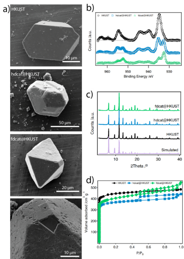
Figure 4: Effect of the catechol coating on the properties of HKUST. (a) SEM images of HKUST, hdcat@HKUST and fdcat@HKUST crystals. (b) Cu 2p high-resolution XPS spectra, (c) PXRD patterns compared to the simulated PXRD of HKUST and (d) N 2 isotherms at 77 K of the solids before and after the coating process. This figure has been adapted with permission from ref. 19. Please click here to view a larger version of this figure.
