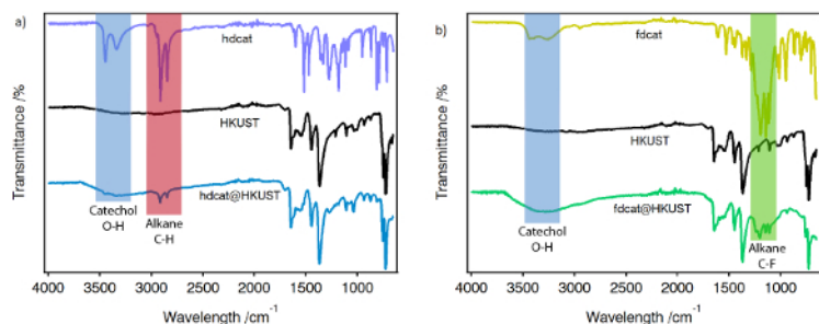
Figure 3: Chemical characterization of hdcats@HKUST and fdcats@HKUST. Fourier-transformed infrared (FT-IR) spectra of hdcats@HKUST with HKUST and hdcats (a), and fdcats@HKUST with HKUST and fdcats (b). This figure has been adapted with permission from ref. 19. Please click here to view a larger version of this figure.
