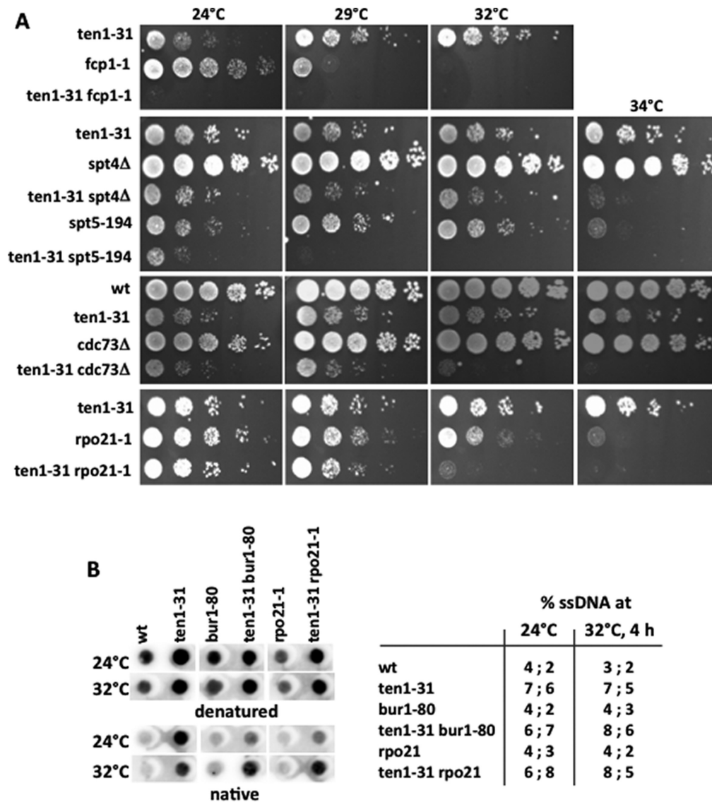
Figure 2. Genetic and functional interactions of ten1-31 with transcription regulators mutants. (A) TEN1 genetically interacts with SPT4 and SPT5 , as well as with FCP1 , RPB1 and CDC73 , as strong synthetic interactions between the corresponding mutations were observed. ten1-31 , spt5-194 , fcp1-1 and rpo21-1 (a mutation in RPB1 ) are temperature-sensitive mutations in essential genes, while spt4Δ and cdc73Δ are null mutations. (B) Measurements by dot blot of increased amounts of telomeric ssDNA reflecting the accumulation of telomeric DNA damage (5). Left panel: Hybridisation of genomic DNA from the indicated mutant and wild-type (wt) strains to a TG 1-3 32 P-labelled probe under native conditions revealed the presence of abnormally high levels of telomeric ssDNA either at 24°C or 32°C, a restrictive temperature of growth for the ten1-31 , bur1-80 and rpo21-1 mutations. Right panel: Quantification of the radioactive signals of telomeric ssDNA was performed by comparing the signal of the native dots to the corresponding signals on the denatured dots (eight times more genomic DNA was loaded on the native blots) and expressed as the percentage (% ssDNA) of signal of the denatured blot. For each temperature, numbers in the left column correspond to the signals from the blots illustrated in the left panel, while numbers in the right column represent the signals obtained in a second experiment (blots not shown). Similar results from a third experiment conducted by Southern blotting allowed us to conclude to an absence of increased telomeric ssDNA signals in the two double mutants compared with the single mutants (not shown).
