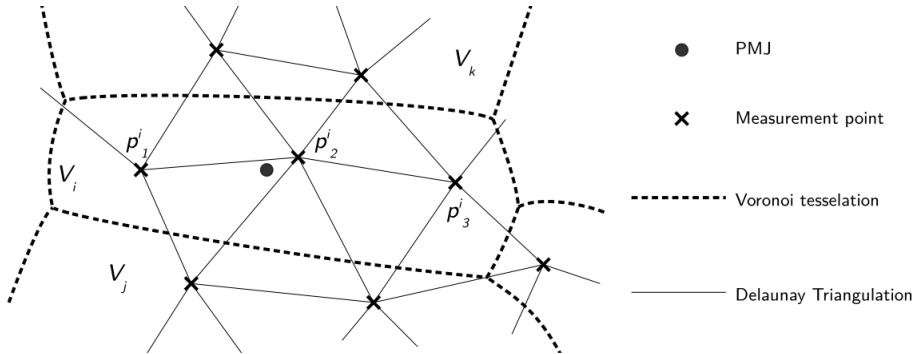
Figure 3.3: A situation with a Voronoi region, V_i , containing three measurement points, \mathbf{p}_1^i , \mathbf{p}_2^i and \mathbf{p}_3^i , which do not form a triangle of the Delaunay triangulation.
