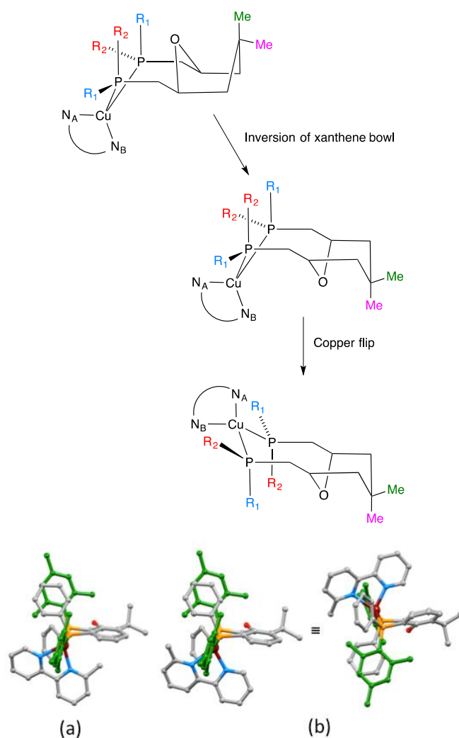
Fig. 5 Upper: Proposed dynamic processes in [\text{Cu}(\text{xantphos})(\text{bpy})]^+ type compounds. N A and N B represent pyridine rings A and B. For ^t\text{Bu}_2\text{xantphos} , R 1 = R 2 = Ph. For \text{xantphosMes}_2 , R 1 = Mes, R 2 = Ph. Lower: Crystallographically determined structure of the [\text{Cu}(\text{xantphosMes}_2)(6\text{-Meppy})]^+ cation in which the 6-Meppy is orientationally disordered: (a) orientation 1 of 6-Meppy, and (b) orientation 2 of 6-Meppy shown in two views of the cation (see text).
