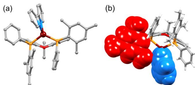
Fig. 3 Structure of the [Cu(xantphosMes 2 )(bpy)] + cation (a) emphasizing the relative positions of the phenyl and mesityl substituents with respect to the bpy unit, and (b) with the bpy (blue) and one mesityl group (red) shown in space-filling representation to emphasize their spatial proximity.
