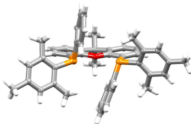
Fig. 1. Crystallographically determined structure of the ( S,S )-enantiomer of xantphosMes 2 . See also Fig. S3 † .
