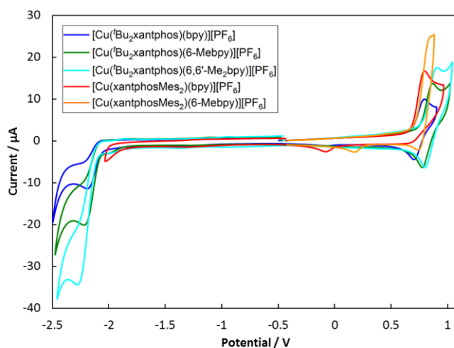
Fig. 9 Cyclic voltammograms of [\text{Cu}(\text{P}^{\wedge}\text{P})(\text{N}^{\wedge}\text{N})][\text{PF}_6] compounds in \text{CH}_2\text{Cl}_2 at a scan rate of 100 \text{mV s}^{-1} referenced to internal \text{Fc}/\text{Fc}^+ = 0 V.
