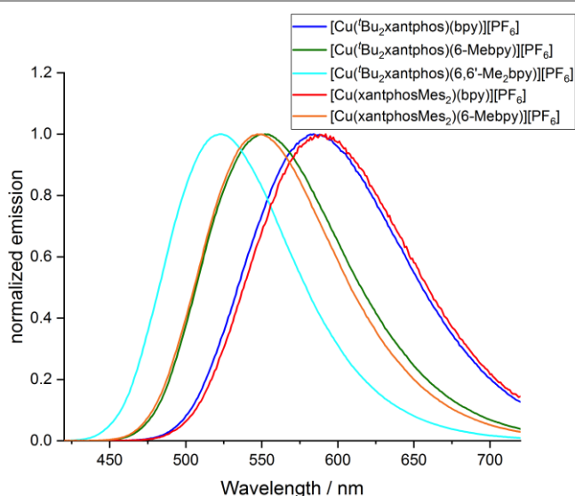
Fig. 12 Normalized solid-state emission spectra of [\text{Cu}(\text{P}^{\wedge}\text{P})(\text{N}^{\wedge}\text{N})][\text{PF}_6] complexes ( \lambda_{\text{exc}} = 365 nm).
