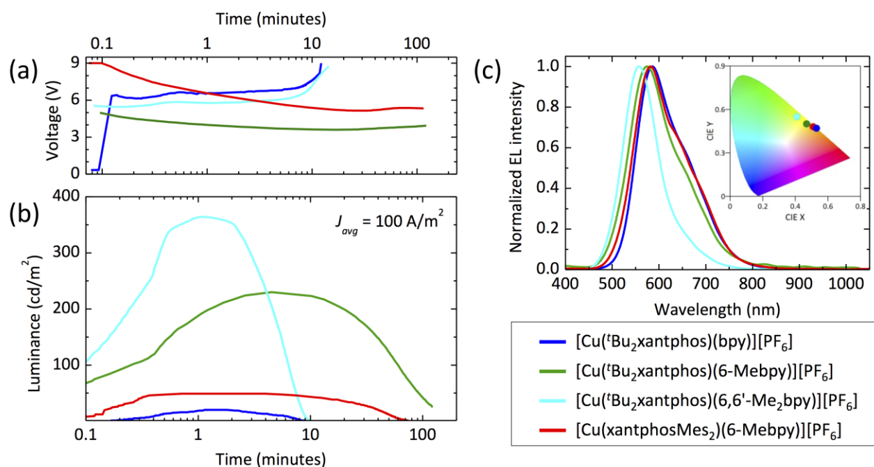
Fig. 14 Time evolution of the (a) voltage and (b) the luminance for a series of LECs driven at an average current density of 100 \text{ A/m}^2 . (c) Electroluminescence spectra for the same device series with (inset) the corresponding colour coordinates in the CIE 1931 colour space.
