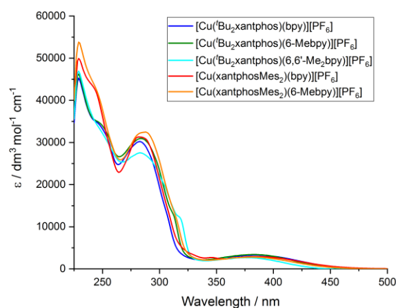
Fig. 11 Solution absorption spectra of Cu(P ^A P)(N ^A N)[PF 6 ] complexes (CH 2 Cl 2 , 2.5 \times 10^{-5} mol dm -3 ).
