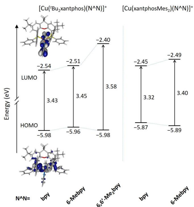
Fig. 10 Energy diagram showing the energies calculated for the HOMO and LUMO of [Cu( t Bu 2 xantphos)(N ^A N)] + and [Cu(xantphosMes 2 )(N ^A N)] + complexes. The HOMO-LUMO energy gap is also quoted. Isovalue contour plots ( \pm 0.03 a.u.) are shown for the HOMO and LUMO of [Cu( t Bu 2 xantphos)(bpy)] + .
