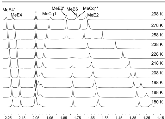
Fig. 8 Alkyl regions of the variable temperature ^1\text{H} NMR spectra (500 MHz, acetone- d_6 ) of [\text{Cu}(\text{}^t\text{Bu}_2\text{xantphos})(6\text{-Mebpy})][\text{PF}_6] . See Scheme 3 for atom labelling.
