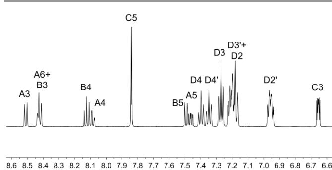
Fig. 6 Aromatic region of the ^1\text{H} NMR spectrum (500 MHz, acetone- d_6 ) of [\text{Cu}(\text{tBu}_2\text{xantphos})(6\text{-Mebpy})][\text{PF}_6] . See Scheme 3 for atom labelling.
