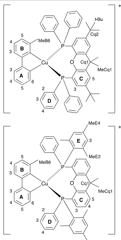
Scheme 3 Structures of [\text{Cu}(\text{tBu}_2\text{xantphos})(6\text{-Mebpy})]^+ and [\text{Cu}(\text{xantphosMes}_2)(6\text{-Mebpy})]^+ with labelling for NMR spectroscopic assignments.
