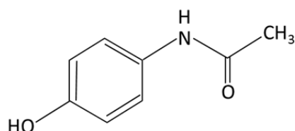
Figure 1: Paracetamol (Acetaminophen) molecule.
