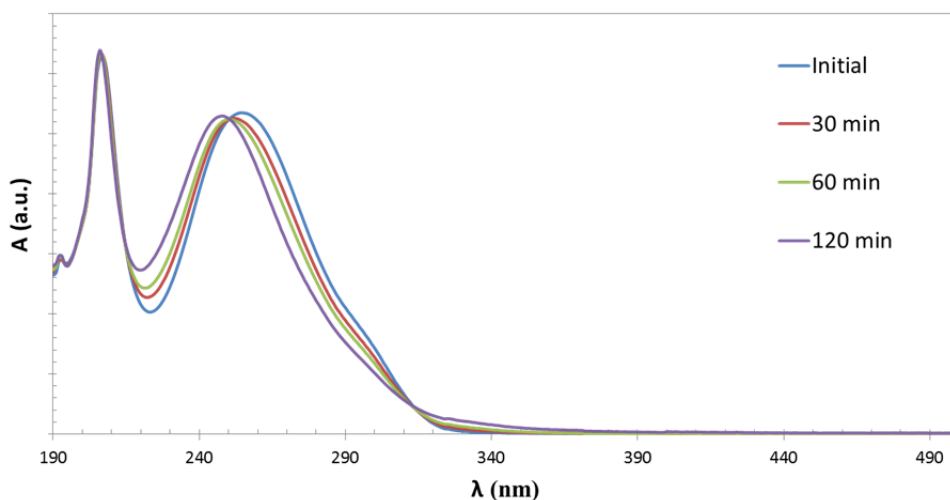
Figure 6: Evolution of UV-Vis spectra of paracetamol solution with time while degradation with iron oxide nanostructure at pH 11.
