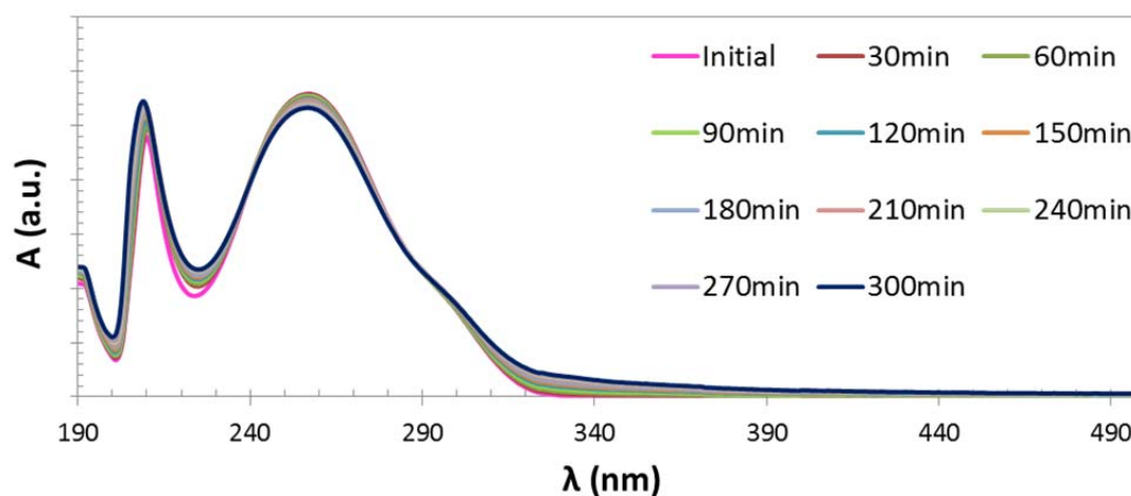
Figure 7: Evolution of UV-Vis spectra of paracetamol solution with time while degradation with iron oxide nanostructure at pH 12.
