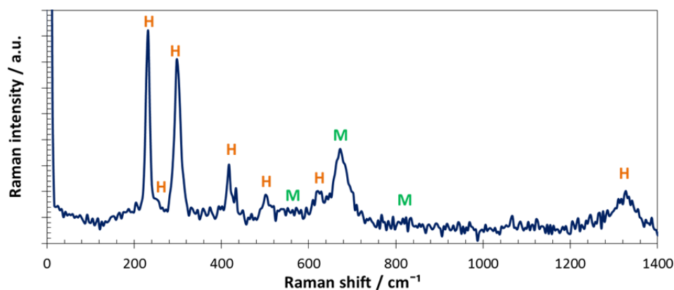
Figure 3: Raman spectra of the iron oxide nanostructures used for the degradation of paracetamol.
