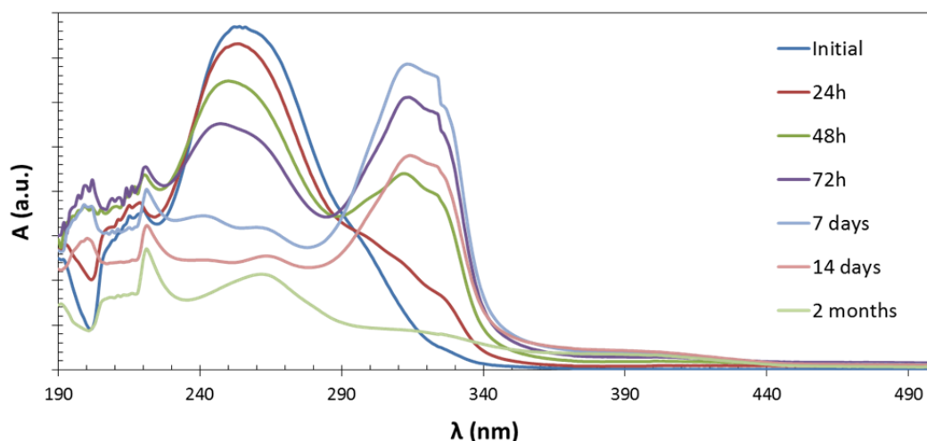
Figure 4: Evolution of UV-Vis spectra of 1 M NaOH solution with paracetamol with time.
