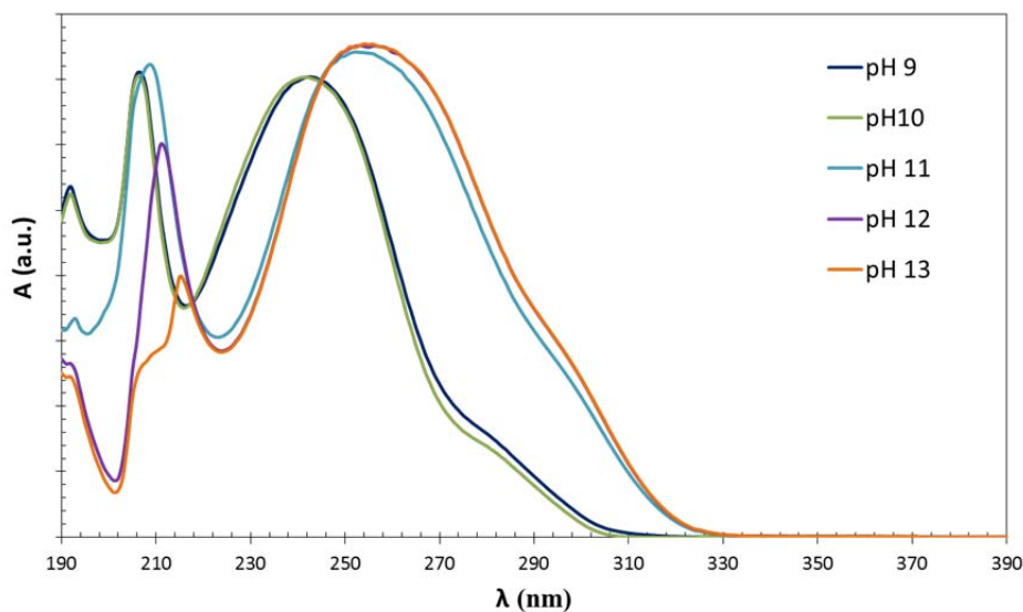
Figure 5: Evolution of UV-Vis spectra of paracetamol solution at different pH.
