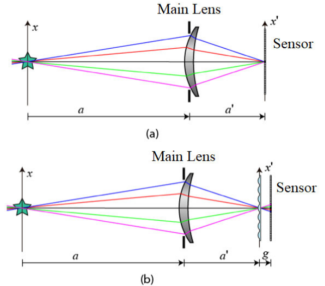
FIGURE 2. a) summation of the rays falling onto a pixel of a conventional 2D camera b) Capturing of individual rays by LF camera.
