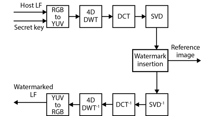
FIGURE 7. The embedding procedure.
