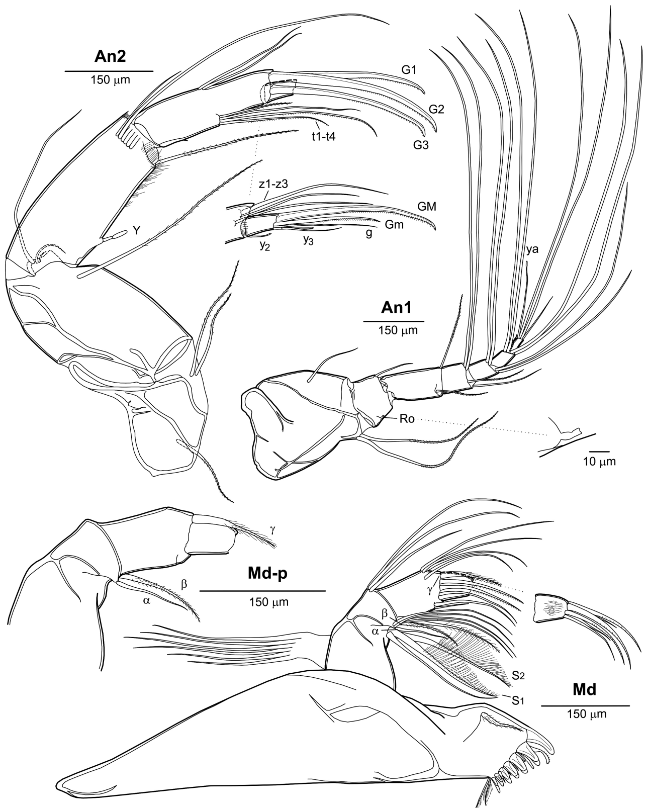
FIGURE 6. Details of the antennula (An1), antenna (An2), and mandibula (Md) of C. pretusi sp. nov. All drawings from individual MUVHNZY0005, except branchial plate of Md and Ro (MUVHNZY0006).
