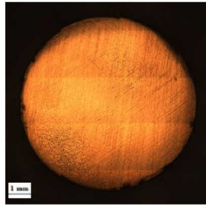
b. Final conditions (sample diameter = 8 mm)
