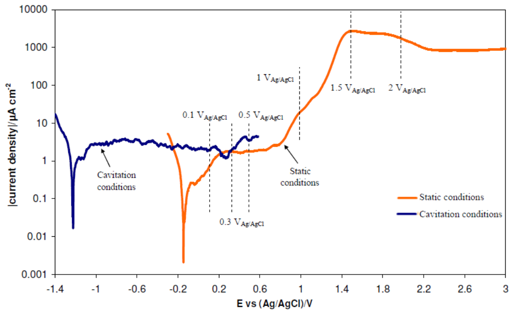
Fig. 3. Potentiodynamic polarisation curves for titanium in 992 g/l LiBr solution under static and cavitation conditions. This figure also shows potentials chosen to perform the potentiostatic tests (on the curve under static conditions).
