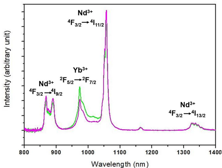
Figure S6.2. Emission spectra of \text{Nd}_{0.943}\text{Yb}_{0.057}(\text{BTC})_3(\text{H}_2\text{O})_6 (magenta line) and \text{Nd}_{0.856}\text{Yb}_{0.144}(\text{BTC})_3(\text{H}_2\text{O})_6 (green line) excited at 580 nm.
