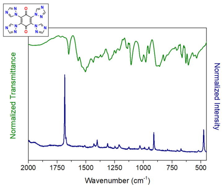
Figure 1.1. Raman spectrum (blue) in 2000-400 \text{cm}^{-1} range and FT-IR spectrum (green) in 1800-400 \text{cm}^{-1} range of 1 (without purification).
