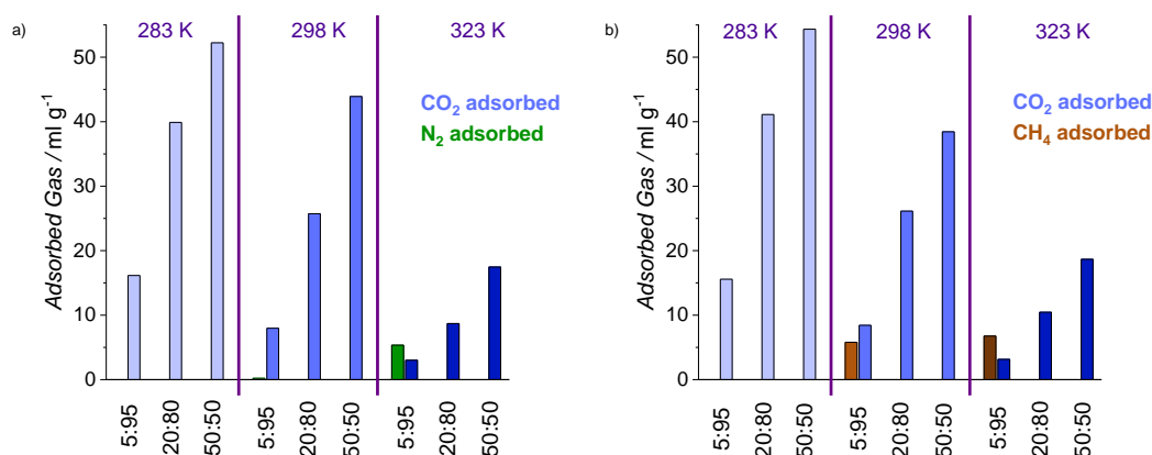
Figure 3.9. Gas adsorbed amounts on 1 , calculated from breakthrough profiles, at 1 bar (absolute pressure) for: a) \text{CO}_2:\text{N}_2 , and b) \text{CO}_2:\text{CH}_4 mixtures; at different concentrations (5 %, 20 % and 50 %) and different temperatures (283 K, 298 K and 323 K). Time zero is set with the first detection of helium (tracer).
