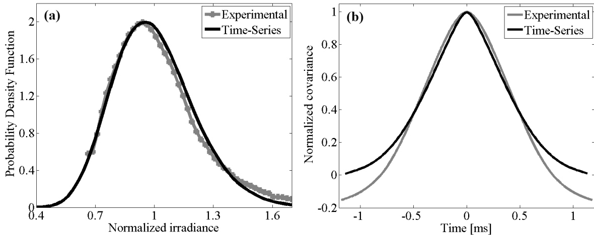
FIG. 5: Comparison between the measured data and predicted time-series for (a) PDF, and (b) the normalized temporal covariance for the case 3.
