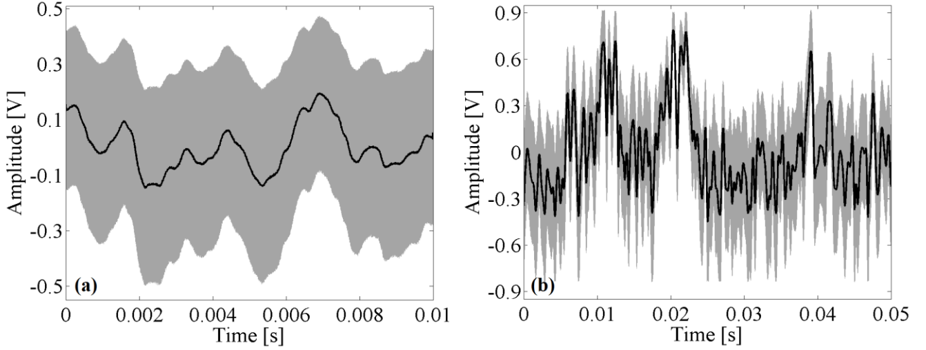
FIG. 3: Sampled signal received by the photodetector (grey line) and the point-by-point average signal value (black line) in case 7 (a), and in case 2 (b).
