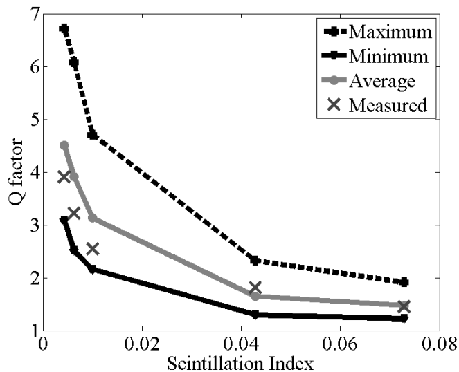
FIG. 7: Q factor versus scintillation index for the measured and the simulated maximum, mean, minimum values.
