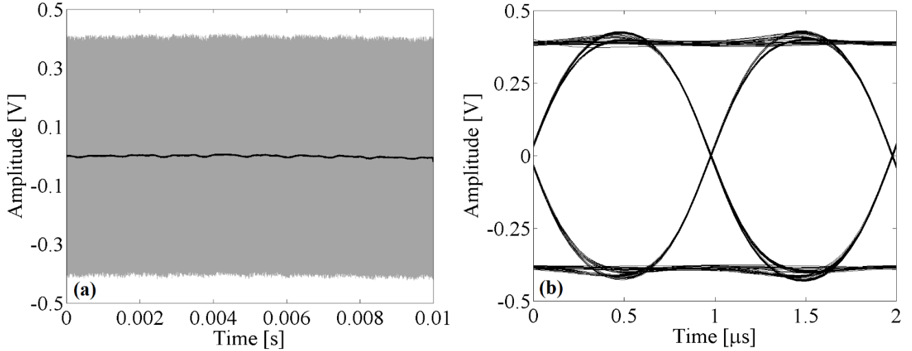
FIG. 2: (a) Sampled signal received at the photodetector (grey line) and the point-by-point average signal value (black line) for case 3, and (b) the corresponding eye-diagram (plotted considering the first 4000 samples).
