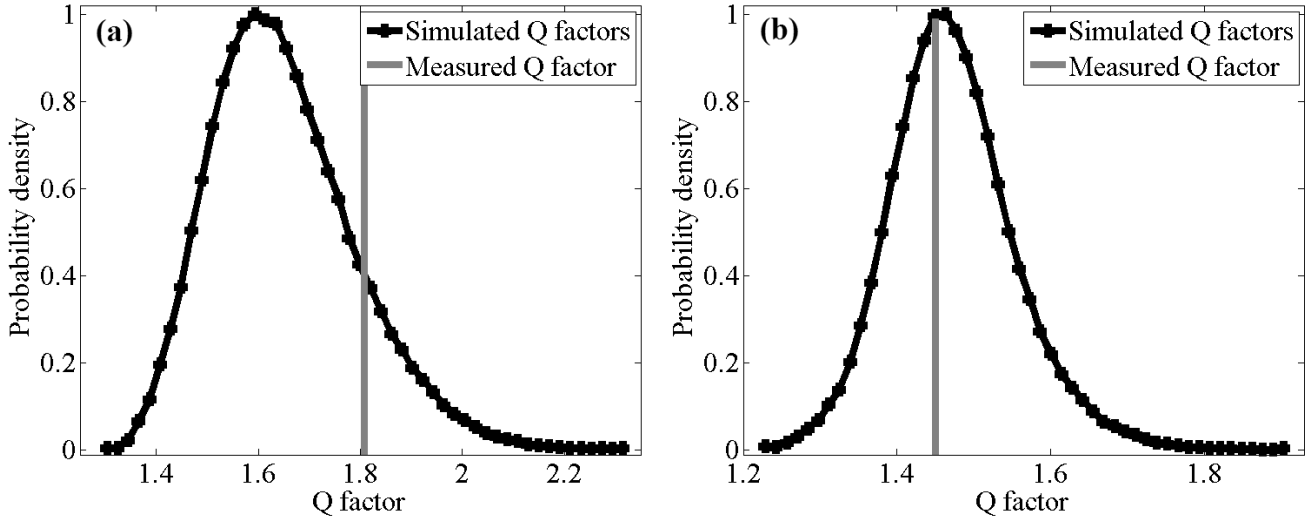
FIG. 6: Simulated and measured probability density against the Q -factor values for: (a) case 3, and (b) case 8.
