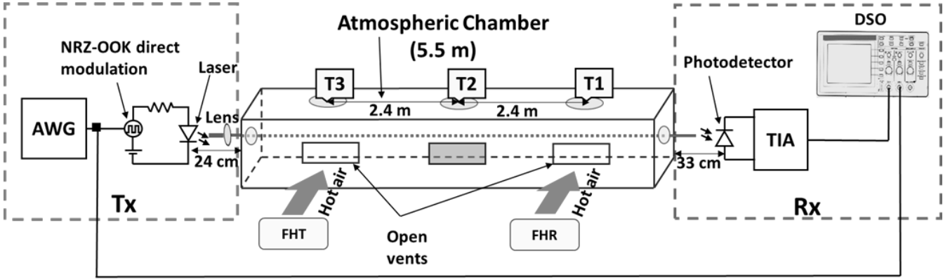
FIG. 1: Schematic block diagram of the experimental set-up
