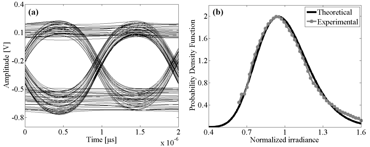
FIG. 4: Case 2 – (a) The eye diagram, and (b) PDF plots for measured samples and predicted using Gamma-Gamma distribution.
