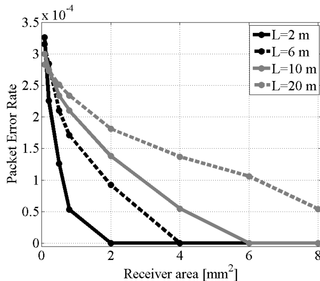
FIG. 8: Packet Error Rate versus receiver active area, at different path lengths and at Rytov variance = 0.096
