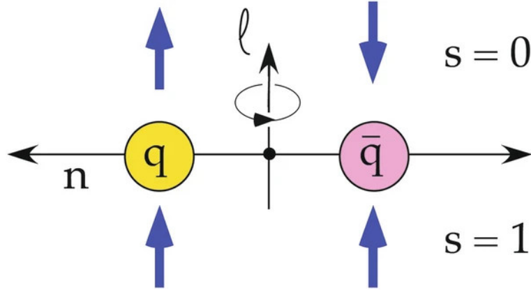
FIGURE 1.2: A q\bar{q} meson pair may be in a spin-singlet state ( s=0 , antiparallel quark spins) or in a spin-triplet state ( s=1 , parallel quark spins). Excited states are obtained by switching angular momentum \ell > 0 within the q\bar{q} pair (orbital excitations) or by inducing vibrations n > 1 (radial excitation). Image taken from Ref. [7].
