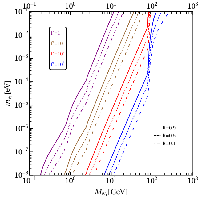
FIGURE 6.3: m_{\nu_1}-M_{N_1} lines corresponding to a specific value of R_{\ell\ell} and f' . For each color, the three lines correspond to values of R_{\ell\ell} = 0.9, 0.5 and 0.1 from left to right.
