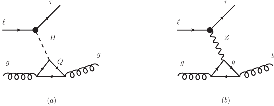
FIGURE 3.8: Higgs and Z contribution to \ell g \rightarrow \tau g , with \ell = e, \mu . The dot indicates the CLFV vertex. Q is a heavy quark, namely Q = c, b, t , and q = u, d, c, s, t, b .
