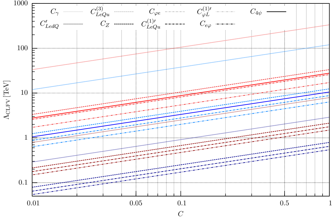
FIGURE 3.9: Constraints on \Lambda_{\text{CLFV}} with respect to the values of WCs, based on the current Belle (shades of blue) and expected Belle II (shades of red) limits, given at the 99.8% confidence level. The four-fermion WCs are represented altogether as C_{4\psi} . For a given set of limits (distinguished by blue and red color shades), the lighter shades correspond to the WCs listed in the first row of the key (omitting now for a moment the common four-fermion WC C_{4\psi} ) and the darker shades correspond to the WCs listed in the second row. To make the use of the plot even simpler, for a given set of bounds (red or blue lines), the WCs (again up to C_{4\psi} ) are listed in the key in the same order as they appear in the plot, the light-shaded lines being always above the dark-shaded ones. Similarly, for a given WC, the red line appears always above the blue line, corresponding to stronger limits expected from Belle II.
