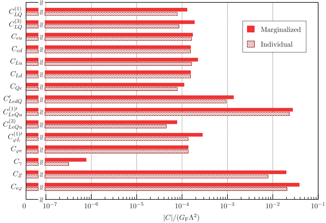
FIGURE 3.12: Allowed values for C/(G_F\Lambda^2) based on the expected Belle II limits, comparing the individual and marginalized analyses for hadronic tau decays, given at the 99% confidence level.
