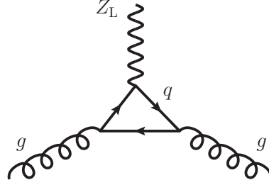
FIGURE D.2: Triangle diagram contributing to Z_L \rightarrow gg . Here, q is a generic quark, q = u, d, c, s, t, b . The final contribution comes from adding to this diagram the analogous one with the quark momenta in the loop reversed.
