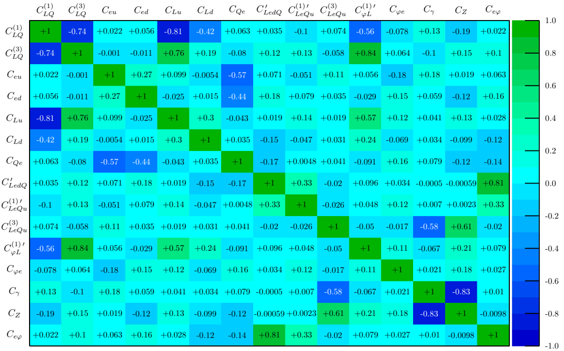
FIGURE H.1: Correlations among all the Wilson coefficients from the numerical analysis considering Belle limits and including FCNCs.
