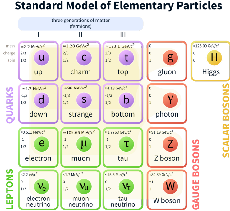
FIGURE 1.1: Diagrammatic illustration of the particle content of the Standard Model.
