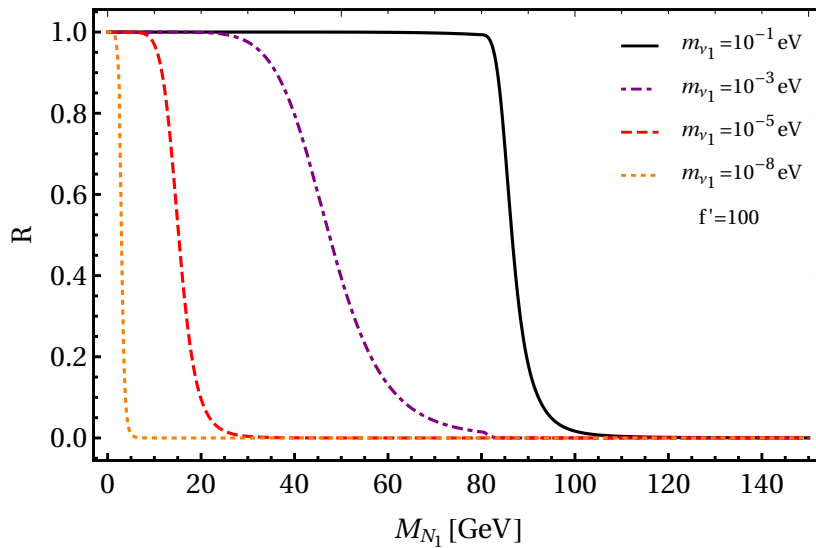
FIGURE 6.2: R_{\ell\ell} vs M_{N_1} for different values of m_{\nu_1} .
