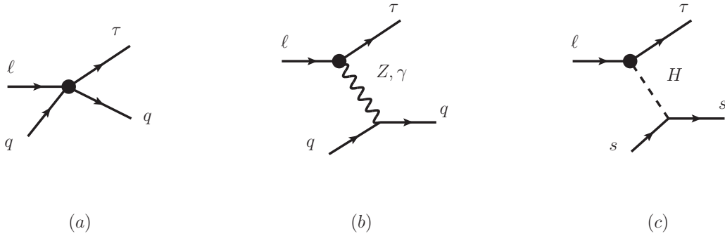
FIGURE 3.7: Different contributions of the SMEFT Lagrangian to \ell q \rightarrow \tau q for \ell = e, \mu and q = u, d, s . The dot indicates the CLFV vertex. We consider m_u = m_d = 0 but m_s \neq 0 . Hence, the contribution of the Higgs in (c) only exists for q = s .
