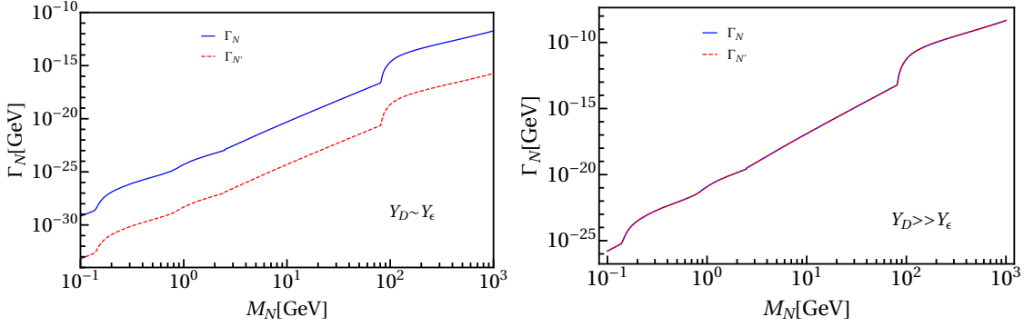
FIGURE 6.1: \Gamma_{N^{(\prime)}} vs M_{N^{(\prime)}} . Left and right panels correspond to the cases where Y_\epsilon \sim Y_D and Y_\epsilon \ll Y_D respectively. Both are shown within Scenario b for g = 1 (left) and g = 10^2 (right), see Section 6.5 for more details.
