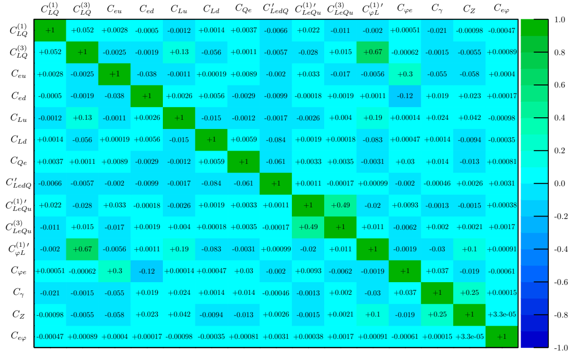
FIGURE H.3: Correlations among all the Wilson coefficients from the numerical analysis considering \ell - \tau limits and including FCNCs.
