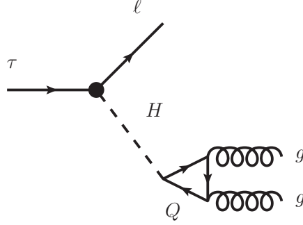
FIGURE 3.6: Dominant scalar contribution [155] to \tau \rightarrow \ell \bar{P} P , with \ell = e, \mu and P = \pi, K . The dot indicates the CLFV vertex. The Q in the loop stands for a heavy quark, namely Q = c, b, t .
