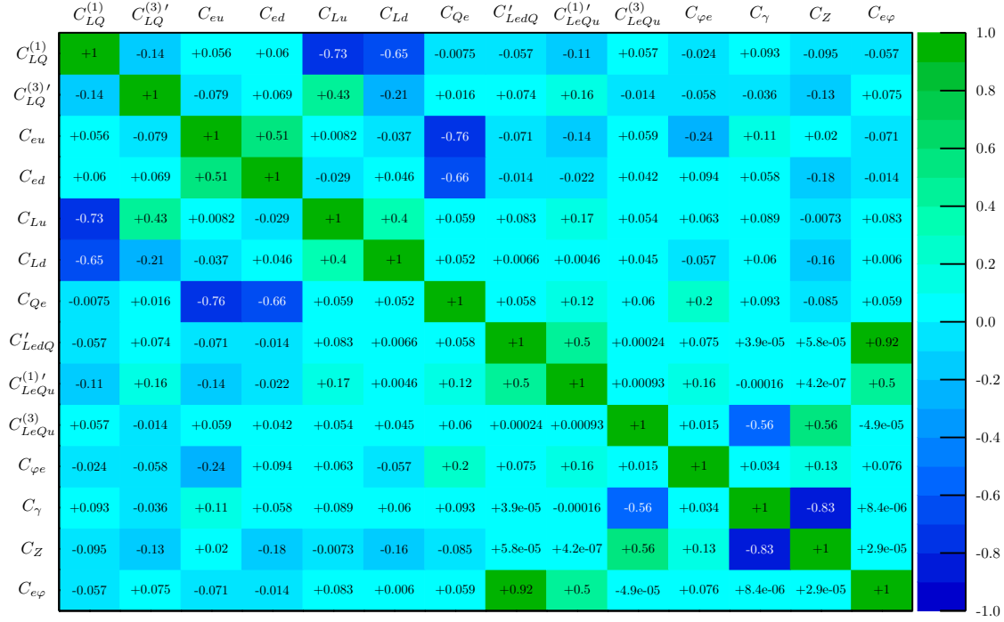
FIGURE H.2: Correlations among all the Wilson coefficients from the numerical analysis considering Belle limits and excluding FCNCs.
