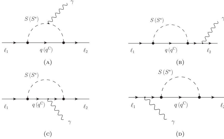
FIGURE 4.1: Feynman diagrams of the leading-order contribution to the \ell_1 \rightarrow \ell_2 \gamma process from scalar leptoquarks.
