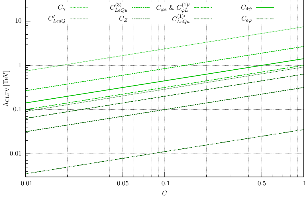
FIGURE 3.13: Constraints on \Lambda_{\text{CLFV}} with respect to the values of WCs from \mu\text{-}\tau conversion in Fe(56,26), based on the expected sensitivity of the NA64 experiment, given at the 99.8% confidence level.
