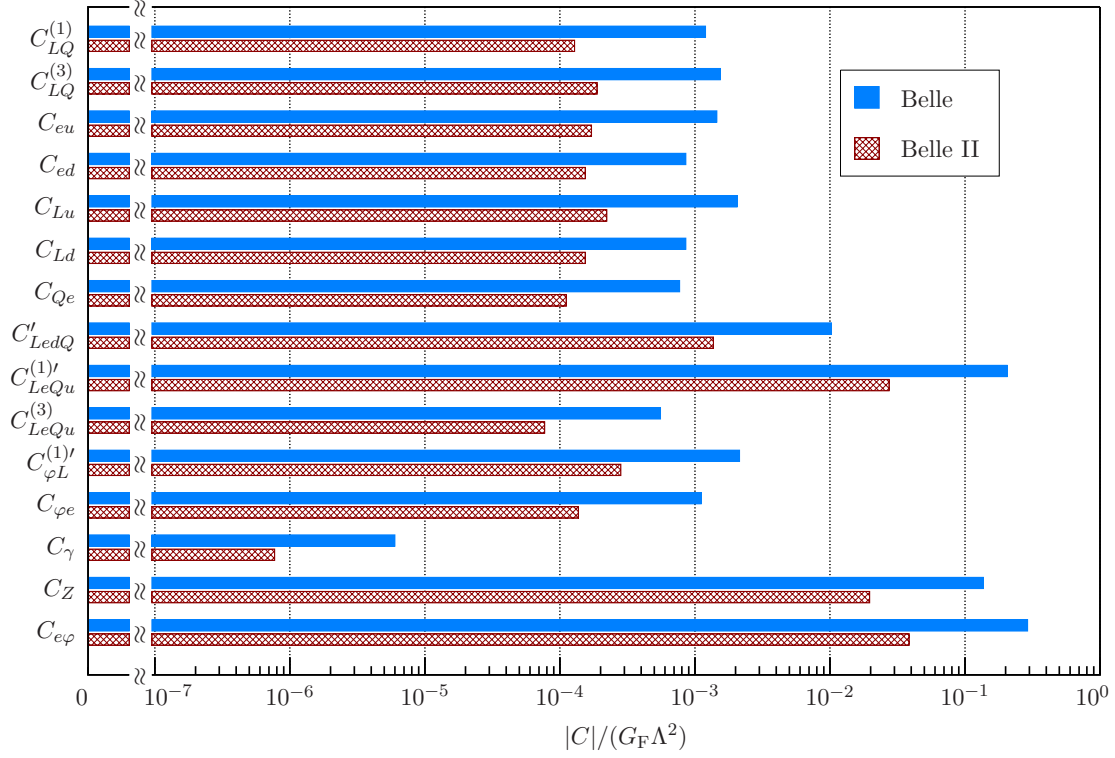
FIGURE 3.11: Allowed values for C/(G_F\Lambda^2) based on the current Belle and expected Belle II limits, stemming from the marginalized analysis for hadronic tau decays, given at the 99% confidence level.
