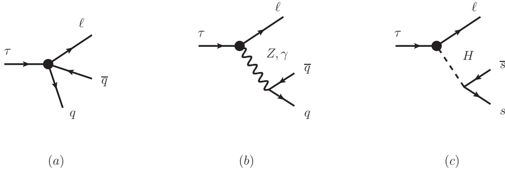
FIGURE 3.5: Different contributions of the SMEFT Lagrangian to \tau \rightarrow \ell \bar{q} q , with \ell = e, \mu . The dot indicates the CLFV vertex. We consider m_u = m_d = 0 , but m_s \neq 0 : the contribution of the Higgs in (c) thus only exists for the production of \bar{s}s .
