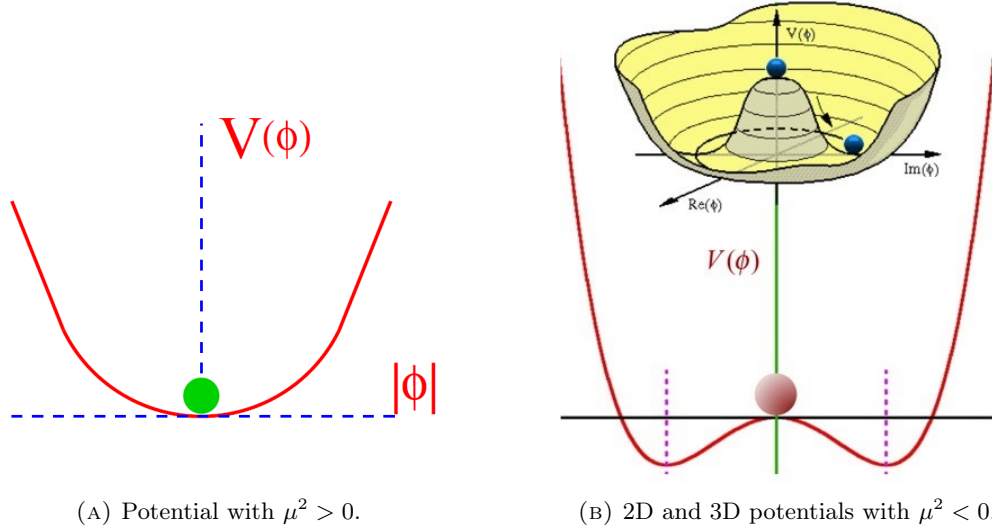
FIGURE 1.3: Different cases of the Higgs potential in terms of \mu^2 .
