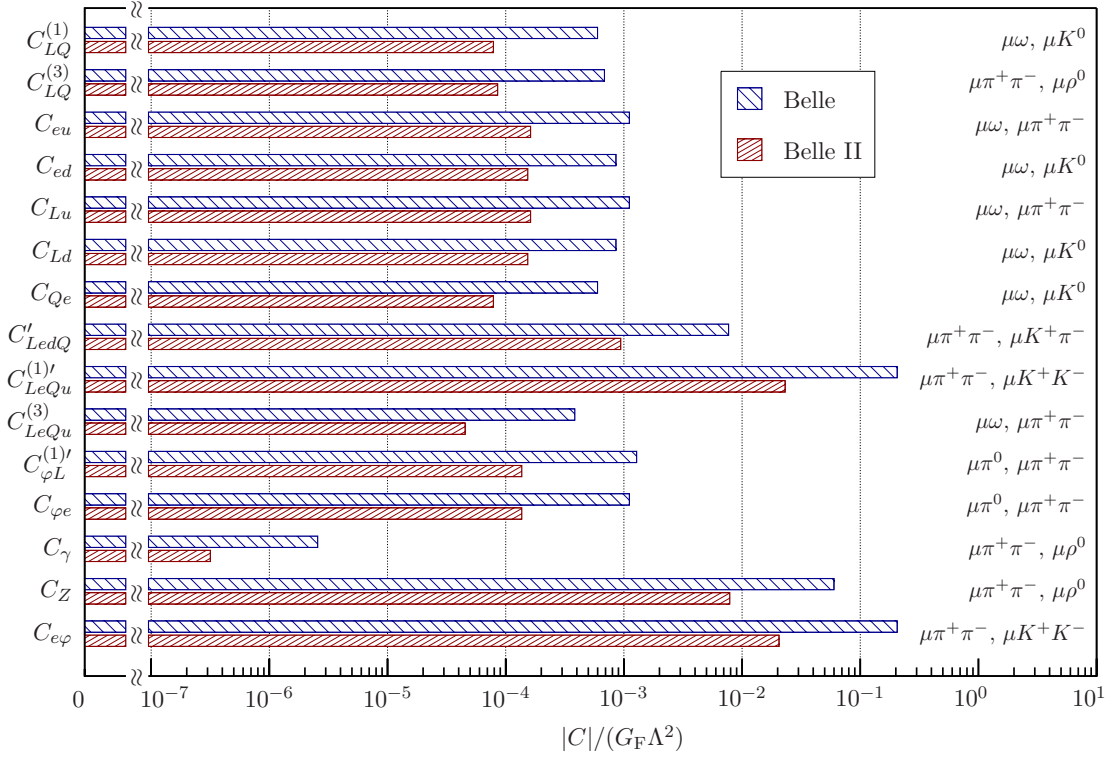
FIGURE 3.10: Allowed values for C/(G_F\Lambda^2) based on the current Belle and expected Belle II limits, stemming from the individual analysis for hadronic tau decays, given at the 99% confidence level. The two most sensitive channels for the given WC are shown.
