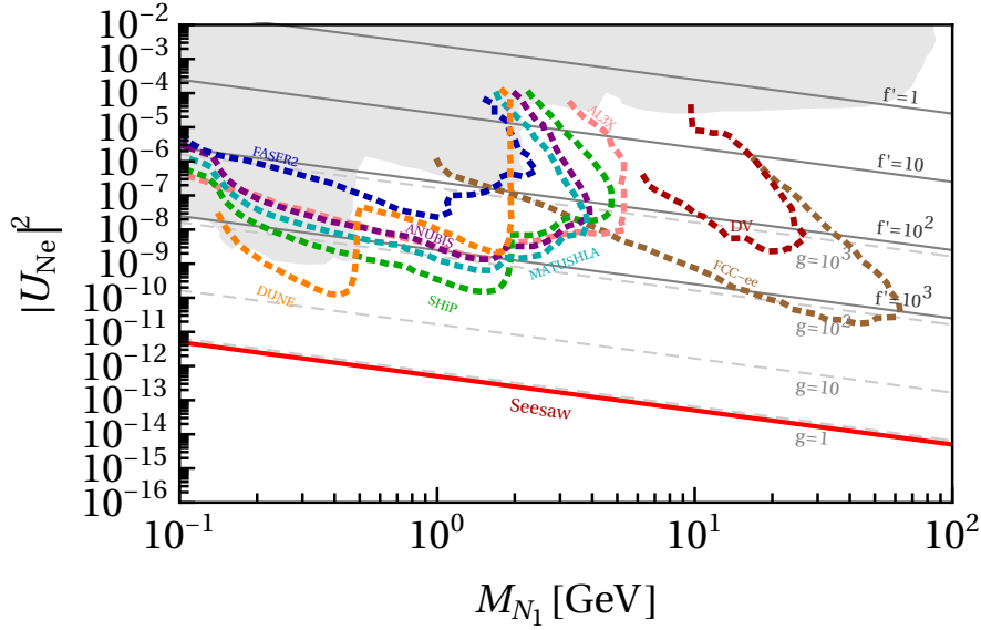
FIGURE 6.4: Active-sterile neutrino mixing |U_{N_1 e}|^2 versus the neutrino mass M_{N_1} , for different values of the parameters f' and g . Dashed lines correspond to the projected sensitivities of future experiments, while the gray shaded area indicates the regions already excluded from current searches as depicted in Ref. [410]. The dashed dark red line limits the zone of the sensitivity of DV searches. The solid red line represents the vanilla seesaw model.
