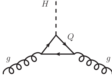
FIGURE D.1: Triangle diagram contributing to H \rightarrow gg . Q indicates a heavy quark, Q = c, b, t . For the final contribution one needs to add an analogous (cross) contribution with the gluons interchanged (or, equivalently, reversed quark momenta in the loop).
