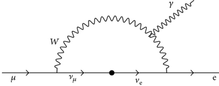
FIGURE 3.4: Diagram of the main contribution to the process \mu \rightarrow e\gamma , within the minimal extension of the SM with a right-handed Dirac neutrino for each family.
