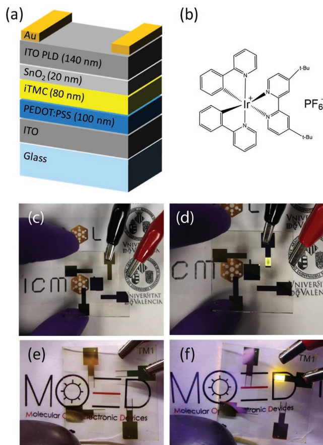
Figure 3. a) Architecture of the semitransparent devices. b) Chemical structure of the yellow Ir(III) emitter [\text{Ir}(\text{ppy})_2(\text{dtb-bpy})][\text{PF}_6^-] used in this work. OFF states of the c) reference and e) semitransparent devices, and ON states of the d) reference and f) semitransparent devices.
