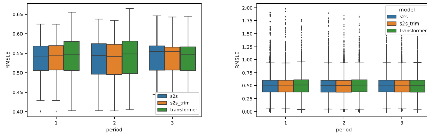
Figure 5.7: Distribution of the error across stores (left) and across items (right) for every model and for the three different test periods used.
