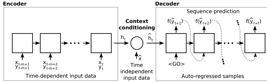
Figure 5.4: Seq2seq architecture diagram. The left box shows the encoder, which takes the historical actual sales y_i as input as well as other exogenous time-dependent features (i.e. oil price, holidays and events, transactions and promotions) denoted by x_i , and returns the hidden vector h_t of the last recurrent module as output (aka context vector ). The middle of the figure shows the context conditioning module, which is the variation proposal over the original sequence-to-sequence proposal. This module receives the context vector h_t from the encoder module and concatenates it with static data \hat{x} producing a conditioned context vector \hat{h}_t = (h_t, \hat{x}) . Finally, on the right, the decoder module receives as initial state the conditioned context vector and provides the first recurrent cell with a go symbol (constant input indicating the input of the decoded sequence). The decoder generates the sequence prediction in an auto-regressive way and f is a stack of two fully-connected layers applied to each output of the decoder.
