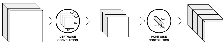
Figure 6.2: Depthwise-separable convolution diagram showing how the whole computation is done in two steps: the depthwise convolution followed by the pointwise convolution .
