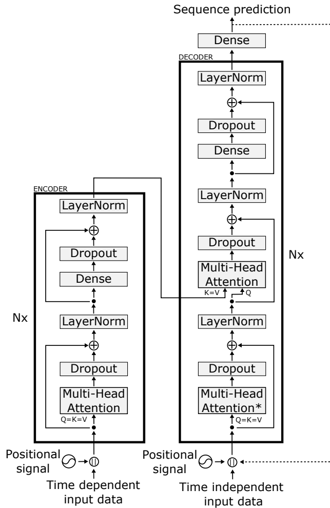
Figure 5.5: Transformer architecture used to perform time series forecasting. In the diagram, the \parallel symbol stands for the concatenation operation, and similarly as in (Vaswani et al., 2017), N_X represents the number of repetitions of the encoder and decoder blocks.
