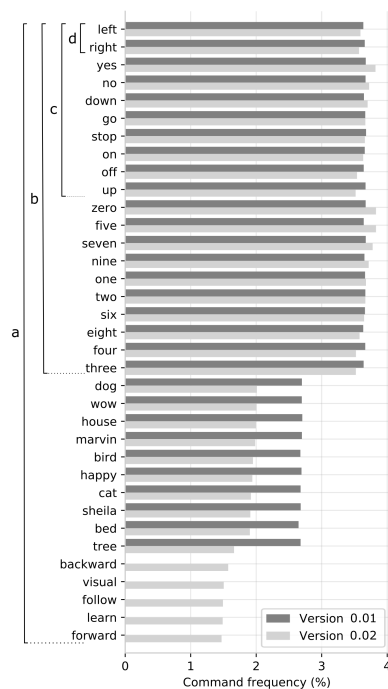
Figure 6.1: Command frequency distribution for both versions of the dataset. The V2 is a refined and extended version of V1. In the left, the four different tasks that have been benchmarked in this work: (a) referred as 35-words-recognition and comprising in both cases all the words for classification, (b) referred as 20-commands-recognition (c) referred as 10-commands-recognition (d) referred as left-right recognition.
