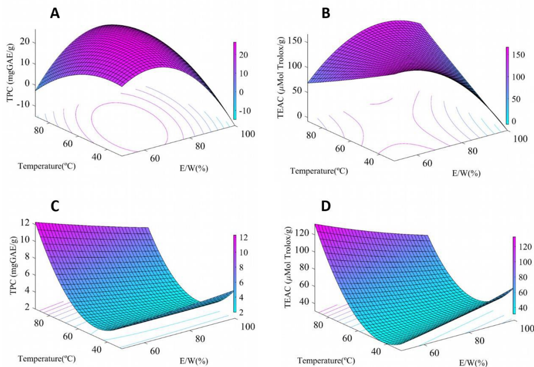
Fig. 1 Response surfaces of the TPC and antioxidant activity of extracts from (a, b) IPE and (c, d) MPE as a function of temperature and E/W with a fixed solid:liquid ratio (12.5 mg/mL).
