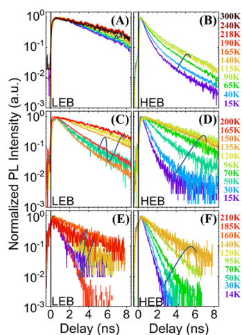
Figure 2. (a–f) Temperature dependence of the time-resolved photoluminescence (PL) emission measured for the three different morphologies: (a, b) one layer of large grains (352 nm-CL), (c, d) multilayers of small grains (550 nm-CS), and (e, f) one layer of islands of small grains (103 nm-IS) at 370 nJ/cm 2 . The blue curves represent the evolution of the emission of the emission by increasing the temperature, which is different in the HEB and LEB.
