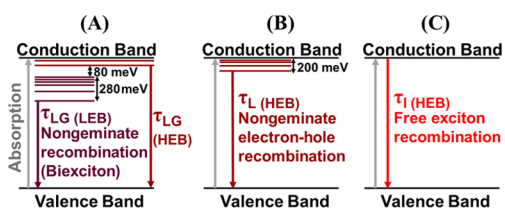
Figure 3. Low-temperature recombination channels in MAPbI 3 for the three morphologies: (a) one layer of large grains (352 nm-CL), (b) multilayers of small grains (550 nm-CS), and (c) one layer of islands of small grains (103 nm-IS). At low temperatures, the grain size of the layer of large grains is responsible for the appearance of the dual emission (see Figure 1 and ref 4). As the island morphology does not exhibit strain inhomogeneities related to the formation of different tetragonal-defective domains, a high excitation fluency of 370 nJ/cm 2 was chosen to fill most of these defective tetragonal-phase sites of the continuous samples (550 nm-CS and 352 nm-CL). This ensures a similar temperature dependence on the lifetime for “O”-excitons for the three morphologies.
